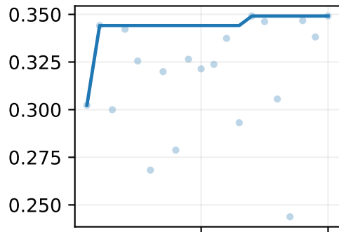
amazon-music · Multi-VAE
