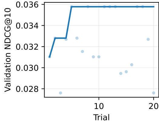
amazon-music · EASE
