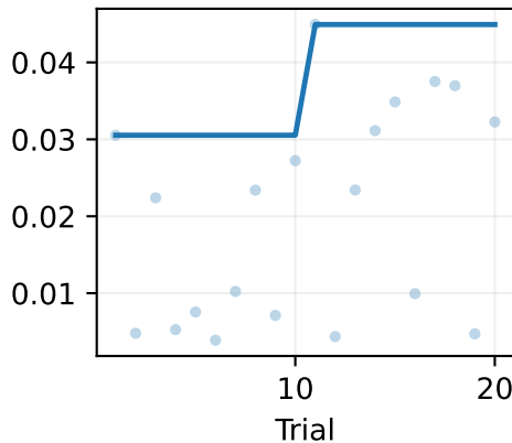
amazon-music · Multi-VAE
