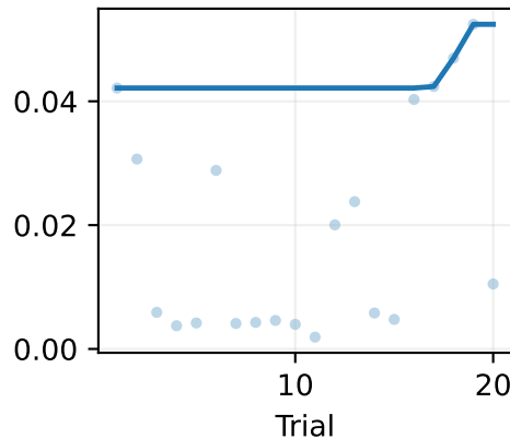
amazon-music · CDAE
