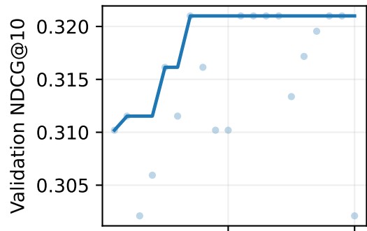
amazon-music · EASE
