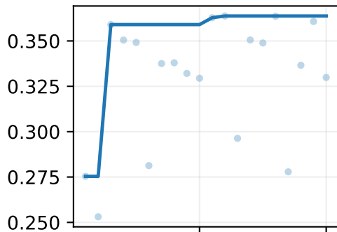
amazon-music · CDAE
