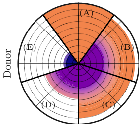
Hydrogen
