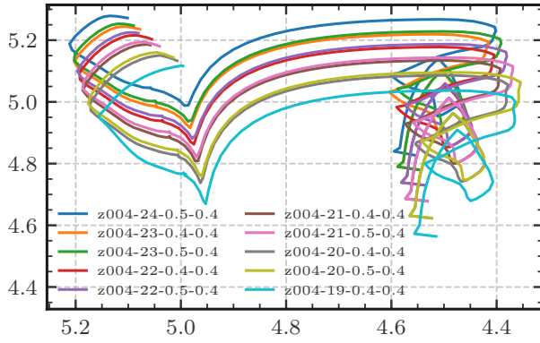
(c) SMC 108086
