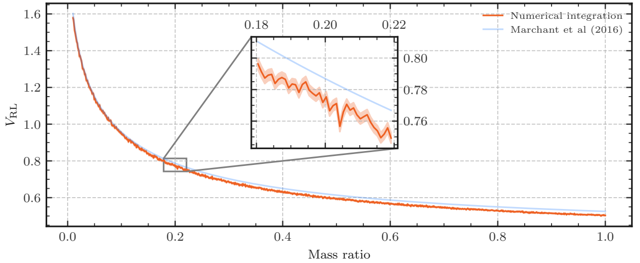
Figure 2.10: As for figure 2.9, but for the \mathcal{L}_2 point with formula given by eqn(2.16) (Marchant et al., 2016).
