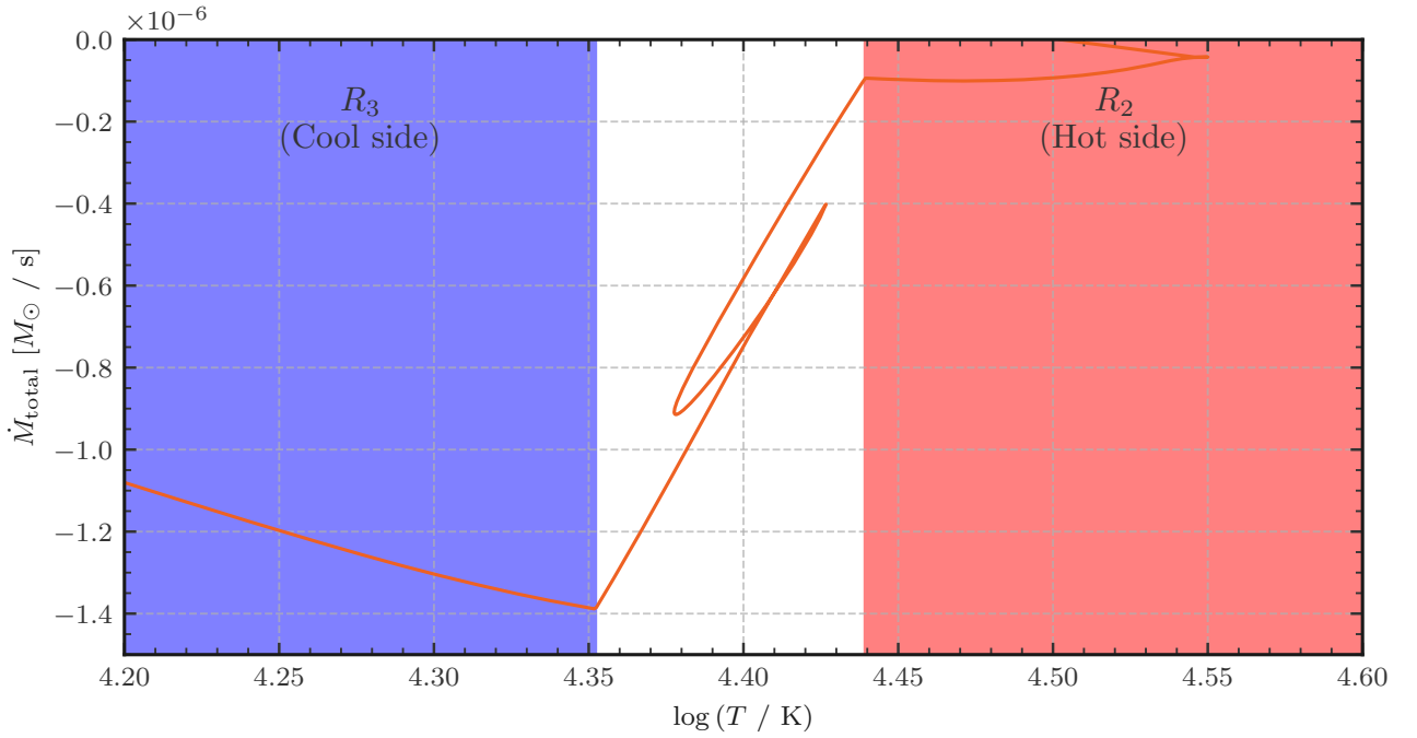
Figure F.1: An illustration of the bi-stability jump at \log T \approx 4.4 . This illustration was computed for a 21 M_{\odot} star. Shown in blue is the cool side of the bistability jump, where R_3 (eqn(F.5)) is the interpolation, and shown in red is the hot side, where R_2 (eqn(F.4)) is the interpolation.
