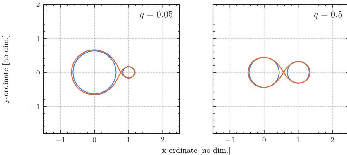
Figure 2.8: A schematic of the Roche lobe formula eqn(2.15). Here, the exact solution to the Roche lobe formula \xi in eqn(2.14) (orange) vs the fit provided by Eggleton (1983) (blue). Although precise details of the Roche lobe, such as the apex of the teardrop at the point \xi , are lost, the volume is preserved to within 1 per cent accuracy over all mass ratios.
