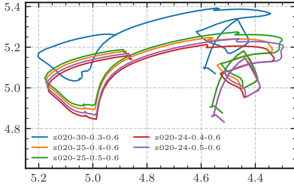
(a) LSS 3074
