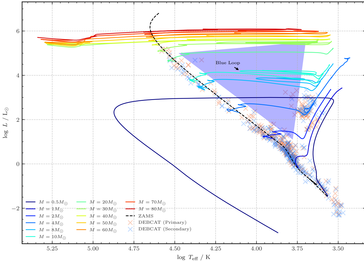
Figure 2.2: The evolution of stars in the range 0.5 - 80 M_{\odot} . The dashed black line represents the Zero-Age Main Sequence (ZAMS), which is the origin point of all of our models, and (in this plot) extends from 0.5 M_{\odot} to 300 M_{\odot} . The blue triangle is the (highly approximate) bounds of the Hertzsprung gap. Crosses indicate binaries in the Double Eclipsing Binaries catalogue (DEBCAT; Southworth, 2015), and illustrate the apparent “zone of avoidance” that defines the Hertzsprung gap.
