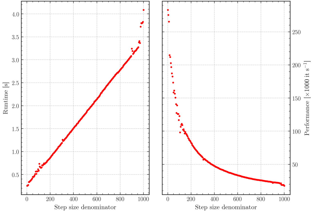
Figure 6.3: The effect of varying de in eqn(6.5) on the runtime, which is demonstrably \mathcal{O}(n) , and the performance of the algorithm. The input data to this algorithm were the LISA binary sample from Tang (priv. comm.). The performance is shown in units of thousands of iterations per second.
