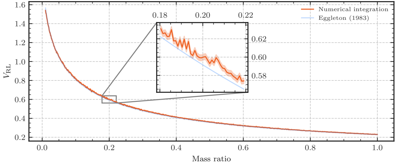
Figure 2.9: The volume of the Roche Lobe computed numerically through Monte-Carlo integration (orange) vs the volume assuming eqn(2.15) (blue). The Eggleton approximation fits well to the volume, with around 1 per cent error across the entire mass ratio range (truncated here to q \leq 1 ).
