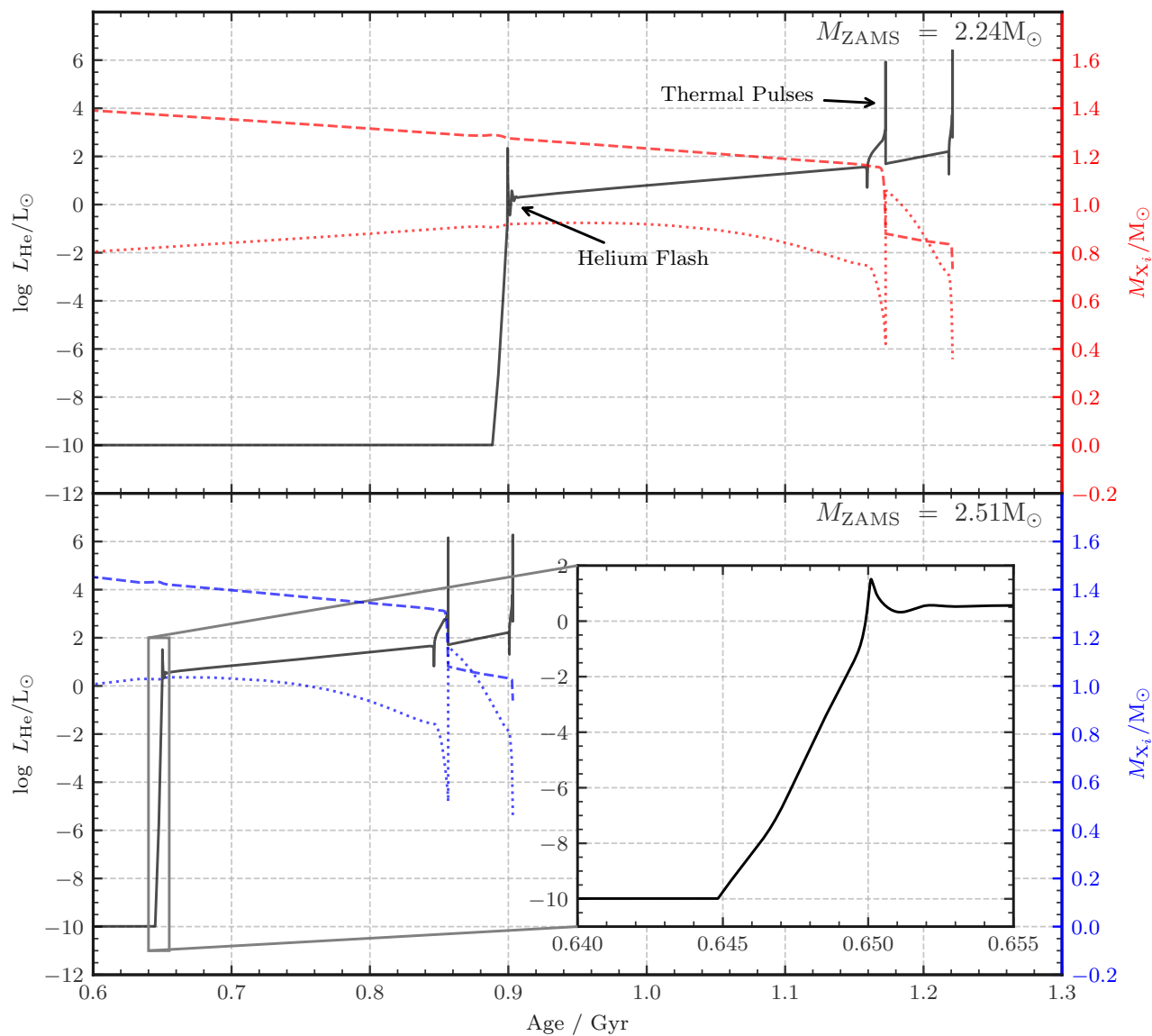
Figure 2.11: Two stars of a similar mass that undergo a helium flash and two thermal pulses. Shown in the inset is a zoomed-in helium flash that lasts \sim 7 Myr. Both stars undergo two thermal pulses before the code crashes due to the relative error in the calculation increasing too rapidly. The two stars could, in principle, undergo many more thermal pulses before their deaths.
