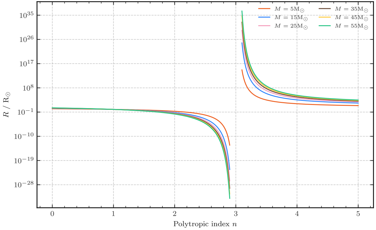
Figure E.1: The radius of stars of varying mass as a function of the polytropic index they are modelled at.
