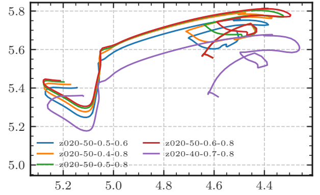
(b) MY Camelopardalis
