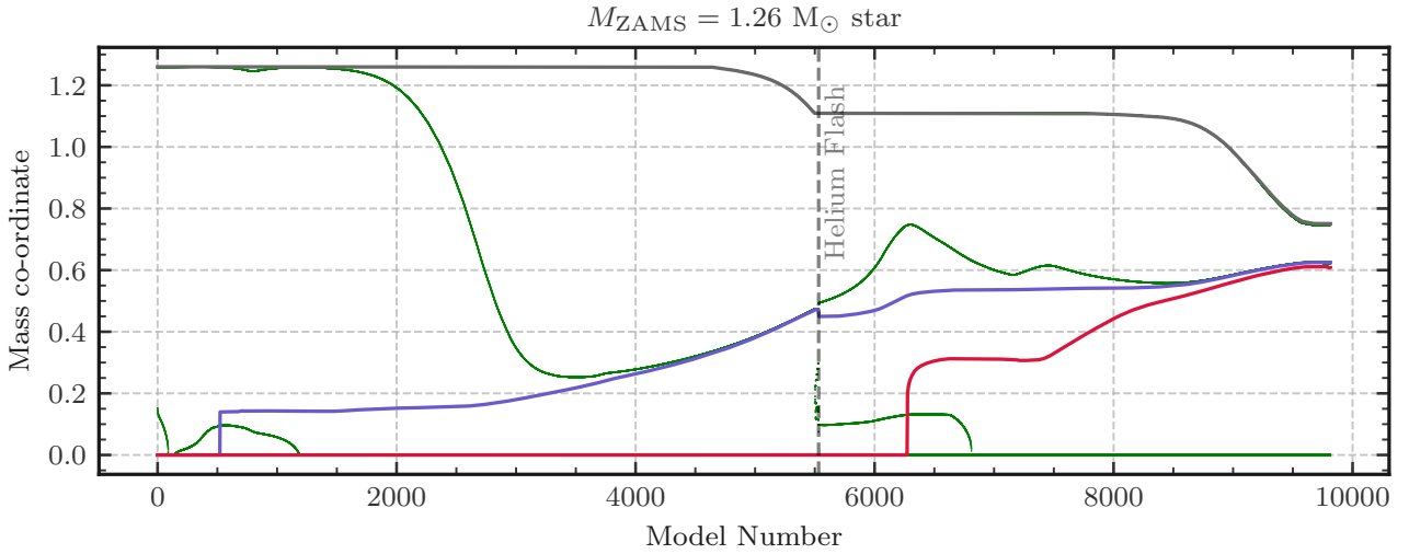
Figure 2.12: The helium flash (gray dashed line) shown on a Kippenhahn diagram. There is a slight discontinuity in the helium core mass (blue) due to a perfect match not existing in the 3 M_{\odot} reference model. The total mass is shown as the solid gray line, and the CO core mass is shown in red. The green lines show the boundaries of the convective regions of the star. [TODO: vectorize]
