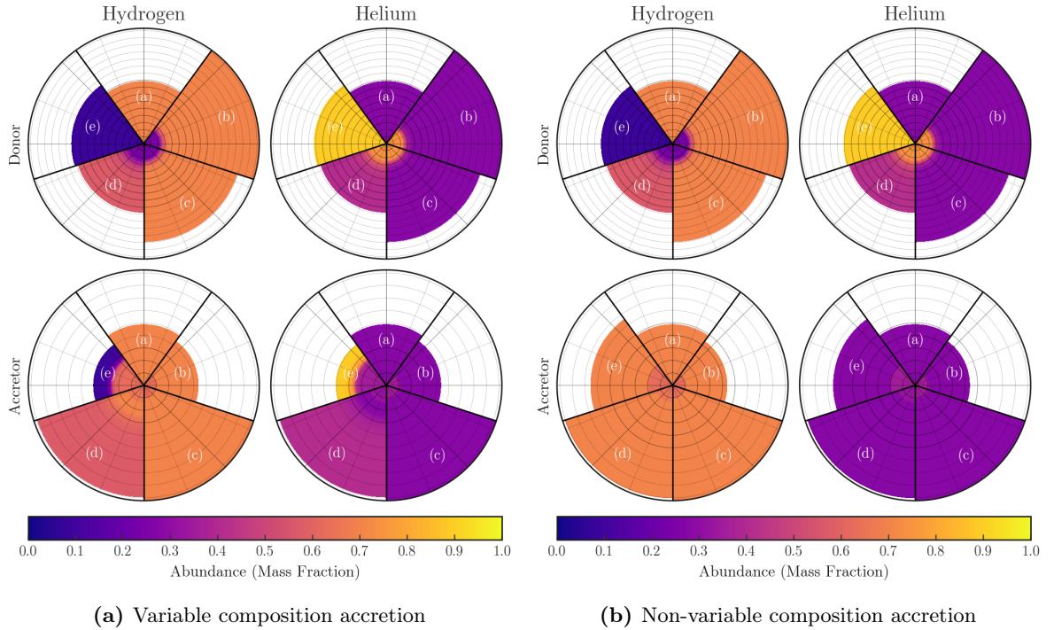
Figure 4.4: The chemical composition of each star as a function of the stellar radius for the donor and accretor at the five key stages of the binary's lifetime as detailed in table 4.2. Letters are as given in the same table. Each grid marking in the radial direction represents 1 R_{\odot} .
