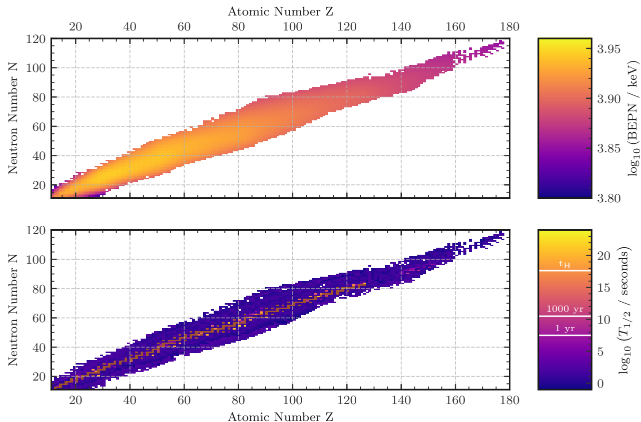
Figure 2.5: Top: The binding energy per nucleon and half-lives for elements up to Oganesson. The most stable element of fusion here is Nickel-62. Elements lighter than Nickel-62 will fuse towards it, and elements heavier will undergo fission to reach it. Bottom: The half-life in seconds across the same isotopes. Marked on the colorbar axis are 1 yr, 1000 yr, and t_H = 13.8 \text{ Gyr} . Stable elements are marked in brown. Underlying data for both plots are from the International Atomic Energy Agency.
