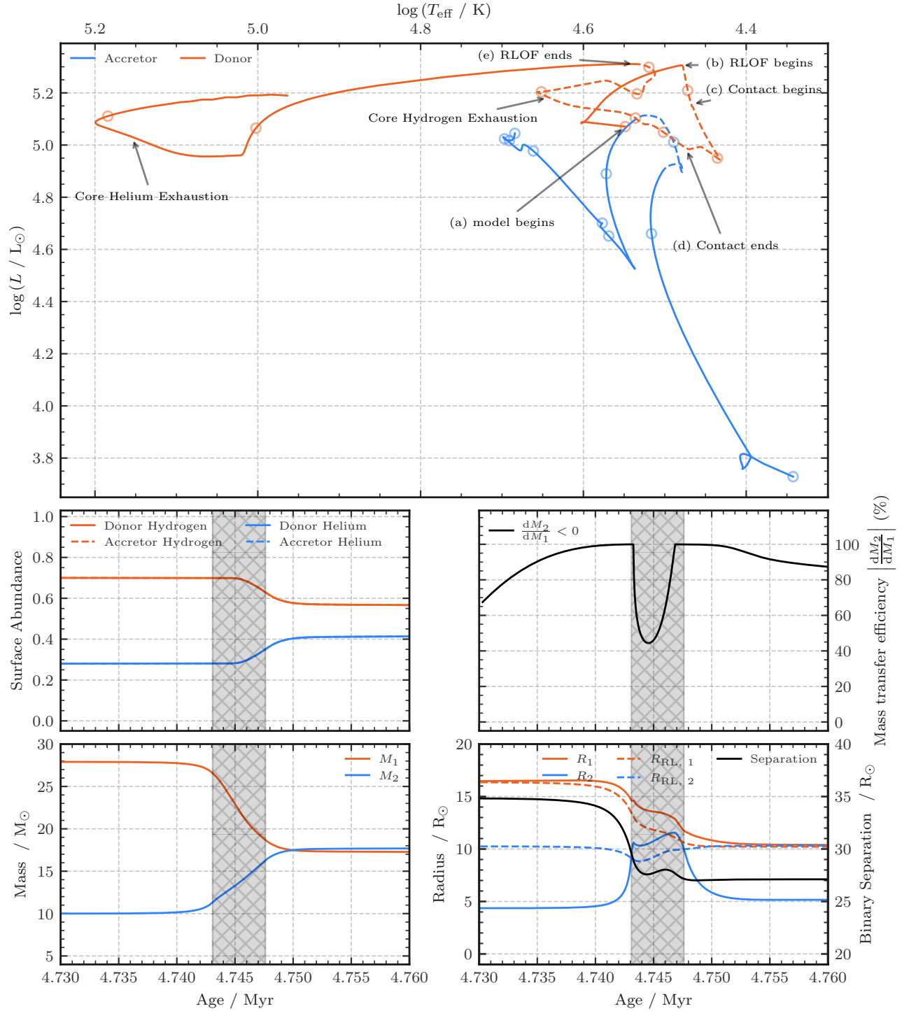
Figure 4.1: The main evolution of a 30 + 10 M_{\odot} binary with variable composition accretion enabled. Clockwise from top: the HR diagram with stages in figure 4.4 and table 4.2, the mass transfer efficiency, the separation / radius, the mass, and the surface abundances. In the lower four plots, the gray region shows the contact phase, and the plots are cropped to show the \sim 13 kyr on each side of the contact phase. The dashed line on each HR diagram track shows when the relevant star is overfilling \mathcal{L}_1 , and contact is when both stars are dashed.
