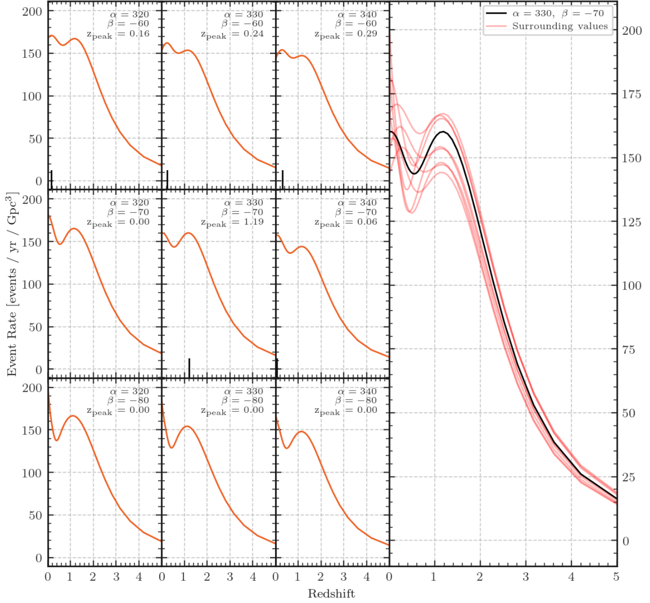
Figure 6.13: The event rate \mathcal{R}(z) for a region surrounding \alpha = 330, \beta = -70 on FINEGRID. This region corresponds to the “outlier” in figure 6.12. Shown on the left are the outlier bin in the center and its neighbours in both \alpha -space and \beta -space. The black line on each plot denotes the location in redshift of the event rate distribution peak. The right plot shows the outlier in black and its neighbours in faded red behind.
