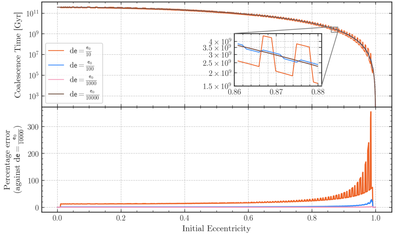
Figure 6.2: The effect of varying de in eqn(6.5) on the coalescence time. Although hard to see, the pink line does oscillate above and below the brown line. This binary was assumed to have m_1 = m_2 = 1.44 M_\odot and a_0 = 1970.5 R_\odot (the mean separation of a sample of binaries with \alpha = 100 \text{ km s}^{-1} , \beta = -170 \text{ km s}^{-1} ).
