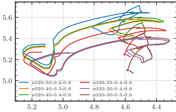
(e) V382 Cygni
