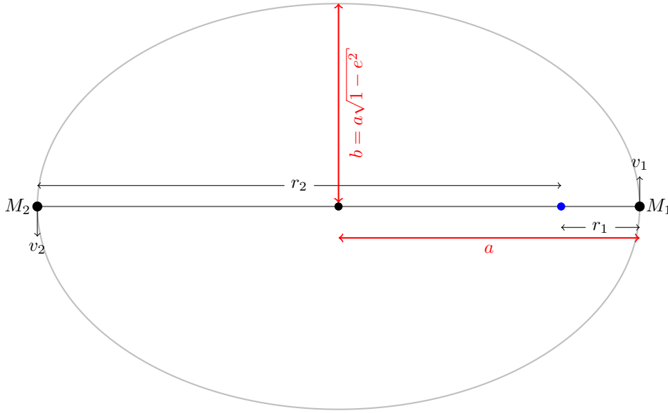
Figure 2.6: A schematic of a simple binary star system with eccentricity e , semimajor axis a , and semiminor axis b . The centre of mass (barycentre) is shown as a blue dot. Here, M_1 is the heavier star, which orbits at a smaller distance r_1 to the barycentre by Kepler's first and Newton's second laws. The elliptical orbital trajectory is shown in grey. Figure adapted from Richards (2021).
