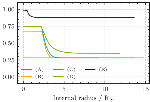
Helium Abundance
