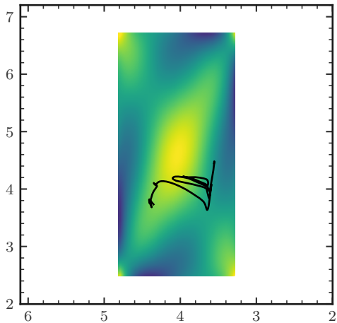
Chebyshev
