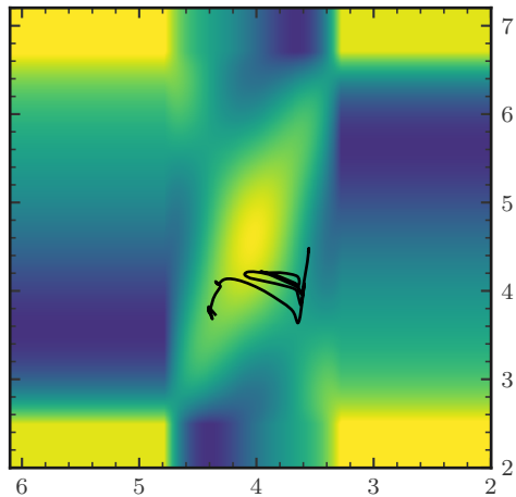
Chebyshev (bounded parameters)
