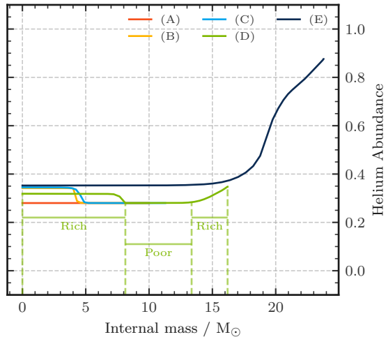
Accretor
