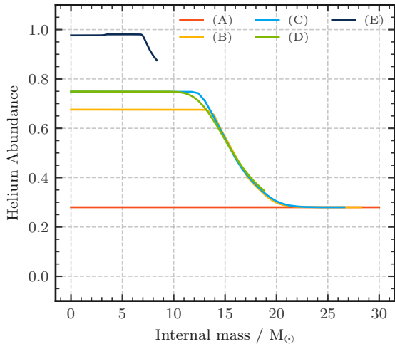
Donor
