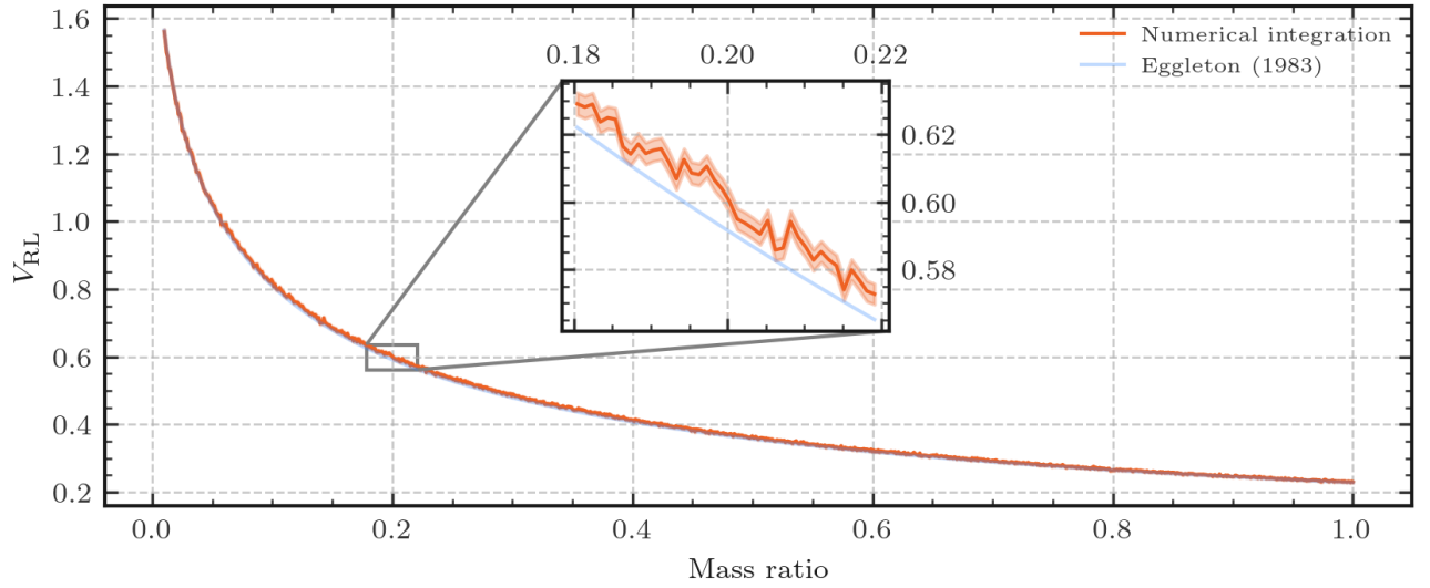
Figure 2.8: The volume of the Roche Lobe computed numerically through Monte-Carlo integration (orange) vs the volume assuming Equation 2.30 (blue). The Eggleton approximation fits well to the volume, with around 1 per cent error across the entire mass ratio range (truncated here to q \leq 1 ).
