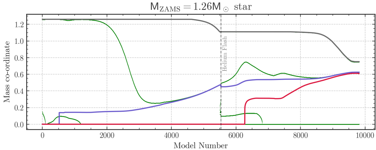
Figure 2.12: The helium flash (gray dashed line) shown on a Kippenhahn diagram. There is a slight discontinuity in the helium core mass (blue) due to a perfect match not existing in the 3 M_{\odot} reference model. The total mass is shown as the solid gray line, and the CO core mass is shown in red. The green lines show the boundaries of the convective regions of the star.
