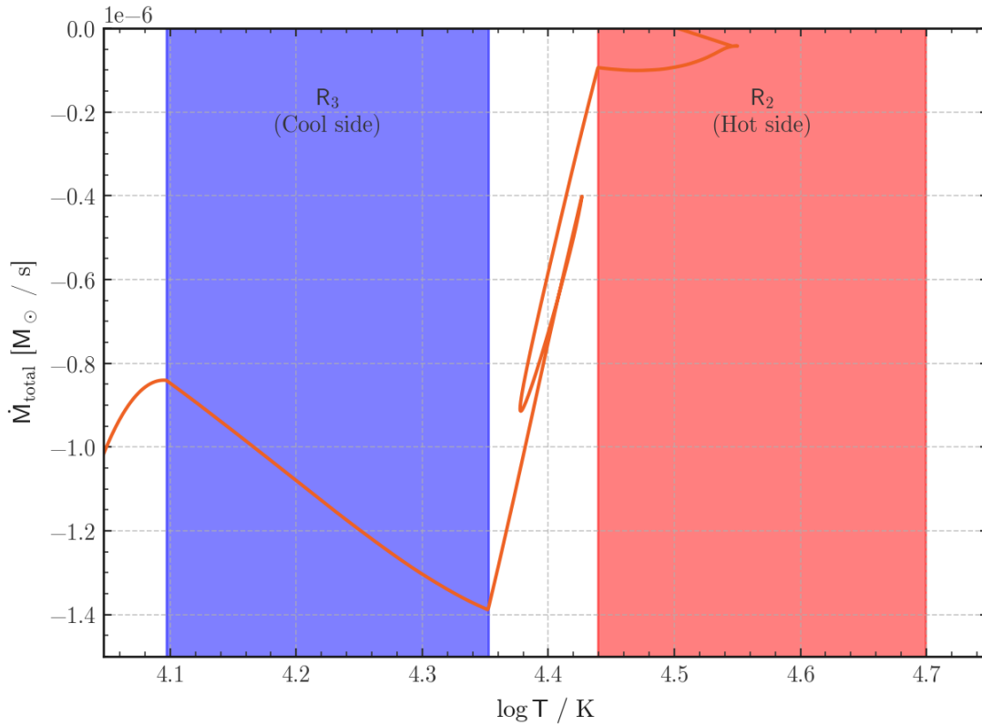
Figure 2.10: An illustration of the bi-stability jump at \log T \approx 4.4 . This illustration was computed for a 21 M_{\odot} star. Shown in blue is the cool side of the bistability jump, where R_3 (Equation 2.48) is the interpolation, and shown in red is the hot side, where R_2 (Equation 2.47) is the interpolation.
