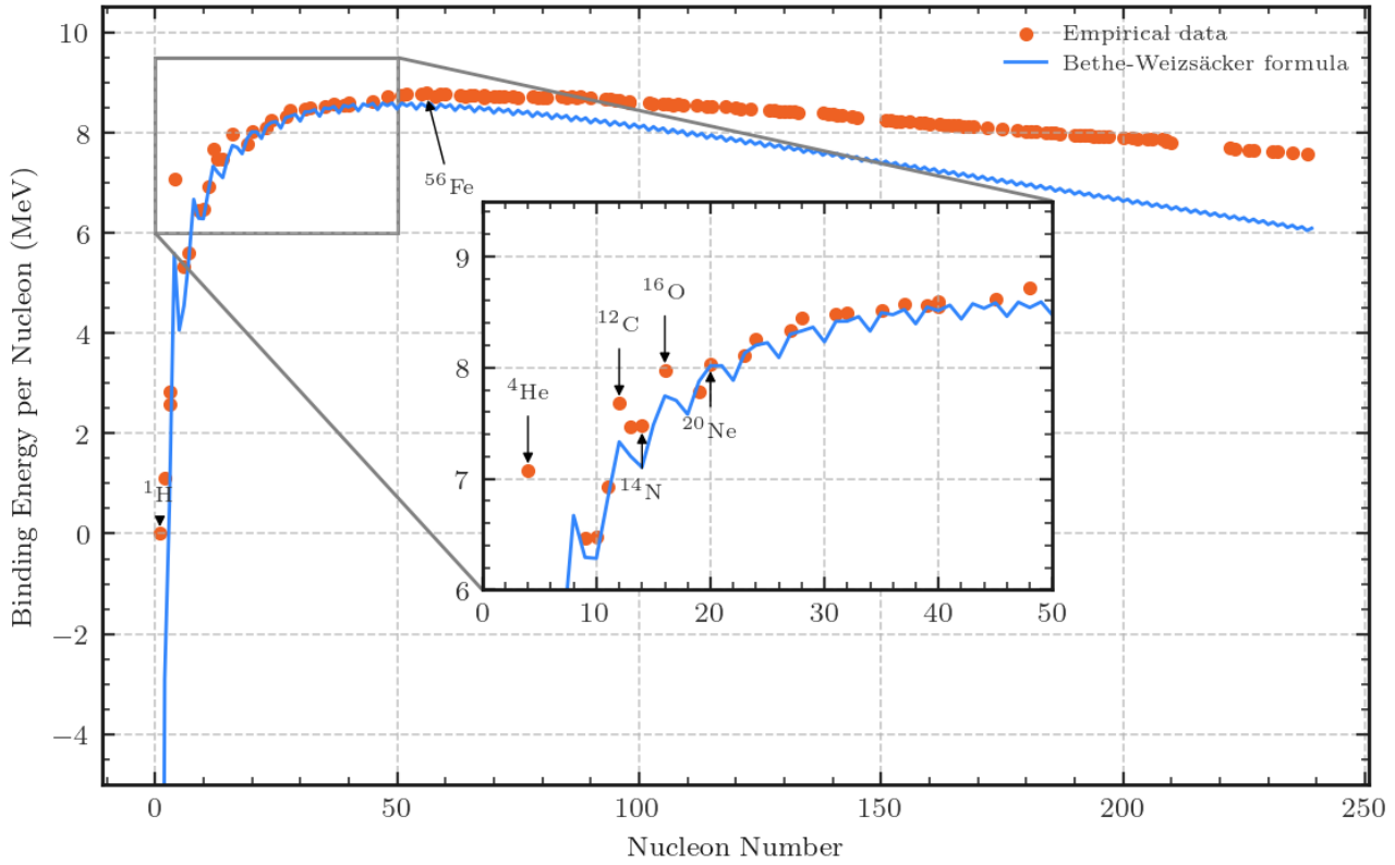
Figure 2.4: The binding energy per nucleon for elements up to Uranium-238. The most stable element of fusion here is Iron-56. Elements lighter than Iron-56 will fuse towards it, and elements lighter will undergo fission to reach it. Graph adapted from Fastfission on Wikimedia Commons (who released it into the public domain).
