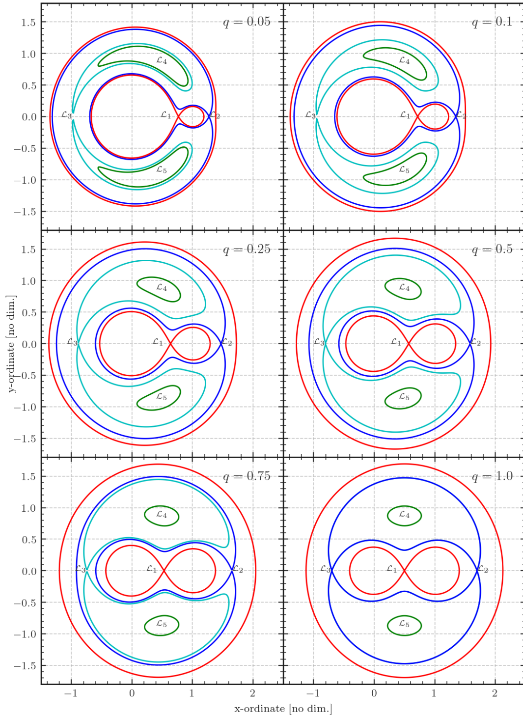
Figure 2.6: The dimensionless Roche potential as a function of mass ratio q . Note that the shape of the Roche potential changes markedly at low mass ratio, and changes more slowly as the mass ratio approaches unity. Distances have been normalised such that the primary star is at (x, y, z) = (0, 0, 0) and the secondary star is at (x, y, z) = (1, 0, 0) , i.e., we measure distances in units of separation and that the coordinate system is centered on the primary star.
