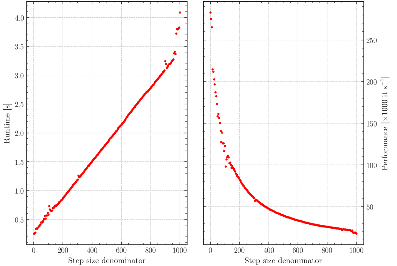
Figure 5.3: The effect of varying d\epsilon in Equation 5.5 on the runtime, which is demonstrably \mathcal{O}(n) , and the performance of the algorithm. The input data to this algorithm were the LISA binary sample from Tang (priv. comm.). The performance is shown in units of thousands of iterations per second.
