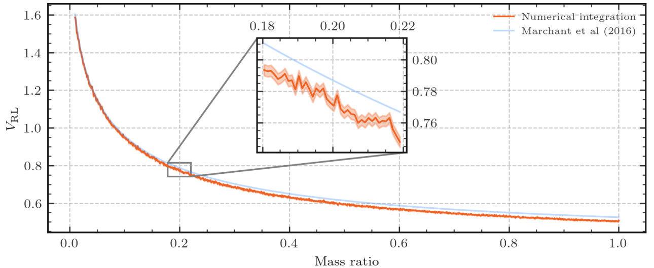
Figure 2.9: As for Figure 2.8, but for the \mathcal{L}_2 point with formula given by Equation 2.31 (Marchant et al., 2016).
