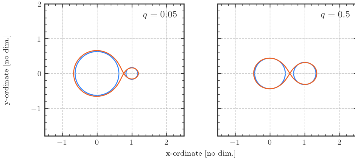
Figure 2.7: A schematic of the Roche lobe formula Equation 2.30. Here, the exact solution to the Roche lobe formula \xi in Equation 2.29 (orange) vs the fit provided by Eggleton (1983) (blue). Although precise details of the Roche lobe, such as the apex of the teardrop at the point \xi , are lost, the volume is preserved to within 1 per cent accuracy over all mass ratios.
