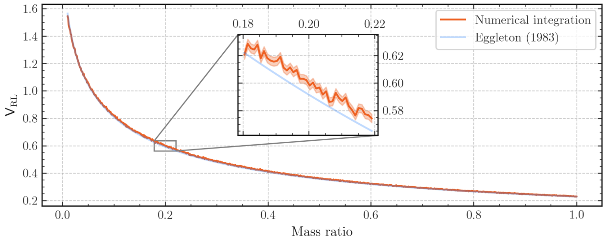
Figure 2.4: The volume of the Roche Lobe computed numerically through Monte-Carlo integration (orange) vs the volume assuming Equation 2.36 (blue). The Eggleton approximation fits well to the volume, with around 1 per cent error across the entire mass ratio range (truncated here to q \leq 1 ).
