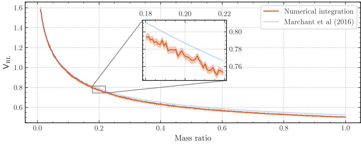
Figure 2.5: As for Figure 2.4, but for the \mathcal{L}_2 point with formula given by Equation 2.37 ( Marchant et al., 2016 ).
