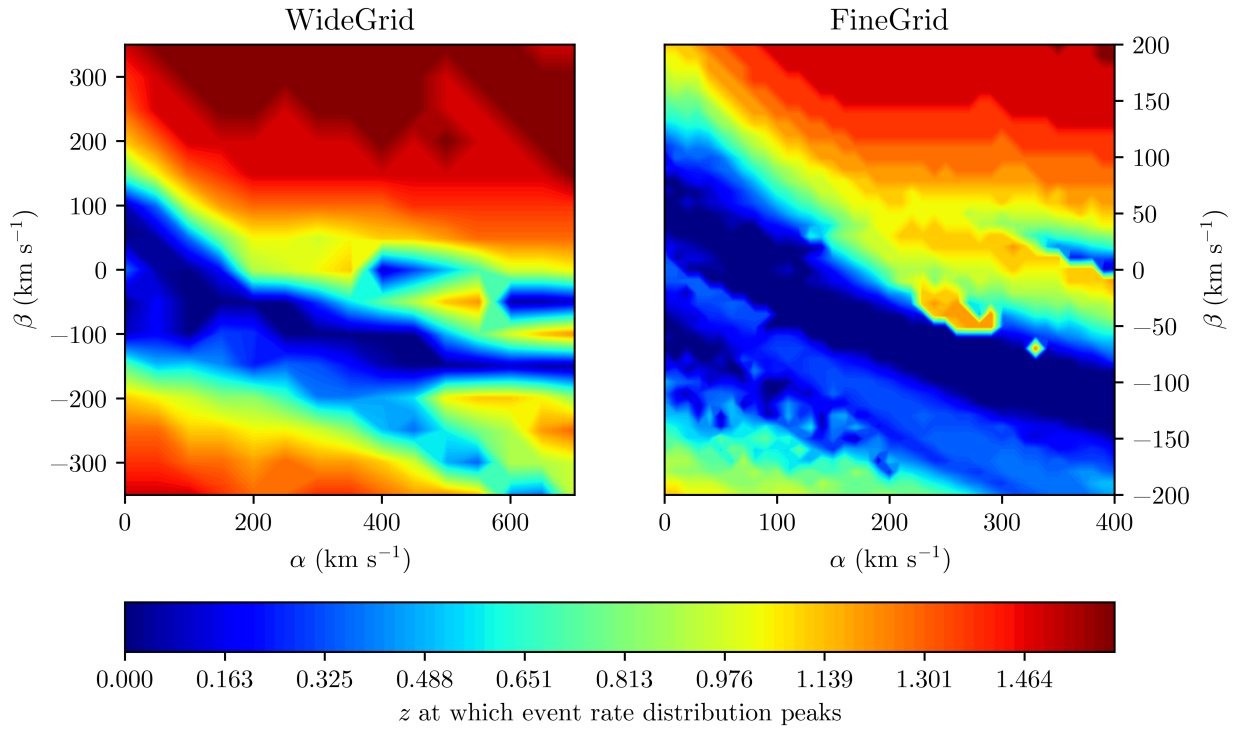
Figure 4.8: The peak of the event rate \mathcal{R}(t) as a function of \alpha and \beta . Varying these two parameters generally brings the peak closer to the present day ( z = 0 ). Absent a merger rate (or, more formally, assuming the merger rate is instantaneous and given by a Dirac-delta function), the SFRD peaks at z \sim 1.863 .
