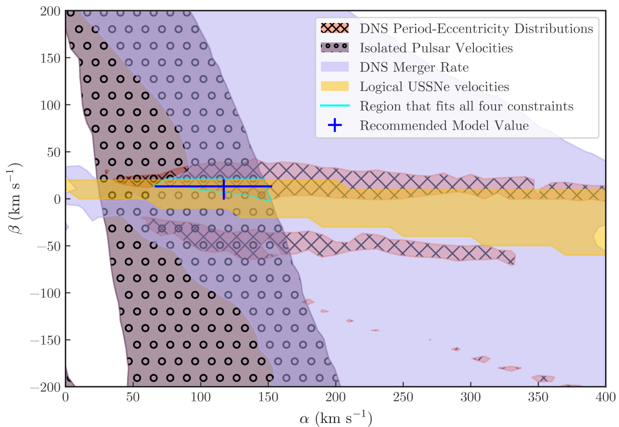
Figure 4.6: The four constraints we apply overlaid on our FINEGRID parameter space. The cyan region represents the region which fits all four parameters, and the blue cross represents the “center of mass” of this region.
