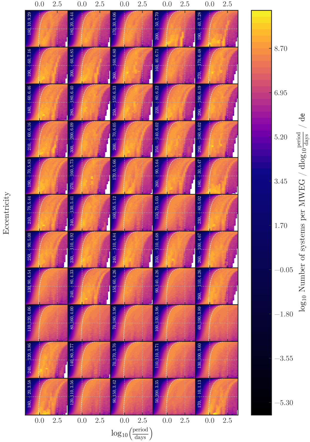
Figure B.1: The period-eccentricity distributions of populations governed by Bray kicks across the LIGO O3 contour. The combination of \alpha and \beta used in the kick prescription is given in white along the left side of each plot. White regions denote no systems passing through those bins.
