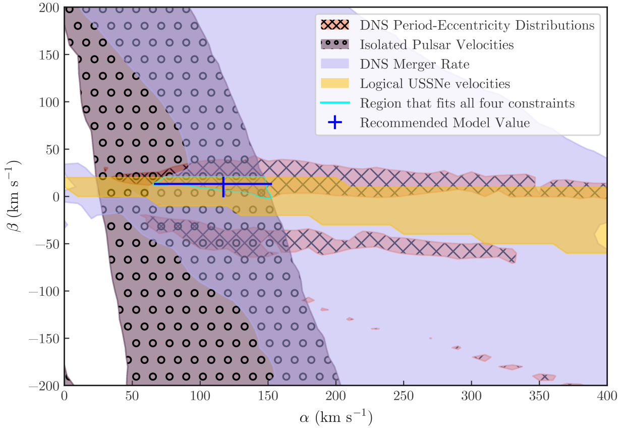
Figure 5.8: The four constraints we apply overlaid on our FINEGRID parameter space. The cyan region represents the region which fits all four parameters, and the blue cross represents the “center of mass” of this region.
