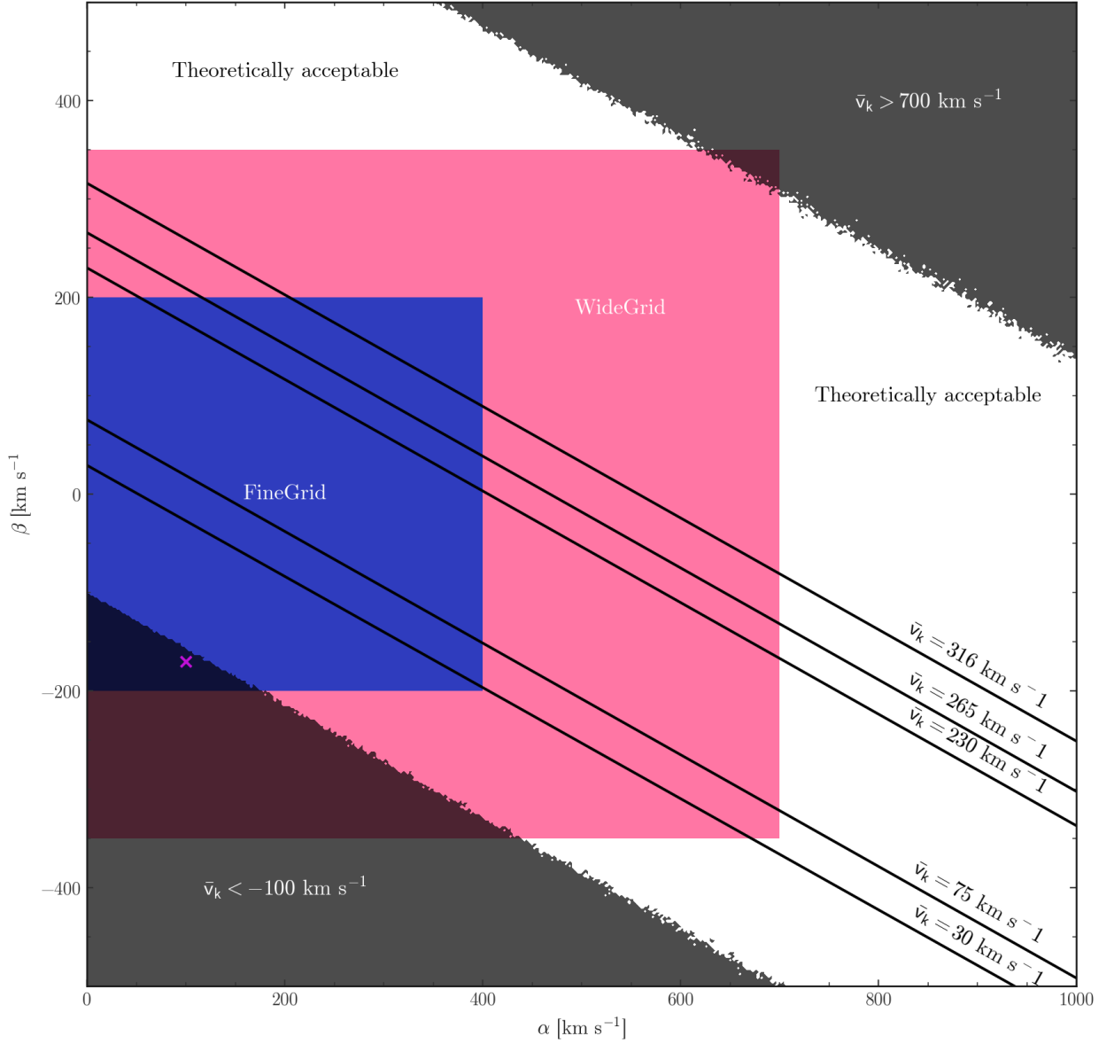
Figure 5.1: A schematic of how FINEGRID and WIDEGRID are related. The mean kick velocity \bar{v}_k was computed by averaging the kick velocities of 1,000 simulated kicks for each combination of \alpha and \beta , with m_{\text{rem}} \in [0.1, 2.5] and m_{\text{ej}} \in [0.1, m_{\text{rem}}] sampled uniformly. The pink cross represents the point \alpha = 100, \beta = -170 , which are the fiducial kick parameters from Bray & Eldridge (2018) .
