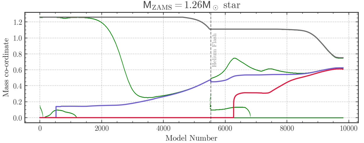
Figure 2.9: The helium flash (gray dashed line) shown on a Kippenhahn diagram. There is a slight discontinuity in the helium core mass (blue) due to a perfect match not existing in the 3 M_{\odot} reference model. The total mass is shown as the solid gray line, and the CO core mass is shown in red. The green lines show the boundaries of the convective regions of the star.
