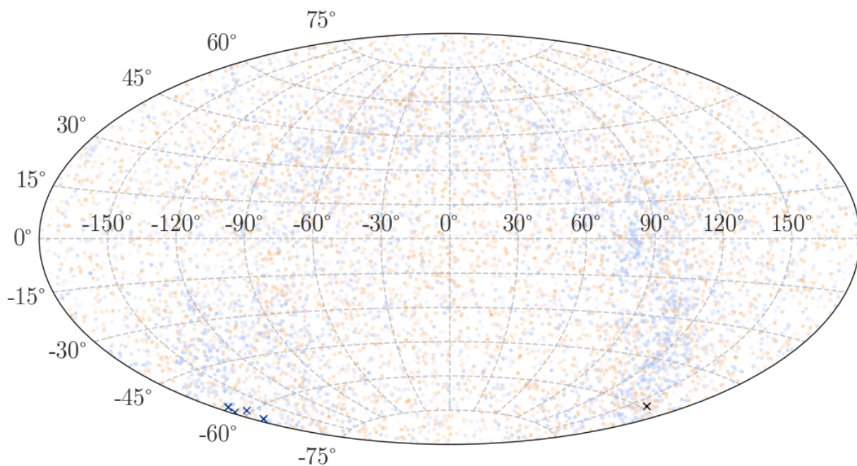
Figure A.1: The locations of the \sim 9000 stars in the night sky visible to the naked eye, as reported in Hoffleit (1964). The colors are computed by converting the B-V color indices to temperatures using the fits in Ballesteros (2012), and then converted to RGB via the algorithm in this StackOverflow post: https://stackoverflow.com/a/45497817 . Transparency correlates to the magnitude of the stars; fainter stars (higher magnitudes) have high transparency. The Southern Cross (Crucis) is shown fully opaque in blue towards the bottom left of the plot as a point of reference, and \eta Carinae is shown fully opaque in black in the bottom right.
