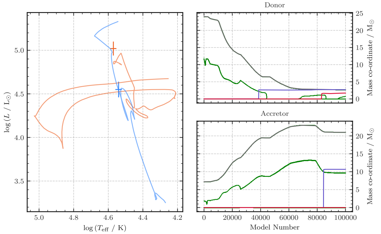
(b) The second match for TU Muscae ( M_1 = 24 M_{\odot} , M_2 = 7.2 M_{\odot} , \log(P / \text{d}) = 0.3 ).
