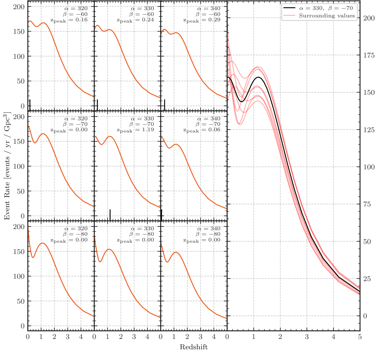
Figure 4.13: The event rate \mathcal{R}(z) for a region surrounding \alpha = 330, \beta = -70 on FINEGRID. This region corresponds to the “outlier” in Figure 4.12. Shown on the left are the outlier bin in the center and its neighbours in both \alpha -space and \beta -space. The black line on each plot denotes the location in redshift of the event rate distribution peak. The right plot shows the outlier in black and its neighbours in faded red behind.
