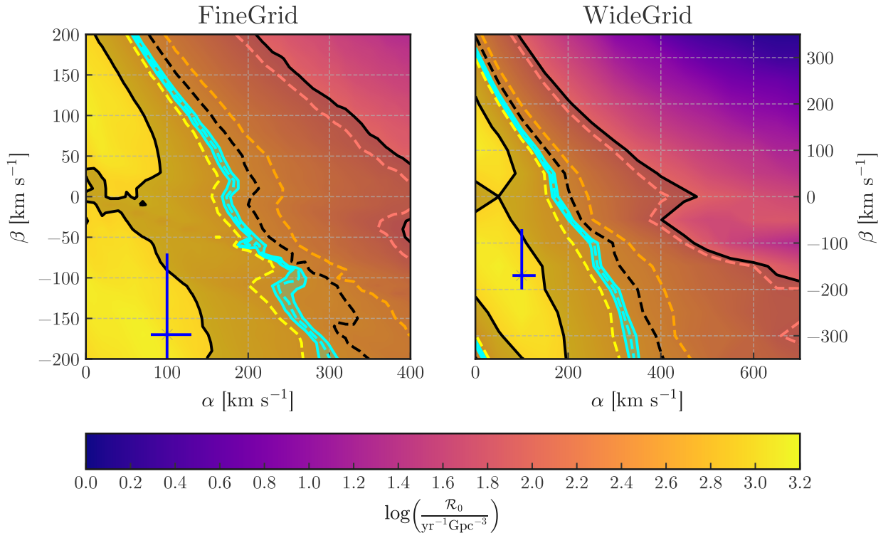
Figure 4.5: The merger rate as a function of kick parameters \alpha and \beta . The cyan contour is the theoretical merger rate as reported by Eldridge et al. (2019). The black contour is the merger rate observed in LIGO-Virgo (2021). The remaining contours are the merger rates reported in LIGO-Virgo-KAGRA (2021) (pink: BGP, yellow: MS, orange: PDB [ind], see LIGO-Virgo-KAGRA (2021) for an explanation of each model). Shaded regions represent uncertainties, and uncertainties are not reported for the LIGO-Virgo-KAGRA (2021) results as they would cover the entire plane. The blue cross is the fiducial value of \alpha and \beta from Bray & Eldridge (2018). This value lies off the previous work’s contours as the rejuvenation age calculation has been improved in TUI in preparation for the next major BPASS release.
