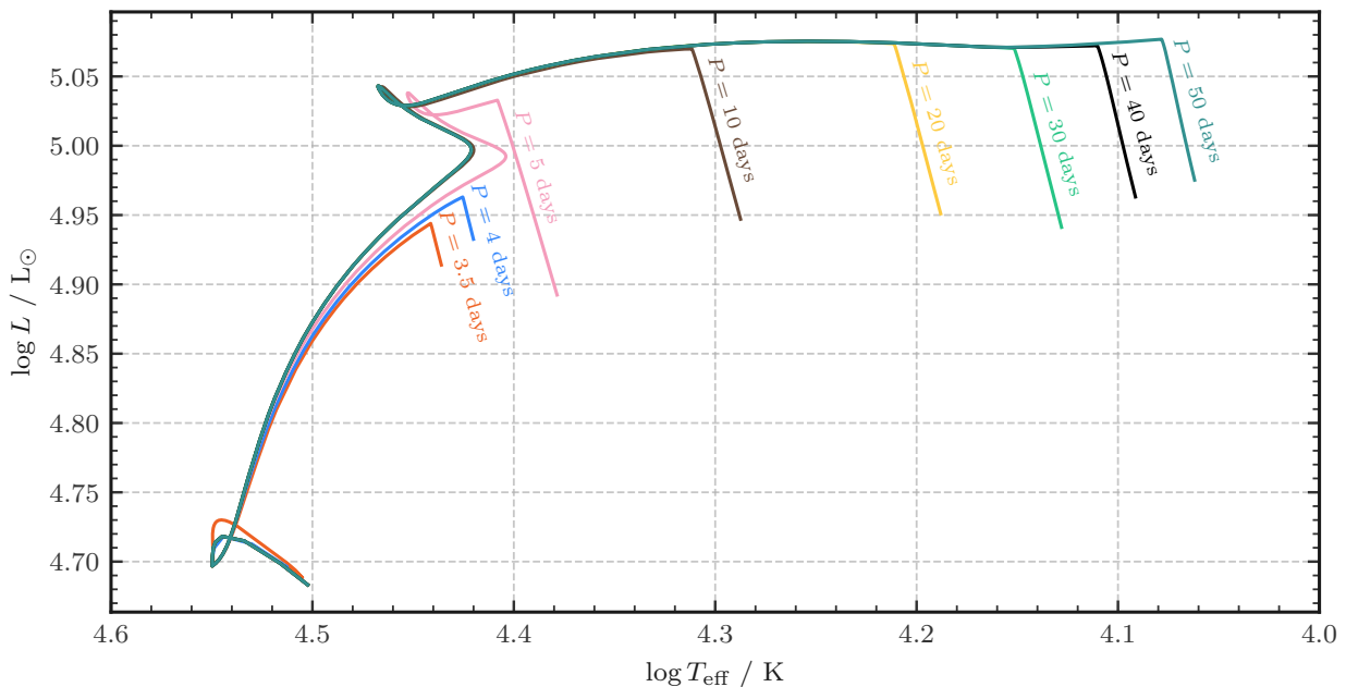
Figure 2.7: The HRD for an 21 M_{\odot} star with an (unshown) 10 M_{\odot} companion with varying period. In this figure, only the initial binary period was free to change between runs. Short periods interact closer to the MS. The evolution was terminated 1,000 models after the primary star achieved RLOF for the first time.
