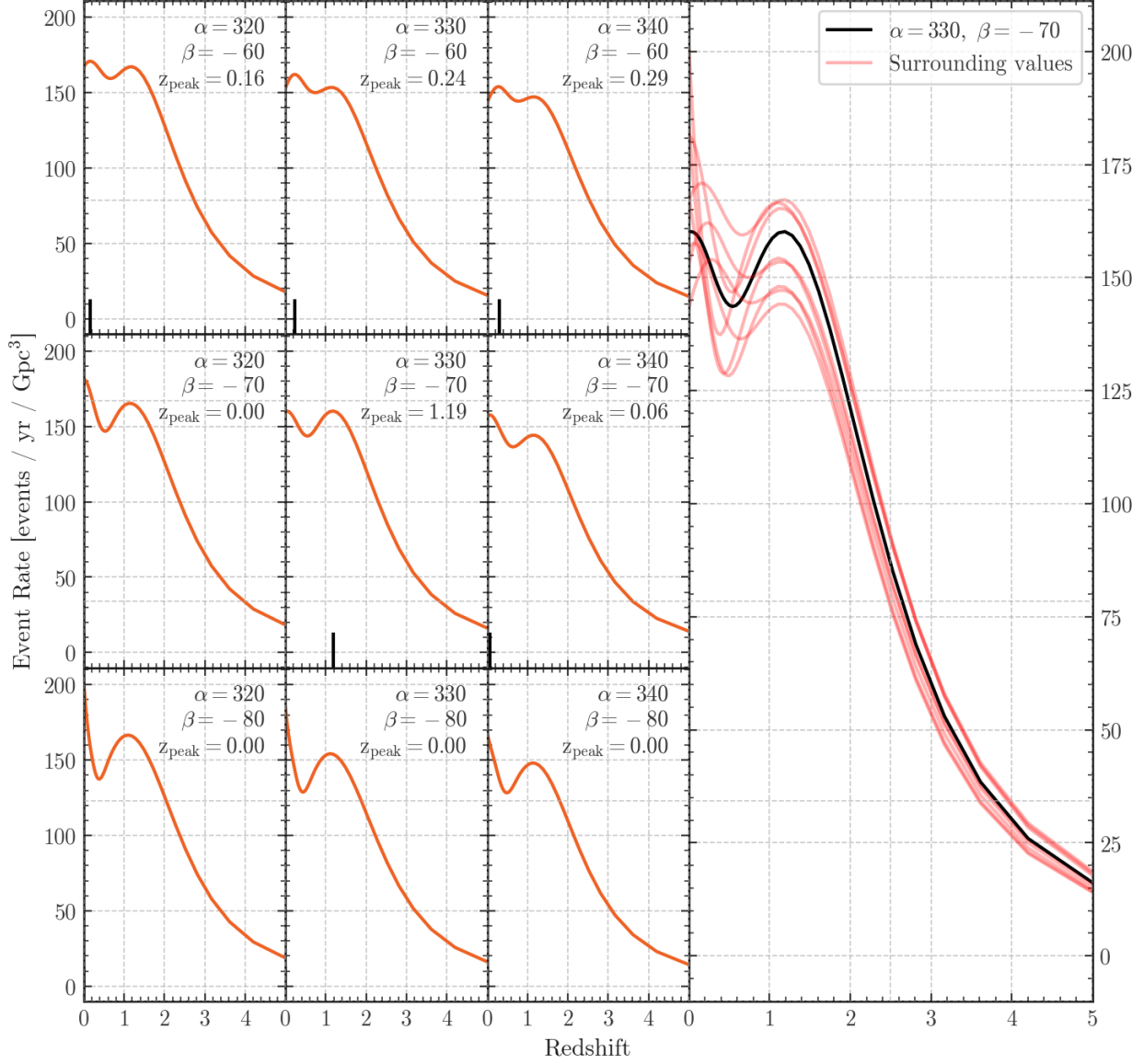
Figure 4.10: The event rate \mathcal{R}(z) for a region surrounding \alpha = 330, \beta = -70 on FINEGRID. This region corresponds to the “outlier” in Figure 4.9. Shown on the left are the outlier bin in the center and its neighbours in both \alpha -space and \beta -space. The black line on each plot denotes the location in redshift of the event rate distribution peak. The right plot shows the outlier in black and its neighbours in faded red behind.
