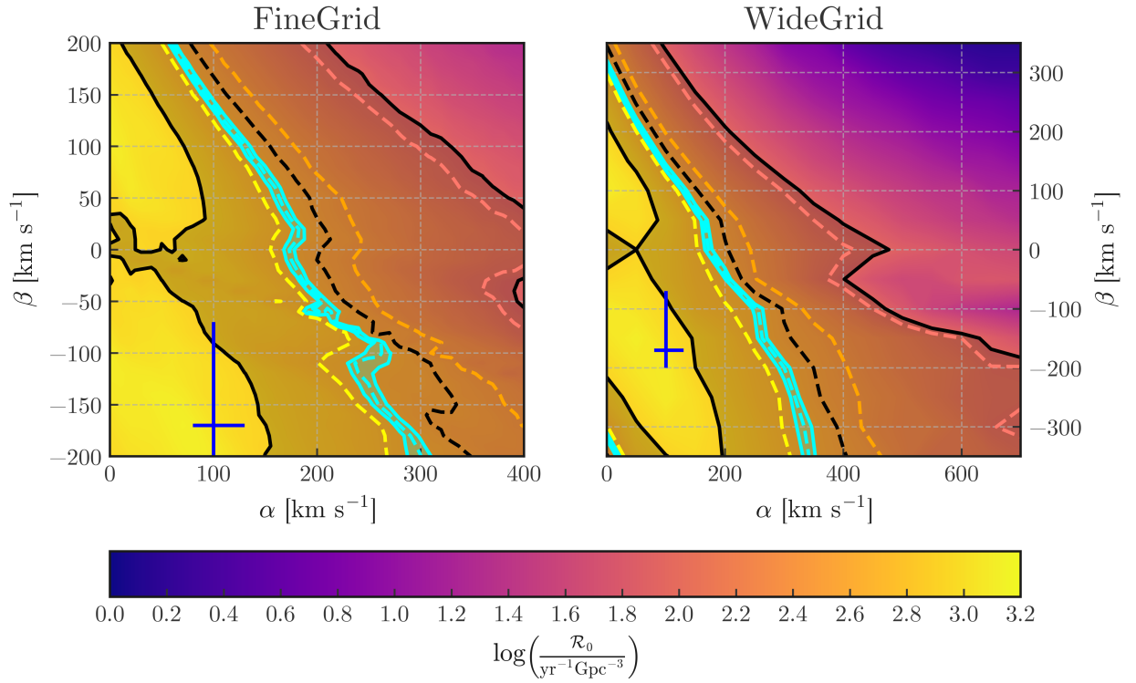
Figure 4.3: The merger rate as a function of kick parameters \alpha and \beta . The cyan contour is the theoretical merger rate as reported by Eldridge et al. (2019) . The black contour is the merger rate observed in LIGO-Virgo (2021) . The remaining contours are the merger rates reported in LIGO-Virgo-KAGRA (2021) (pink: BGP, yellow: MS, orange: PDB [ind], see LIGO-Virgo-KAGRA (2021) for an explanation of each model). Shaded regions represent uncertainties, and uncertainties are not reported for the LIGO-Virgo-KAGRA (2021) results as they would cover the entire plane. The blue cross is the fiducial value of \alpha and \beta from Bray & Eldridge (2018) . This value lies off the previous work’s contours as the rejuvenation age calculation has been improved in TUI in preparation for the next major BPASS release.
