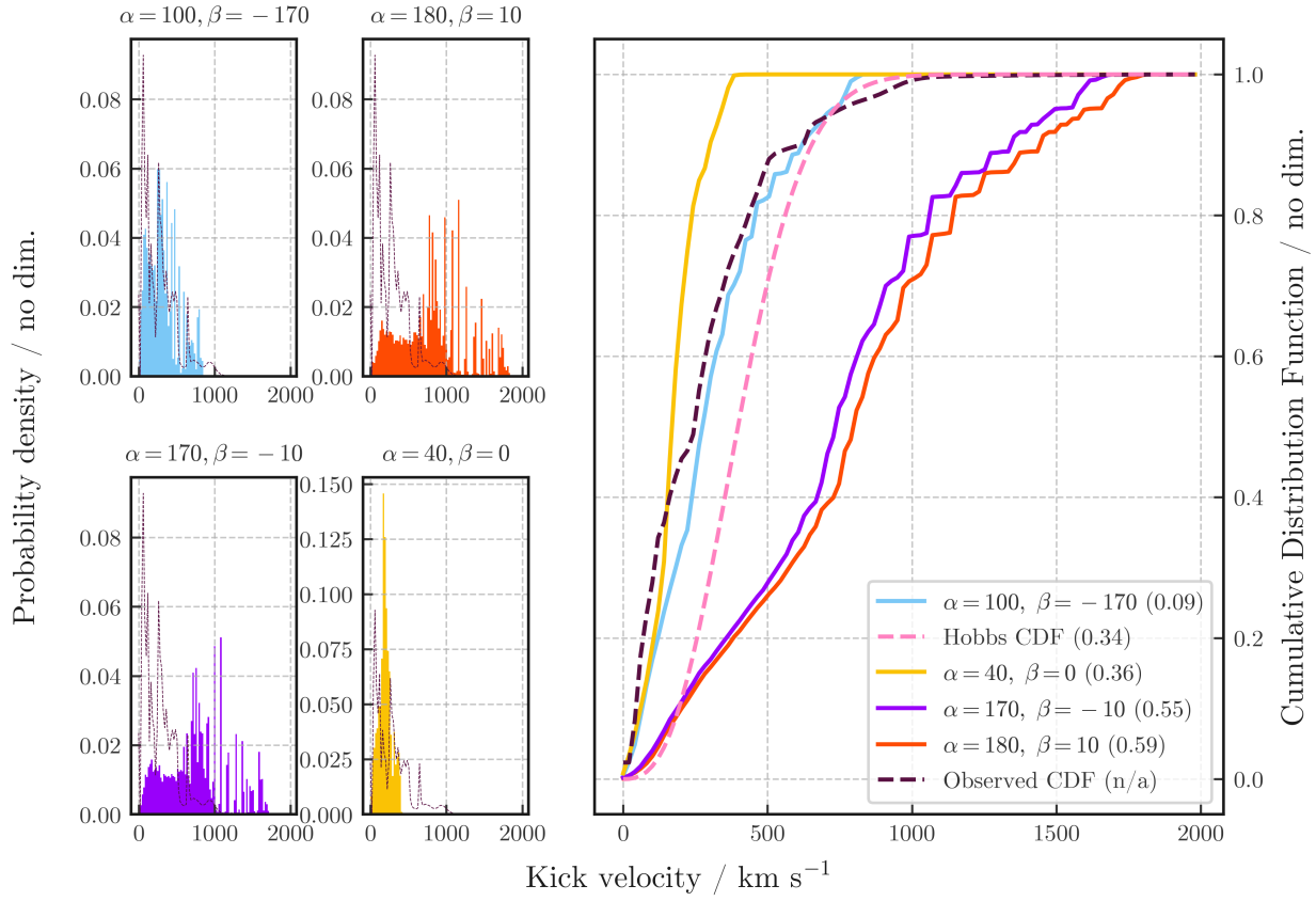
Figure 4.6: The PDFs and CDFs of four systems, alongside the Hobbs CDF and Willcox et al. (2021) CDF. The dashed line on the PDF plots is the PDF of the observed distribution from Willcox et al. (2021). On the right hand plot, the number in parentheses represents the K-S statistic for the distribution, measured relative to Willcox et al. (2021), which by definition has no K-S statistic.
