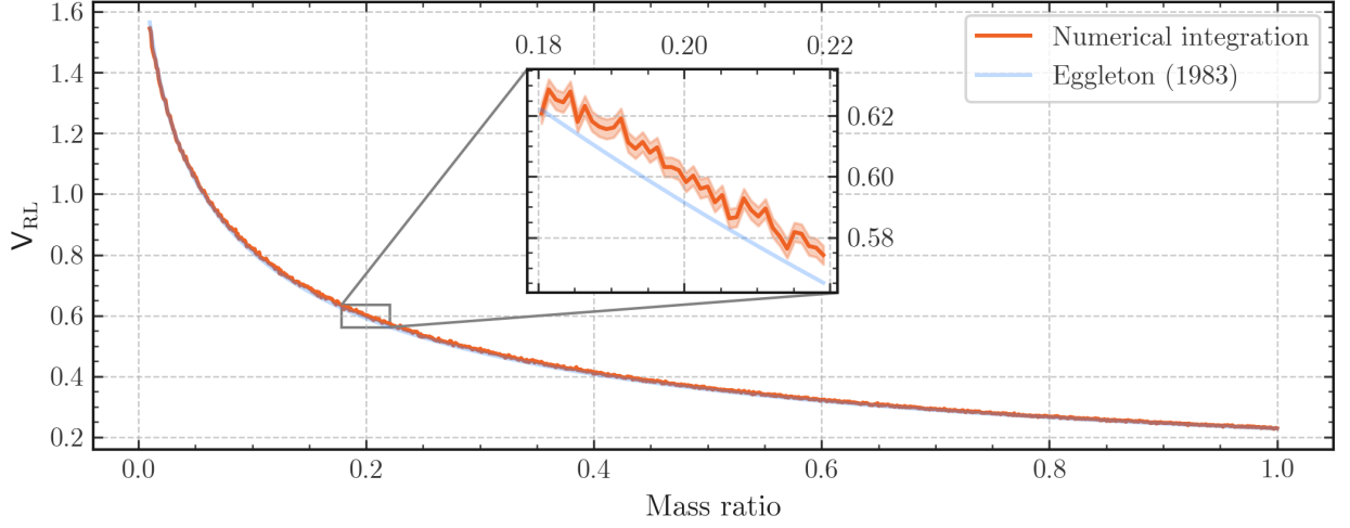
Figure 2.5: The volume of the Roche Lobe computed numerically through Monte-Carlo integration (orange) vs the volume assuming Equation 2.36 (blue). The Eggleton approximation fits well to the volume, with around 1 per cent error across the entire mass ratio range (truncated here to q \leq 1 ).
