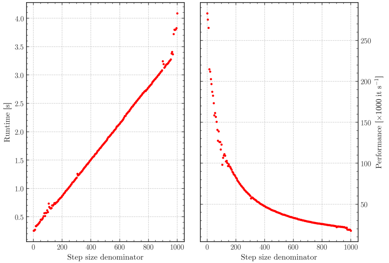
Figure 4.2: The effect of varying d_e in Equation 4.5 on the runtime, which is demonstrably \mathcal{O}(n) , and the performance of the algorithm. The input data to this algorithm were the LISA binary sample from Tang (2024) . The performance is shown in units of thousands of iterations per second.
