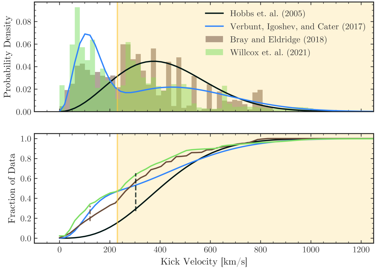
Figure 4.4: The PDF and CDF of the distributions using kicks from Hobbs et al. (2005) ; Verbunt et al. (2017) ; Bray & Eldridge (2018) ; Willcox et al. (2021) . Hobbs et al. (2005) has a closed-form expression, whereas the others are computed empirically, hence the Bray and Willcox CDFs are less smooth than that of Hobbs. The two dashed lines indicate where and how the K-S statistic is measured for the associated distribution. The yellow region indicates the region for which v_{\text{kick}} \geq v_{\text{TGRV}} , the transverse Galactic rotation velocity of the Sun, \sim 230 \text{ km s}^{-1} .
