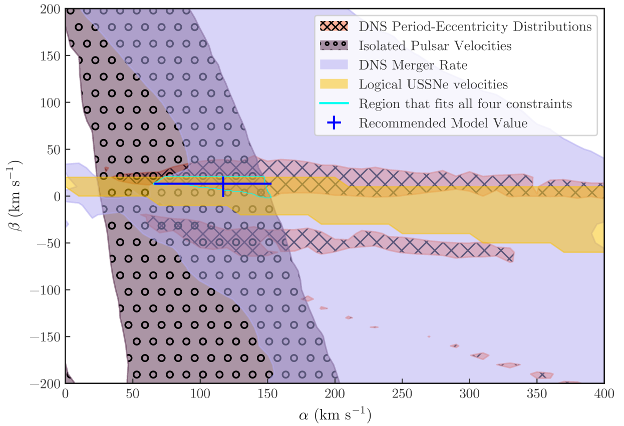
Figure 4.7: The four constraints we apply overlaid on our FINEGRID parameter space. The cyan region represents the region which fits all four parameters, and the blue cross represents the “center of mass” of this region.
