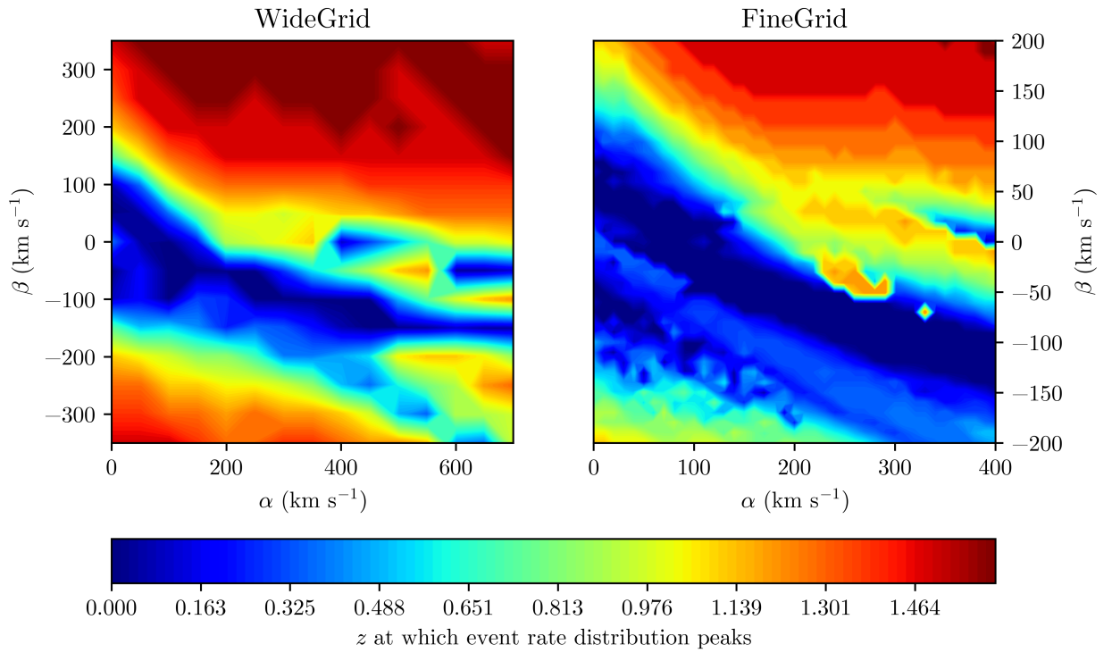
Figure 4.9: The peak of the event rate \mathcal{R}(t) as a function of \alpha and \beta . Varying these two parameters generally brings the peak closer to the present day ( z = 0 ). Absent a merger rate (or, more formally, assuming the merger rate is instantaneous and given by a Dirac-delta function), the SFRD peaks at z \sim 1.863 . The region surrounding the peak at \alpha = 330, \beta = -70 is shown in Figure 4.10.
