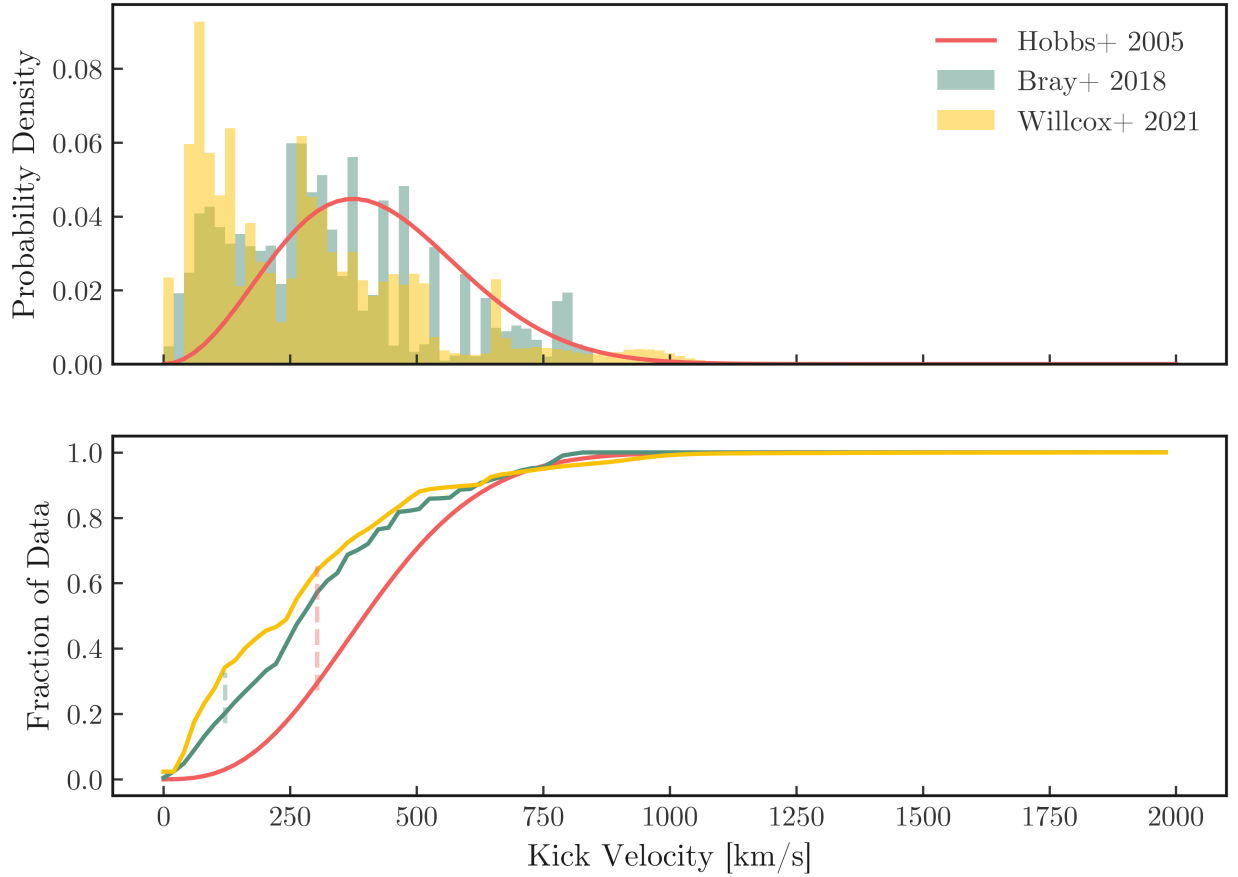
Figure 4.2: The PDF and CDF of the distributions using kicks from Hobbs et al. (2005) ; Bray & Eldridge (2018) ; Willcox et al. (2021) . Hobbs et al. (2005) has a closed-form expression, whereas the others are computed empirically, hence the Bray and Willcox CDFs are less smooth than that of Hobbs. The two dashed lines indicate where and how the K-S statistic is measured for the associated distribution.
