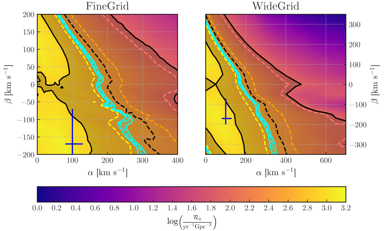
Figure 4.1: The merger rate as a function of kick parameters \alpha and \beta . The cyan contour is the theoretical merger rate as reported by Eldridge et al. (2019) . The black contour is the merger rate observed in LIGO-Virgo (2021) . The remaining contours are the merger rates reported in LIGO-Virgo-KAGRA (2021) (pink: BGP, yellow: MS, orange: PDB [ind], see LIGO-Virgo-KAGRA (2021) for an explanation of each model). Shaded regions represent uncertainties, and uncertainties are not reported for the LIGO-Virgo-KAGRA (2021) results as they would cover the entire plane. The blue cross is the fiducial value of \alpha and \beta from Bray & Eldridge (2018) . This value lies off the previous work’s contours as the rejuvenation age calculation has been improved in TUI in preparation for the next major BPASS release.
