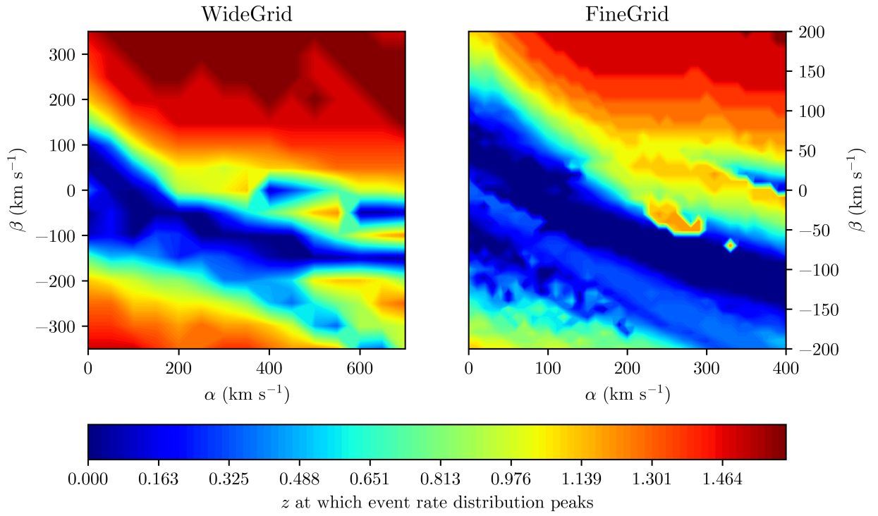
Figure 4.7: The peak of the event rate \mathcal{R}(t) as a function of \alpha and \beta . Varying these two parameters generally brings the peak closer to the present day ( z = 0 ). Absent a merger rate (or, more formally, assuming the merger rate is instantaneous and given by a Dirac-delta function), the SFRD peaks at z \sim 1.863 .
