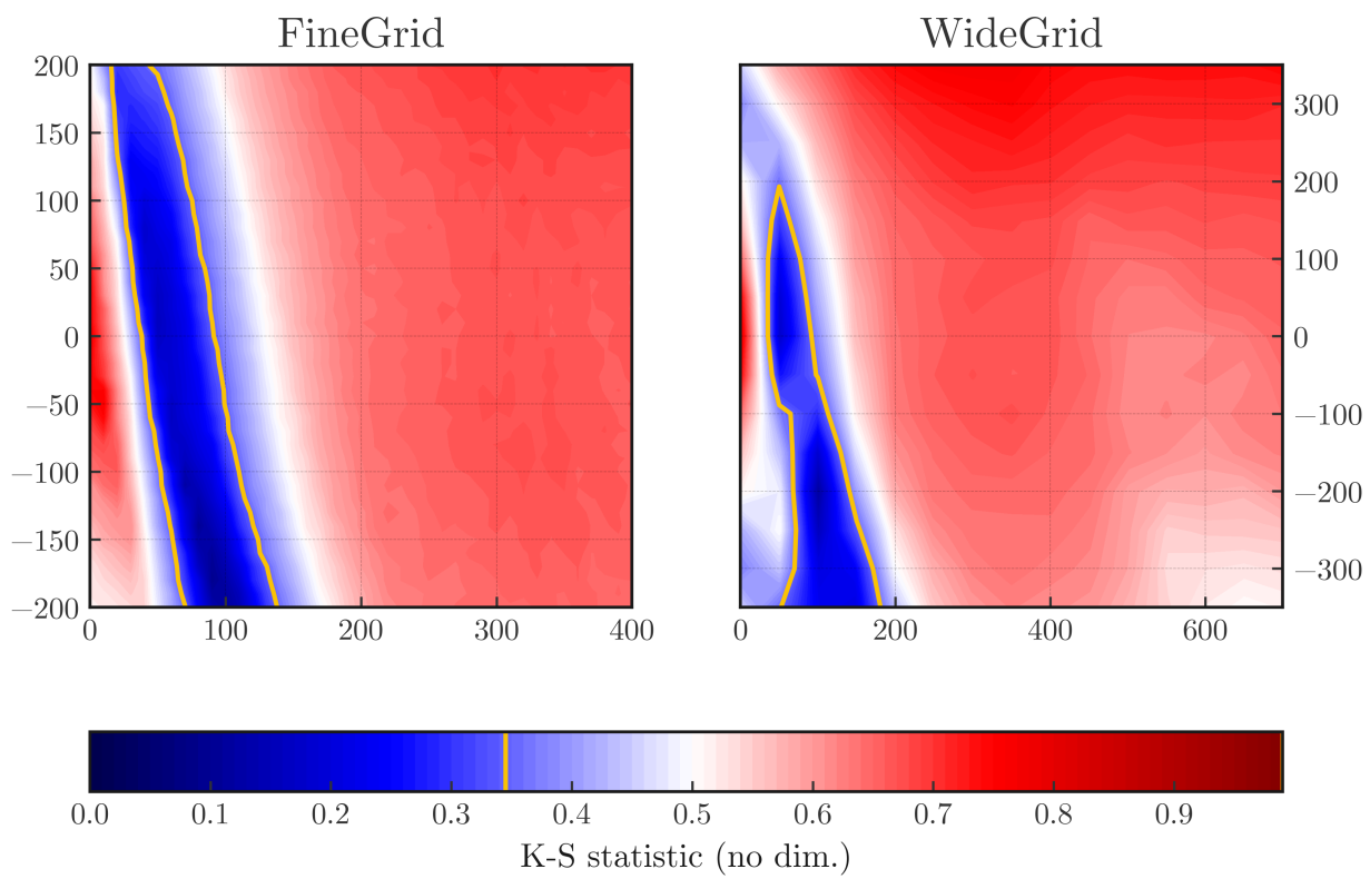
Figure 4.3: The K-S statistic for FINEGRID and WIDEGRID. The orange line denotes the K-S statistic for the Hobbs kick, which has a value of 0.34.
