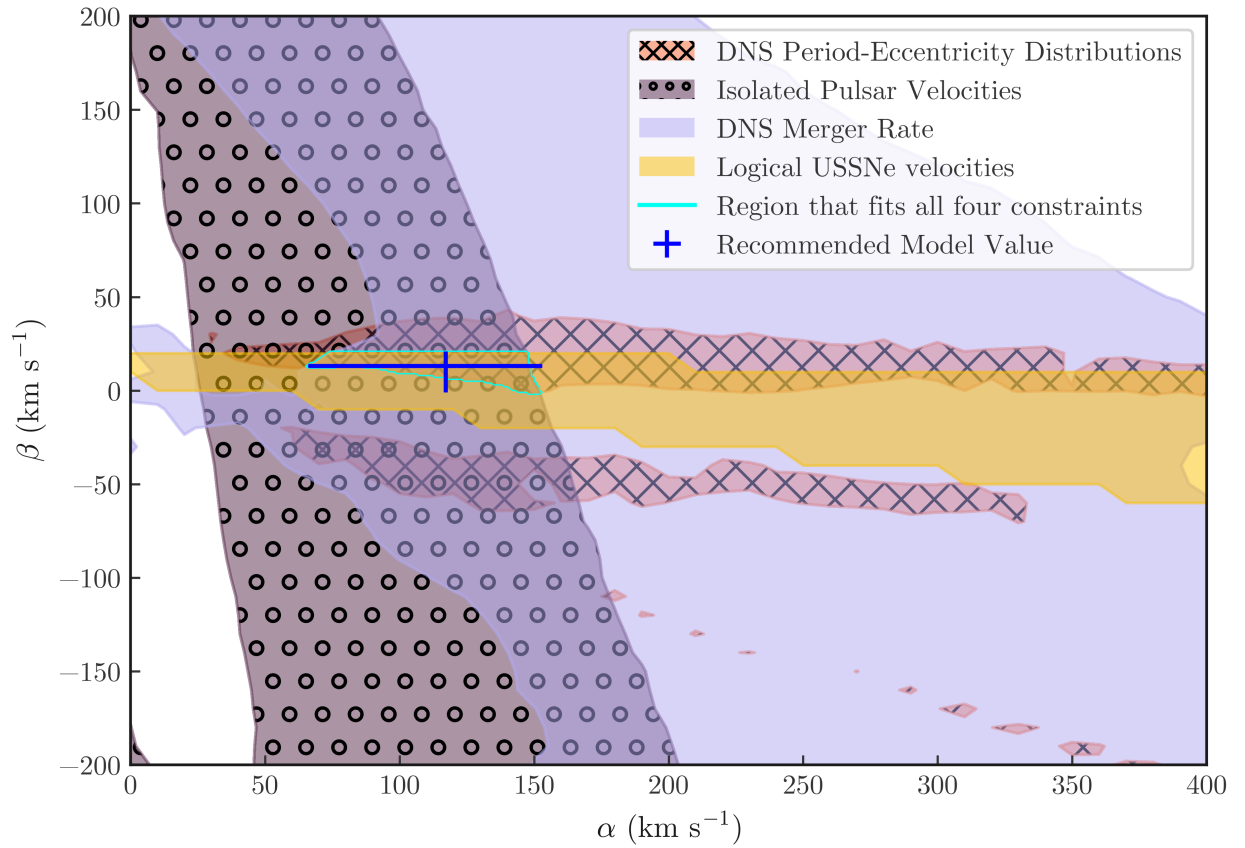
Figure 4.5: The four constraints we apply overlaid on our FINEGRID parameter space. The cyan region represents the region which fits all four parameters, and the blue cross represents the “center of mass” of this region.
