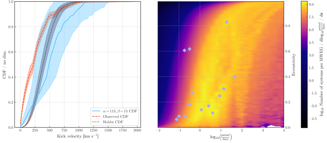
Figure 4.6: The CDF for a population of isolated pulsars (left) and the period-eccentricity distribution (right) for \alpha = 115 \text{ km s}^{-1}, \beta = 15 \text{ km s}^{-1} . The blue region on the CDF plot shows the uncertainty region for the reported value. The red region shows the uncertainty band on the Willcox et al. (2021) CDF, which was computed by sampling the PDF 10,000 times, taking 2,000 samples each time, and plotting the extent of the simulated distribution. The black band is the uncertainty on the Hobbs distribution, taking \sigma_{\text{max}} = 291 \text{ km s}^{-1} and \sigma_{\text{min}} = 239 \text{ km s}^{-1} from Verbunt et al. (2017).
