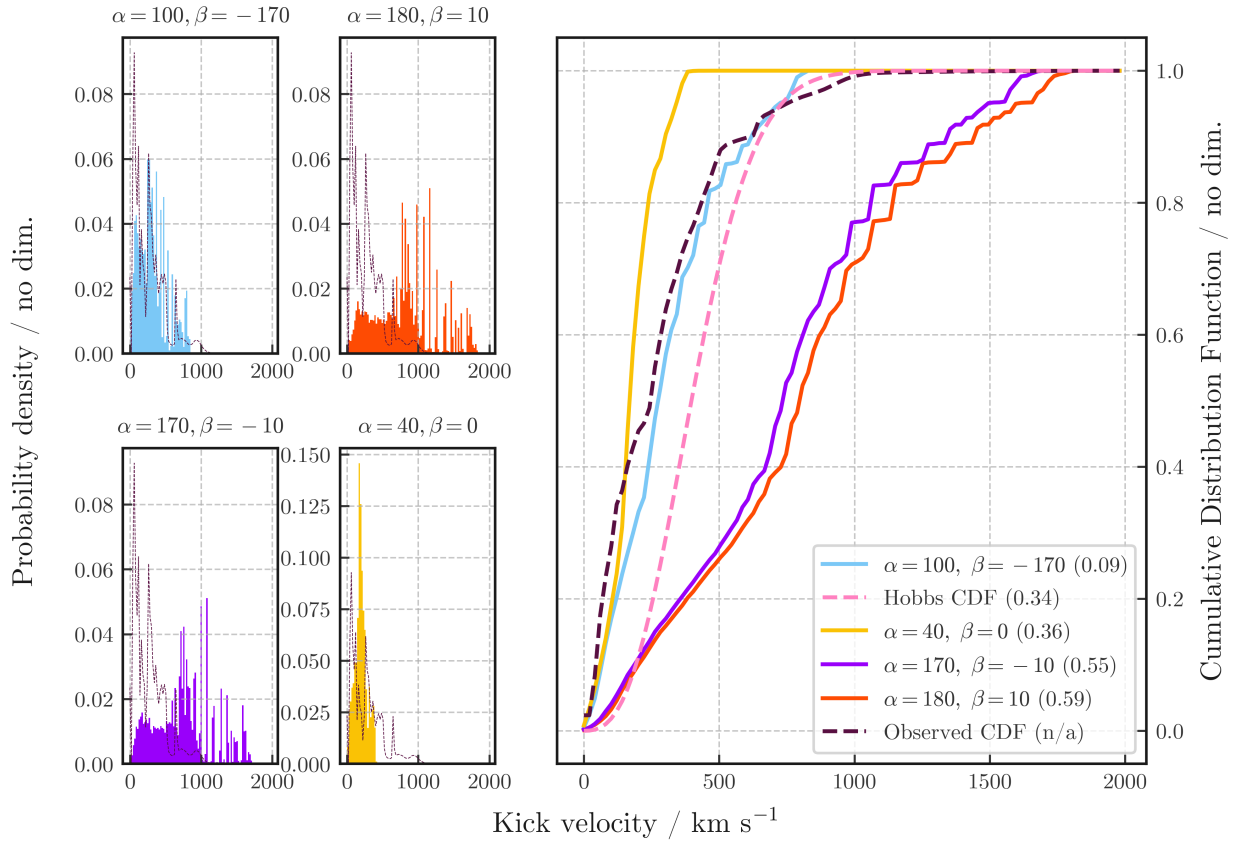
Figure 4.4: The PDFs and CDFs of four systems, alongside the Hobbs CDF and Willcox et al. (2021) CDF. The dashed line on the PDF plots is the PDF of the observed distribution from Willcox et al. (2021). On the right hand plot, the number in parentheses represents the K-S statistic for the distribution, measured relative to Willcox et al. (2021), which by definition has no K-S statistic.
