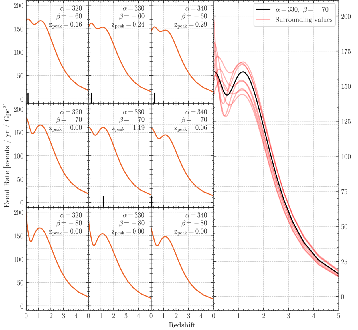
Figure 4.10: The event rate \mathcal{R}(z) for a region surrounding \alpha = 330, \beta = -70 on FINEGRID. This region corresponds to the “outlier” in ???. Shown on the left are the outlier bin in the center and its neighbours in both \alpha -space and \beta -space. The black line on each plot denotes the location in redshift of the event rate distribution peak. The right plot shows the outlier in black and its neighbours in faded red behind.
