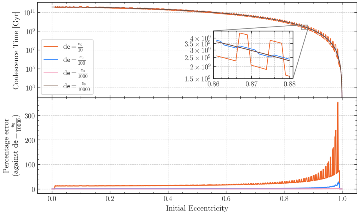
Figure 4.1: The effect of varying de in ?? on the coalescence time. Although hard to see, the pink line does oscillate above and below the brown line. This binary was assumed to have m_1 = m_2 = 1.44 M_\odot and a_0 = 1970.5 R_\odot (the mean separation of a sample of binaries with \alpha = 100 \text{ km s}^{-1} , \beta = -170 \text{ km s}^{-1} ).
