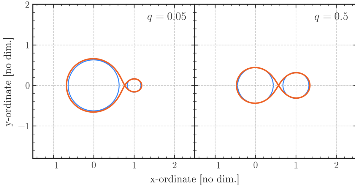
Figure 2.4: A schematic of the Roche lobe formula ???. Here, the exact solution to the Roche lobe formula \xi in ?? (orange) vs the fit provided by ? (blue). Although precise details of the Roche lobe, such as the apex of the teardrop at the point \xi , are lost, the volume is preserved to within 1 per cent accuracy over all mass ratios.
