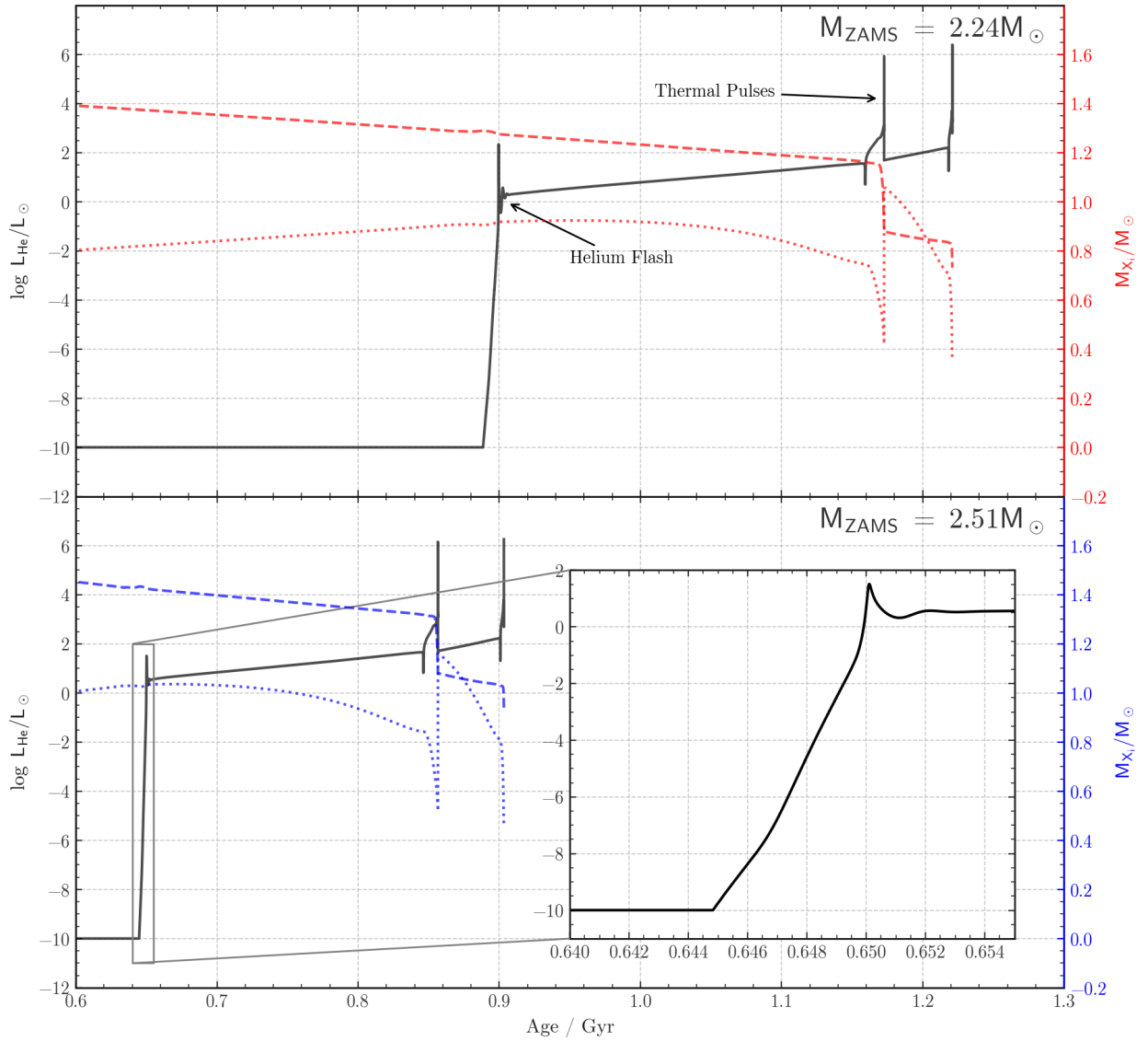
Figure 2.7: Two stars of a similar mass that undergo a helium flash and two thermal pulses. Shown in the inset is a zoomed-in helium flash that lasts \sim 7 Myr. Both stars undergo two thermal pulses before the code crashes due to the relative error in the calculation increasing too rapidly. The two stars could, in principle, undergo many more thermal pulses before their deaths.
