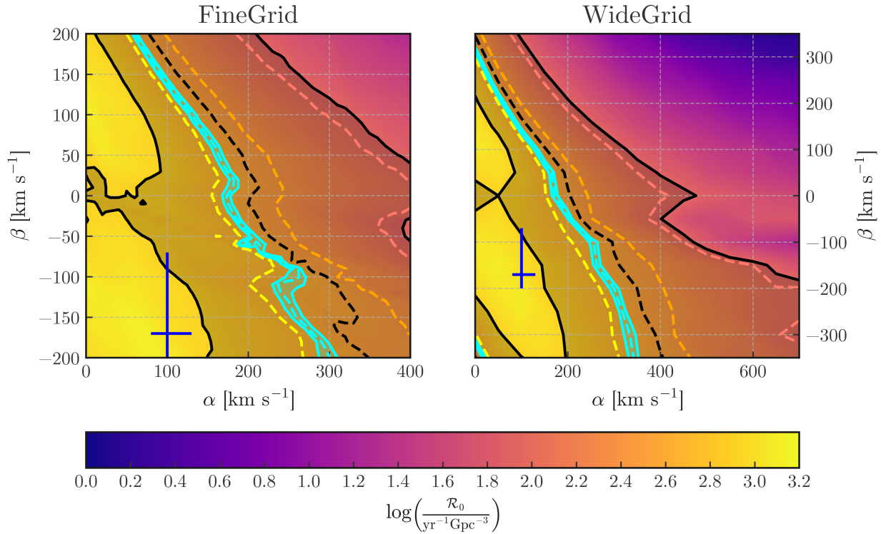
Figure 4.3: The merger rate as a function of kick parameters \alpha and \beta . The cyan contour is the theoretical merger rate as reported by ?. The black contour is the merger rate observed in ?. The remaining contours are the merger rates reported in ? (pink: BGP, yellow: MS, orange: PDB [ind], see ? for an explanation of each model). Shaded regions represent uncertainties, and uncertainties are not reported for the ? results as they would cover the entire plane. The blue cross is the fiducial value of \alpha and \beta from ?. This value lies off the previous work’s contours as the rejuvenation age calculation has been improved in TUI in preparation for the next major BPASS release.
