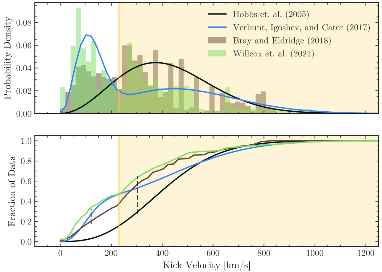
Figure 4.4: The PDF and CDF of the distributions using kicks from ???. ? has a closed-form expression, whereas the others are computed empirically, hence the Bray and Willcox CDFs are less smooth than that of Hobbs. The two dashed lines indicate where and how the K-S statistic is measured for the associated distribution. The yellow region indicates the region for which v_{\text{kick}} \geq v_{\text{TGRV}} , the transverse Galactic rotation velocity of the Sun, \sim 230 \text{ km s}^{-1} .
