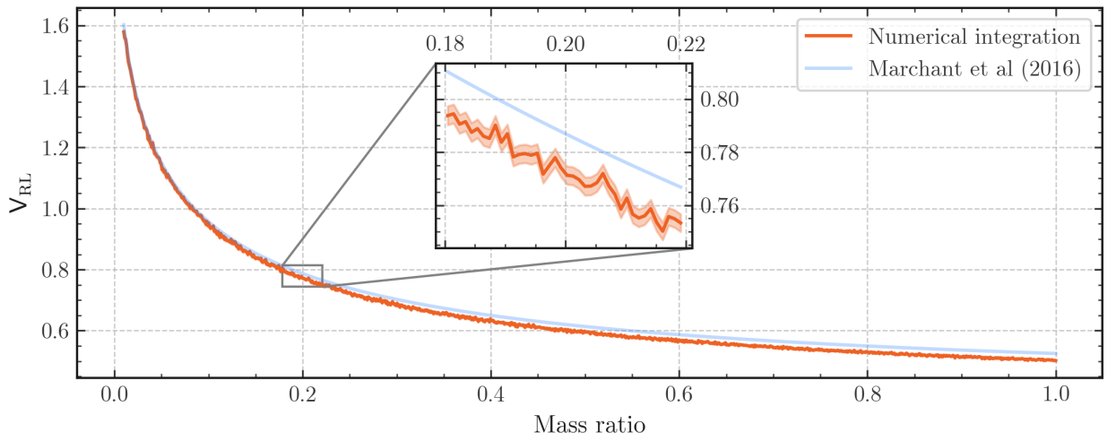
Figure 2.6: As for ??, but for the \mathcal{L}_2 point with formula given by ?? (?).
