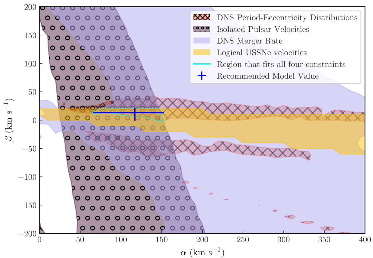
Figure 4.7: The four constraints we apply overlaid on our FINEGRID parameter space. The cyan region represents the region which fits all four parameters, and the blue cross represents the “center of mass” of this region.
