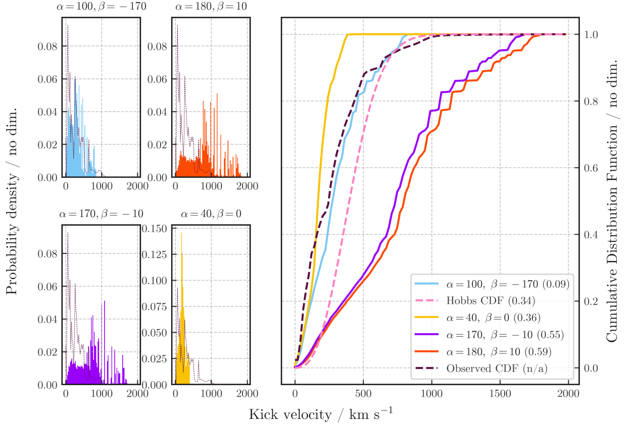
Figure 4.6: The PDFs and CDFs of four systems, alongside the Hobbs CDF and ? CDF. The dashed line on the PDF plots is the PDF of the observed distribution from ?. On the right hand plot, the number in parentheses represents the K-S statistic for the distribution, measured relative to ?, which by definition has no K-S statistic.
