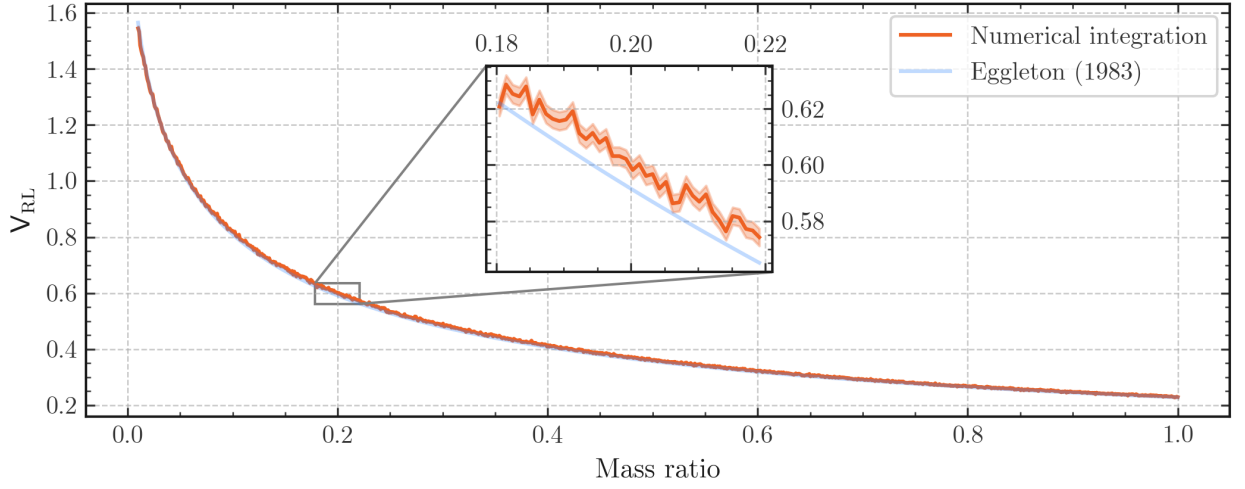
Figure 2.5: The volume of the Roche Lobe computed numerically through Monte-Carlo integration (orange) vs the volume assuming ?? (blue). The Eggleton approximation fits well to the volume, with around 1 per cent error across the entire mass ratio range (truncated here to q \leq 1 ).
