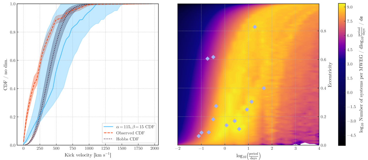
Figure 4.8: The CDF for a population of isolated pulsars (left) and the period-eccentricity distribution (right) for \alpha = 115 \text{ km s}^{-1}, \beta = 15 \text{ km s}^{-1} . The blue region on the CDF plot shows the uncertainty region for the reported value. The red region shows the uncertainty band on the \text{?} CDF, which was computed by sampling the PDF 10,000 times, taking 2,000 samples each time, and plotting the extent of the simulated distribution. The black band is the uncertainty on the Hobbs distribution, taking \sigma_{\text{max}} = 291 \text{ km s}^{-1} and \sigma_{\text{min}} = 239 \text{ km s}^{-1} from \text{?} .
