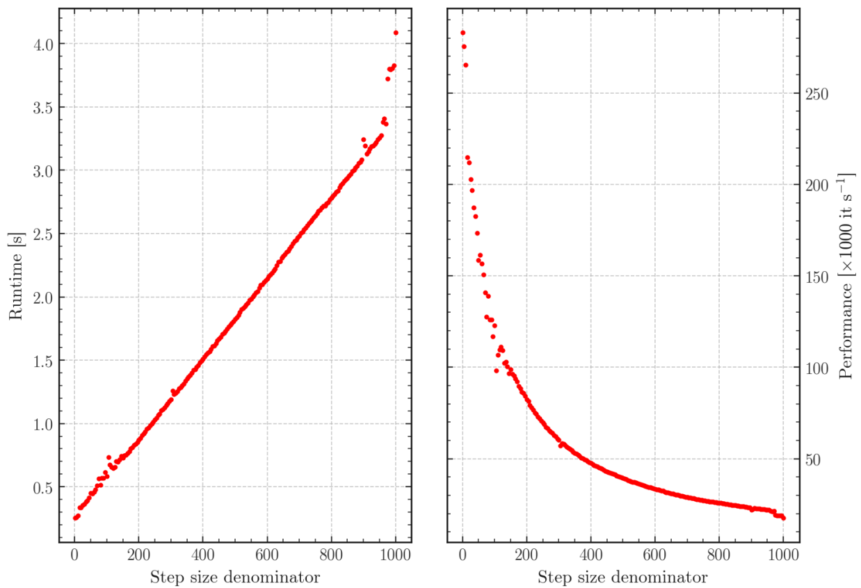
Figure 4.2: The effect of varying de in ?? on the runtime, which is demonstrably \mathcal{O}(n) , and the performance of the algorithm. The input data to this algorithm were the LISA binary sample from ?. The performance is shown in units of thousands of iterations per second.
