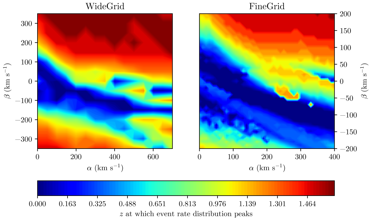
Figure 4.9: The peak of the event rate \mathcal{R}(t) as a function of \alpha and \beta . Varying these two parameters generally brings the peak closer to the present day ( z = 0 ). Absent a merger rate (or, more formally, assuming the merger rate is instantaneous and given by a Dirac-delta function), the SFRD peaks at z \sim 1.863 . The region surrounding the peak at \alpha = 330, \beta = -70 is shown in ??.
