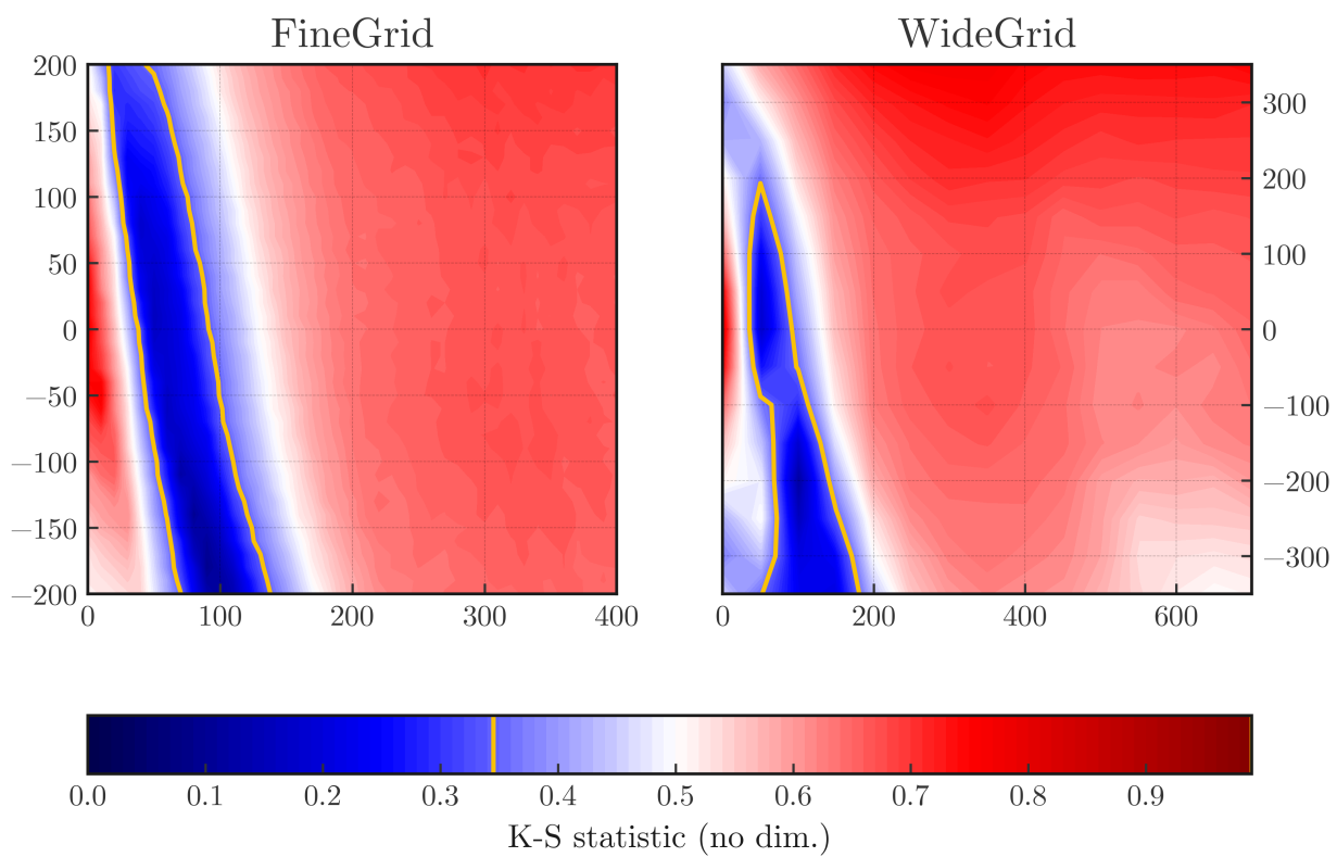
Figure 4.5: The K-S statistic for FINEGRID and WIDEGRID. The orange line denotes the K-S statistic for the Hobbs kick, which has a value of 0.34.
