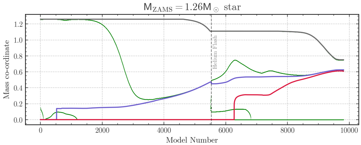
Figure 2.8: The helium flash (gray dashed line) shown on a Kippenhahn diagram. There is a slight discontinuity in the helium core mass (blue) due to a perfect match not existing in the 3 M_{\odot} reference model. The total mass is shown as the solid gray line, and the CO core mass is shown in red. The green lines show the boundaries of the convective regions of the star.
