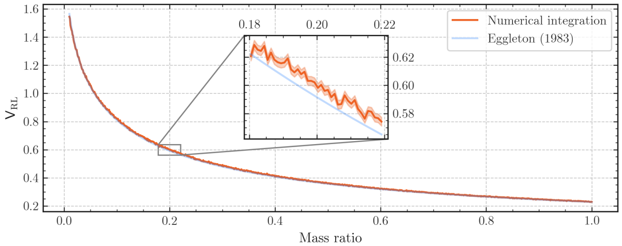
Figure 2.7: The volume of the Roche Lobe computed numerically through Monte-Carlo integration (orange) vs the volume assuming Equation 2.30 (blue). The Eggleton approximation fits well to the volume, with around 1 per cent error across the entire mass ratio range (truncated here to q \leq 1 ).
