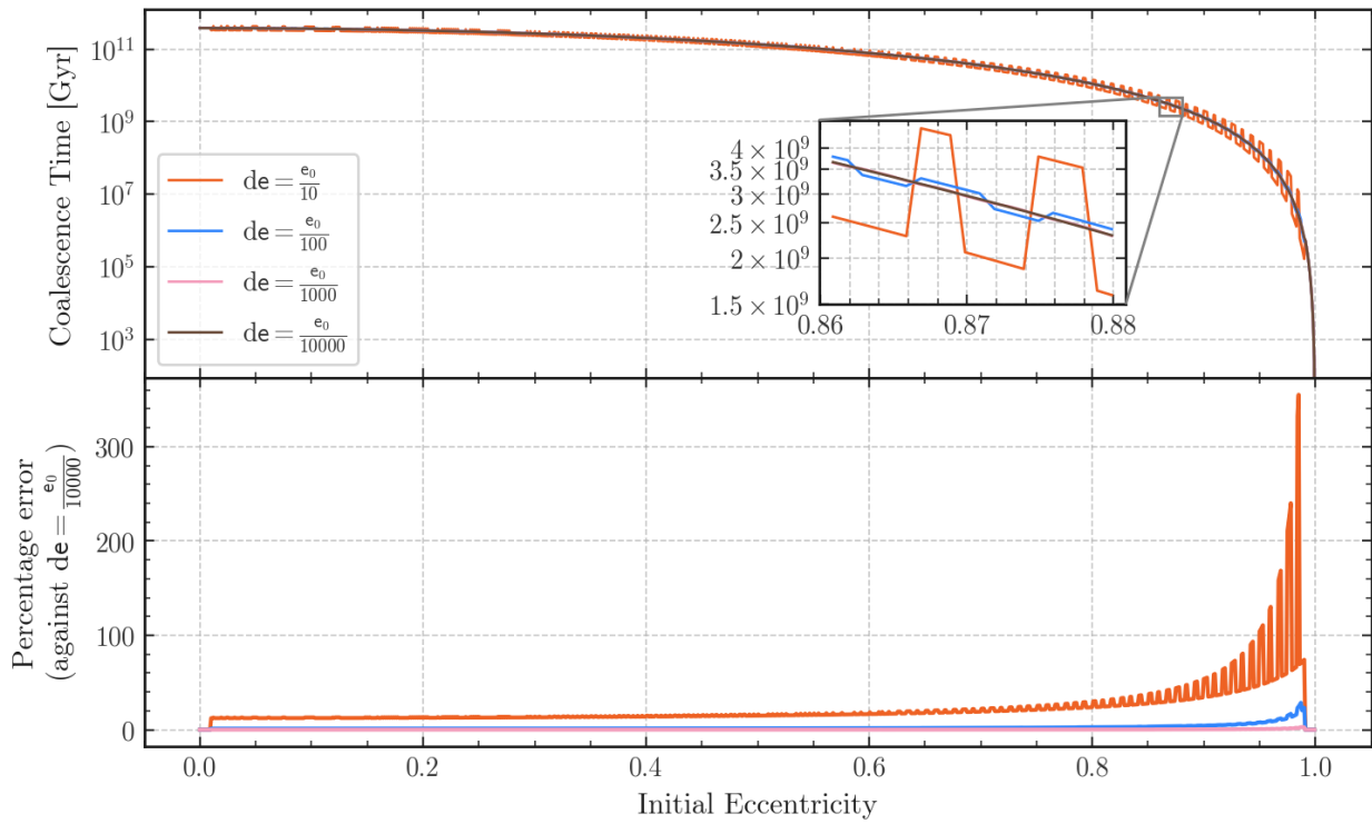
Figure 6.2: The effect of varying de in Equation 6.5 on the coalescence time. Although hard to see, the pink line does oscillate above and below the brown line. This binary was assumed to have m_1 = m_2 = 1.44 M_\odot and a_0 = 1970.5 R_\odot (the mean separation of a sample of binaries with \alpha = 100 \text{ km s}^{-1} , \beta = -170 \text{ km s}^{-1} ).
