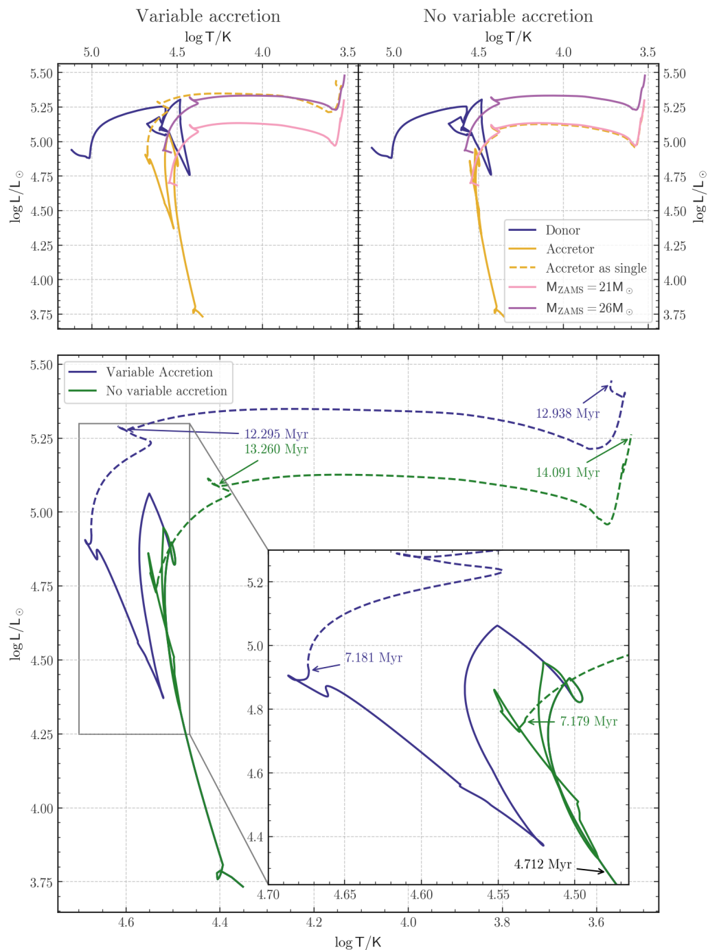
Figure 4.2: An HR diagram showing the evolution of our model both with (top left) and without (top right) the variable accretion prescription. The bottom panel shows only the evolution of the secondary. The point of divergence between the two models is shortly into the contact phase. The two dashed lines on the bottom top HR diagram represent models evolved as the final model of the binary secondary, as a single star. On the top HR diagrams, the pink and brown models are single stars evolved with ZAMS masses of 21 M_{\odot} and 26 M_{\odot} respectively.
