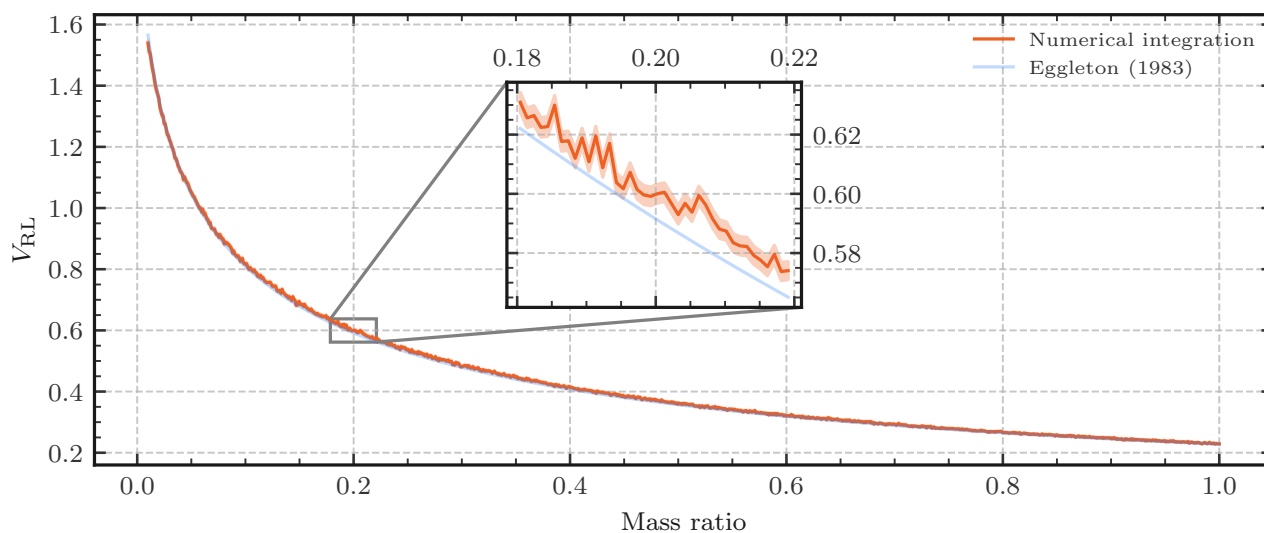
Figure 2.9: The volume of the Roche Lobe computed numerically through Monte-Carlo integration (orange) vs the volume assuming equation (2.13) (blue). The Eggleton approximation fits well to the volume, with around 1 per cent error across the entire mass ratio range (truncated here to q \leq 1 ).
