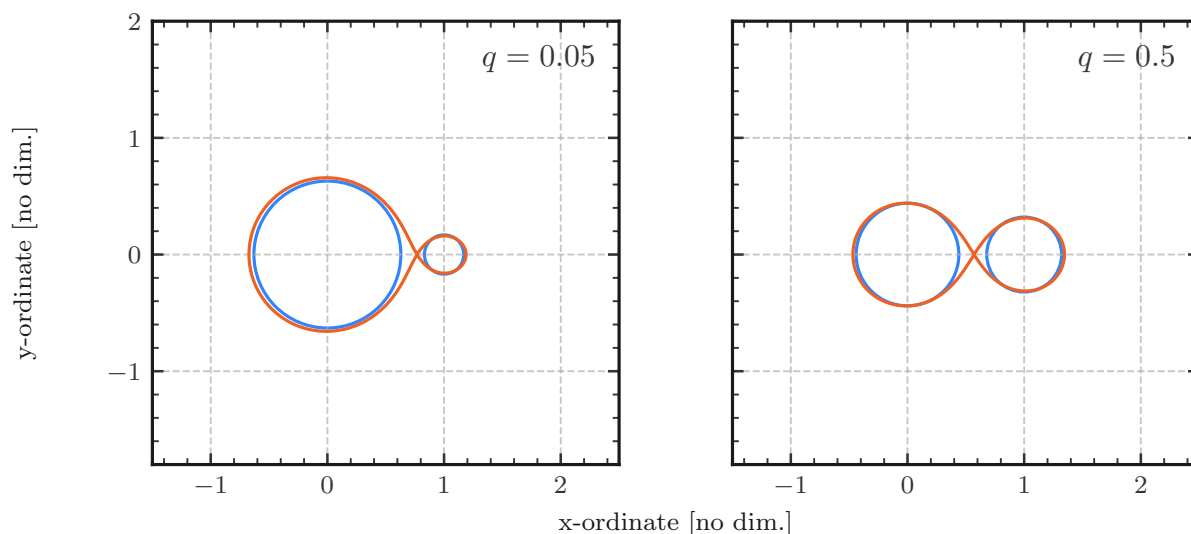
Figure 2.8: A schematic of the Roche lobe formula equation (2.13). Here, the exact solution to the Roche lobe formula \xi in equation (2.12) (orange) vs the fit provided by Eggleton (1983) (blue). Although precise details of the Roche lobe, such as the apex of the teardrop at the point \xi , are lost, the volume is preserved to within 1 per cent accuracy over all mass ratios.
