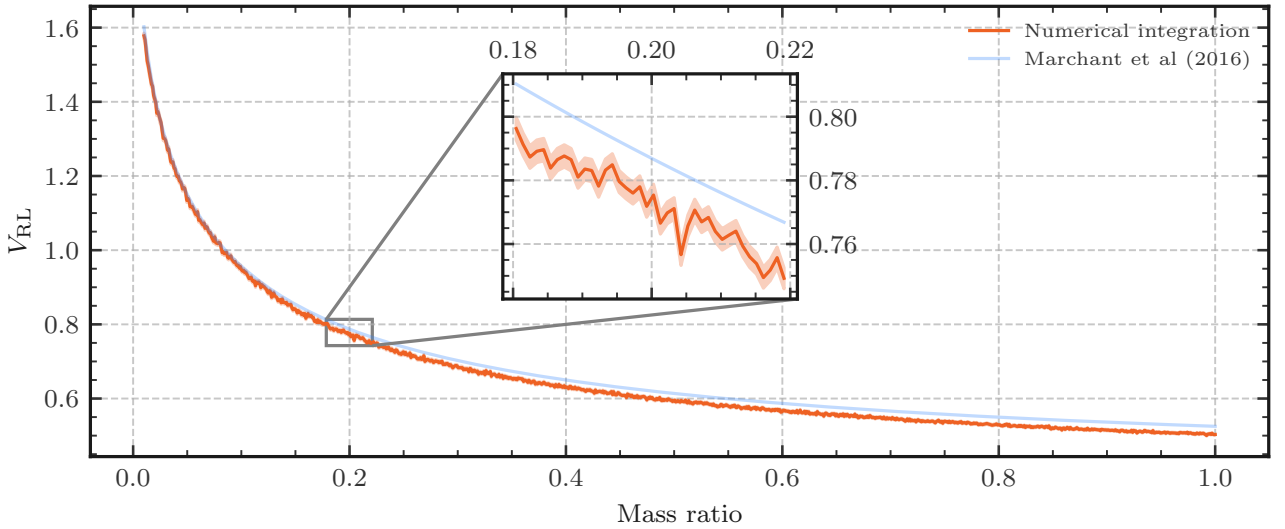
Figure 2.10: As for figure 2.9, but for the \mathcal{L}_2 point with formula given by equation (2.14) (Marchant et al., 2016).
