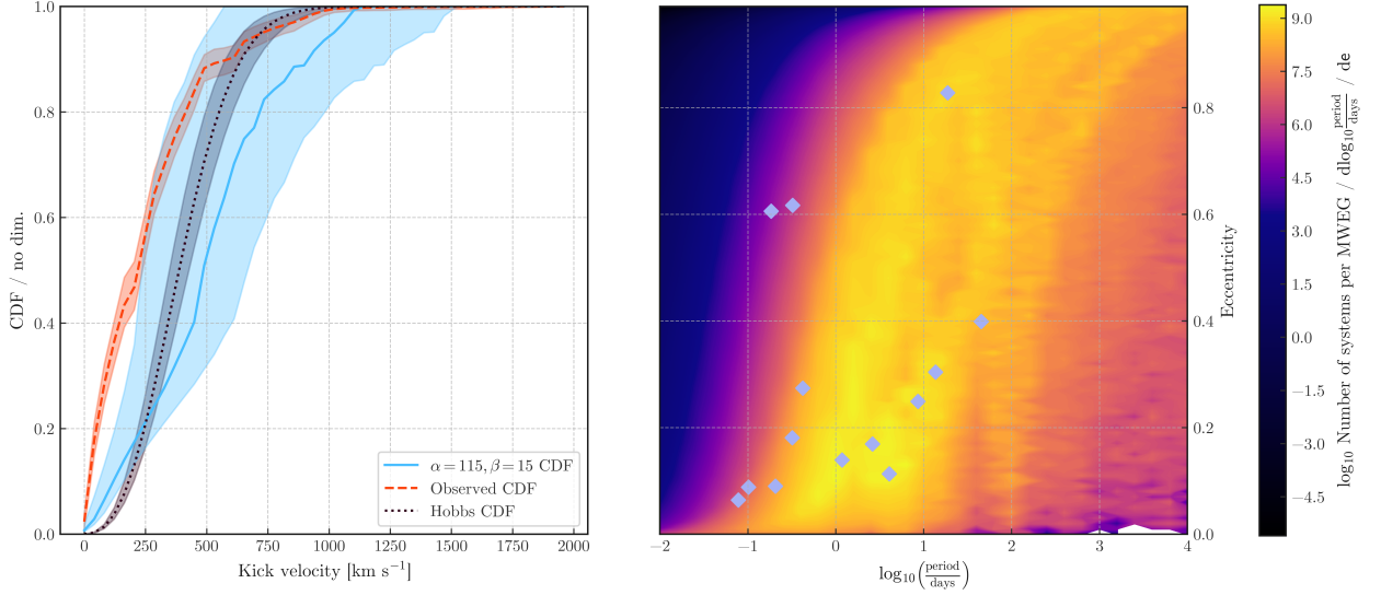
Figure 4.9: The CDF for a population of isolated pulsars (left) and the period-eccentricity distribution (right) for \alpha = 115 \text{ km s}^{-1}, \beta = 15 \text{ km s}^{-1} . The blue region on the CDF plot shows the uncertainty region for the reported value. The red region shows the uncertainty band on the Willcox et al. (2021) CDF, which was computed by sampling the PDF 10,000 times, taking 2,000 samples each time, and plotting the extent of the simulated distribution. The black band is the uncertainty on the Hobbs distribution, taking \sigma_{\text{max}} = 291 \text{ km s}^{-1} and \sigma_{\text{min}} = 239 \text{ km s}^{-1} from Verbunt et al. (2017) .
