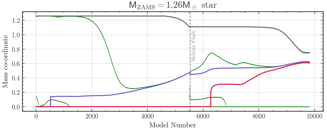
Figure 2.8: The helium flash (gray dashed line) shown on a Kippenhahn diagram. There is a slight discontinuity in the helium core mass (blue) due to a perfect match not existing in the 3M_{\odot} reference model. The total mass is shown as the solid gray line, and the CO core mass is shown in red. The green lines show the boundaries of the convective regions of the star.
