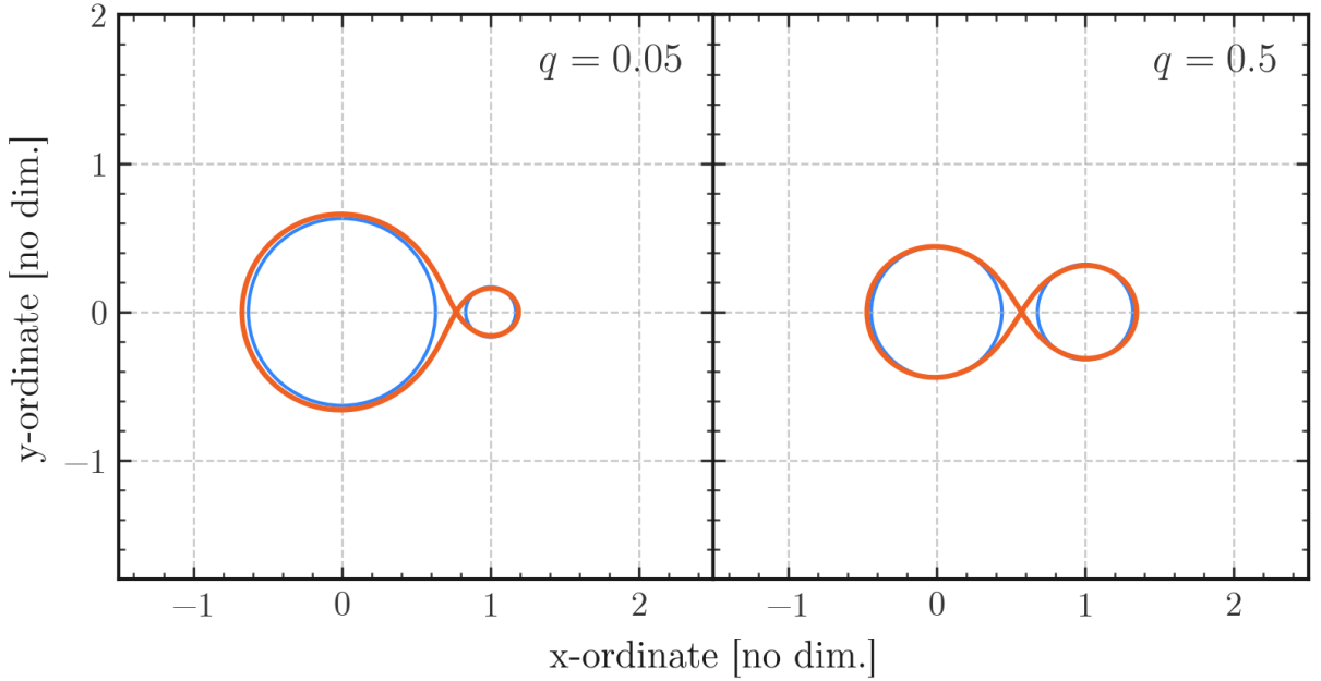
Figure 2.4: A schematic of the Roche lobe formula Equation 2.44. Here, the exact solution to the Roche lobe formula \xi in Equation 2.43 (orange) vs the fit provided by Eggleton (1983) (blue). Although precise details of the Roche lobe, such as the apex of the teardrop at the point \xi , are lost, the volume is preserved to within 1 per cent accuracy over all mass ratios.
