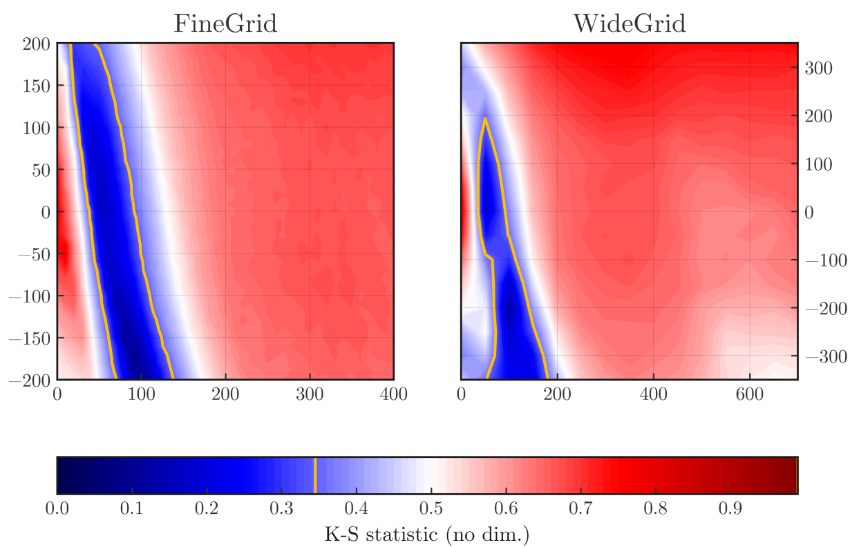
Figure 4.6: The K-S statistic for FINEGRID and WIDEGRID. The orange line denotes the K-S statistic for the Hobbs kick, which has a value of 0.34.
