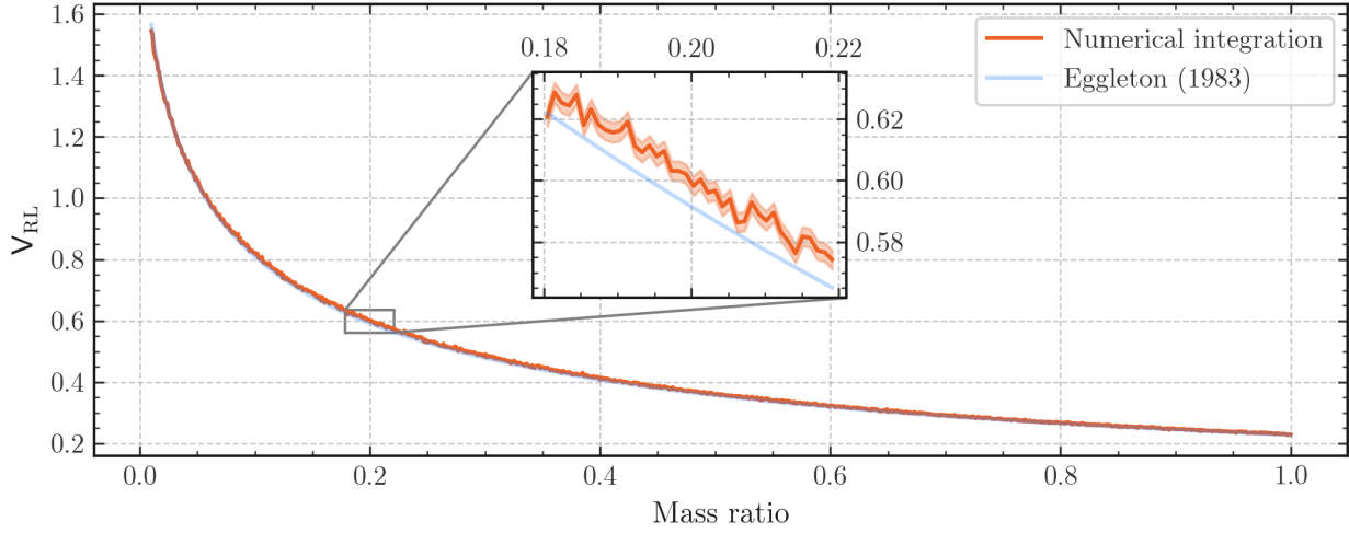
Figure 2.5: The volume of the Roche Lobe computed numerically through Monte-Carlo integration (orange) vs the volume assuming Equation 2.44 (blue). The Eggleton approximation fits well to the volume, with around 1 per cent error across the entire mass ratio range (truncated here to q \leq 1 ).
