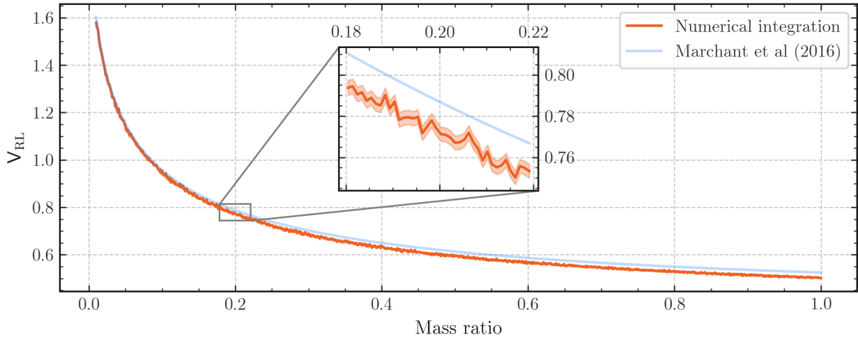
Figure 2.6: As for Figure 2.5, but for the \mathcal{L}_2 point with formula given by Equation 2.45 (Marchant et al., 2016).
