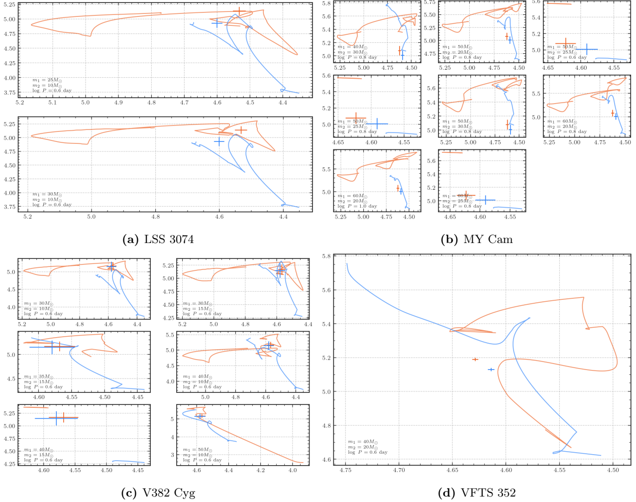
Figure 3.4: Detailed models of the close contact binaries found in subsection 3.1.2. Not shown are SMC 108086 and TU Mus, which both only have matches outside of the coarse grid. Also not shown is a match for MY Cam, which has a primary which is more massive than the grid.
