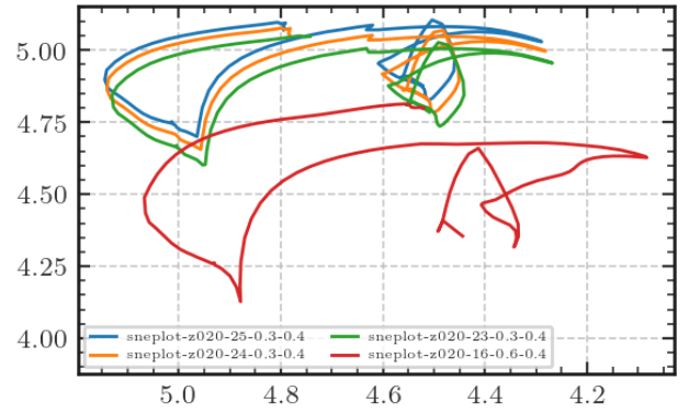
TU Mus matches according to HOKI
