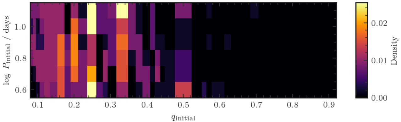
Figure 5.1: The density of systems which undergo helium-rich mass transfer across our grid. There is effectively a cutoff point at q_{\text{initial}} = 0.5 where systems above this mass ratio undergo helium-rich mass transfer significantly more rarely than systems below this.
