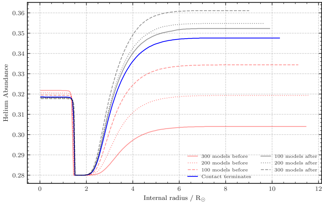
Accretor chemical composition near contact termination
