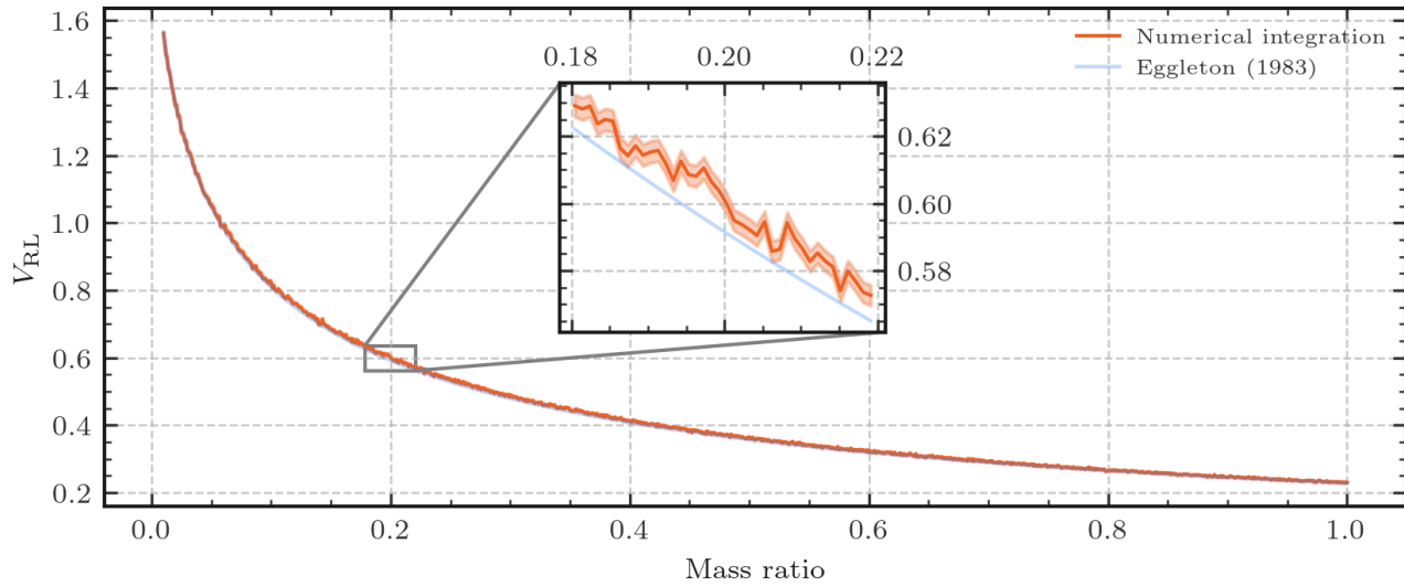
Figure 2.9: The volume of the Roche Lobe computed numerically through Monte-Carlo integration (orange) vs the volume assuming Equation 2.31 (blue). The Eggleton approximation fits well to the volume, with around 1 per cent error across the entire mass ratio range (truncated here to q \leq 1 ).
