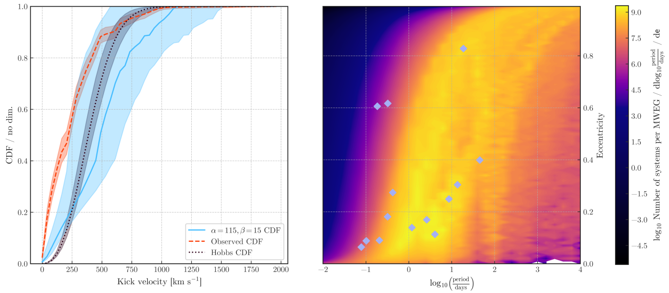
Figure 6.11: The CDF for a population of isolated pulsars (left) and the period-eccentricity distribution (right) for \alpha = 115 \text{ km s}^{-1} , \beta = 15 \text{ km s}^{-1} . The blue region on the CDF plot shows the uncertainty region for the reported value. The red region shows the uncertainty band on the Willcox et al. (2021) CDF, which was computed by sampling the PDF 10,000 times, taking 2,000 samples each time, and plotting the extent of the simulated distribution. The black band is the uncertainty on the Hobbs distribution, taking \sigma_{\text{max}} = 291 \text{ km s}^{-1} and \sigma_{\text{min}} = 239 \text{ km s}^{-1} from Verbunt et al. (2017).
