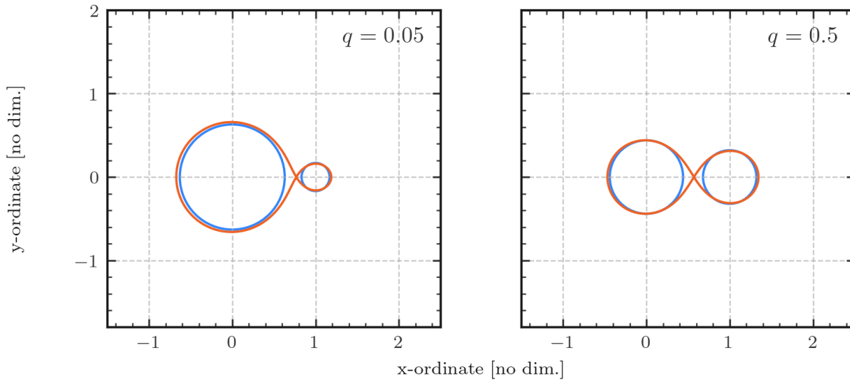
Figure 2.8: A schematic of the Roche lobe formula Equation 2.31. Here, the exact solution to the Roche lobe formula \xi in Equation 2.30 (orange) vs the fit provided by Eggleton (1983) (blue). Although precise details of the Roche lobe, such as the apex of the teardrop at the point \xi , are lost, the volume is preserved to within 1 per cent accuracy over all mass ratios.
