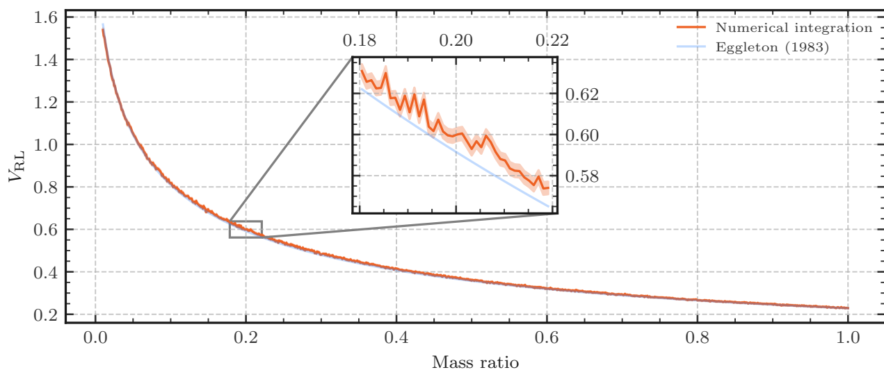
Figure 2.9: The volume of the Roche Lobe computed numerically through Monte-Carlo integration (orange) vs the volume assuming equation (2.21) (blue). The Eggleton approximation fits well to the volume, with around 1 per cent error across the entire mass ratio range (truncated here to q \leq 1 ).
