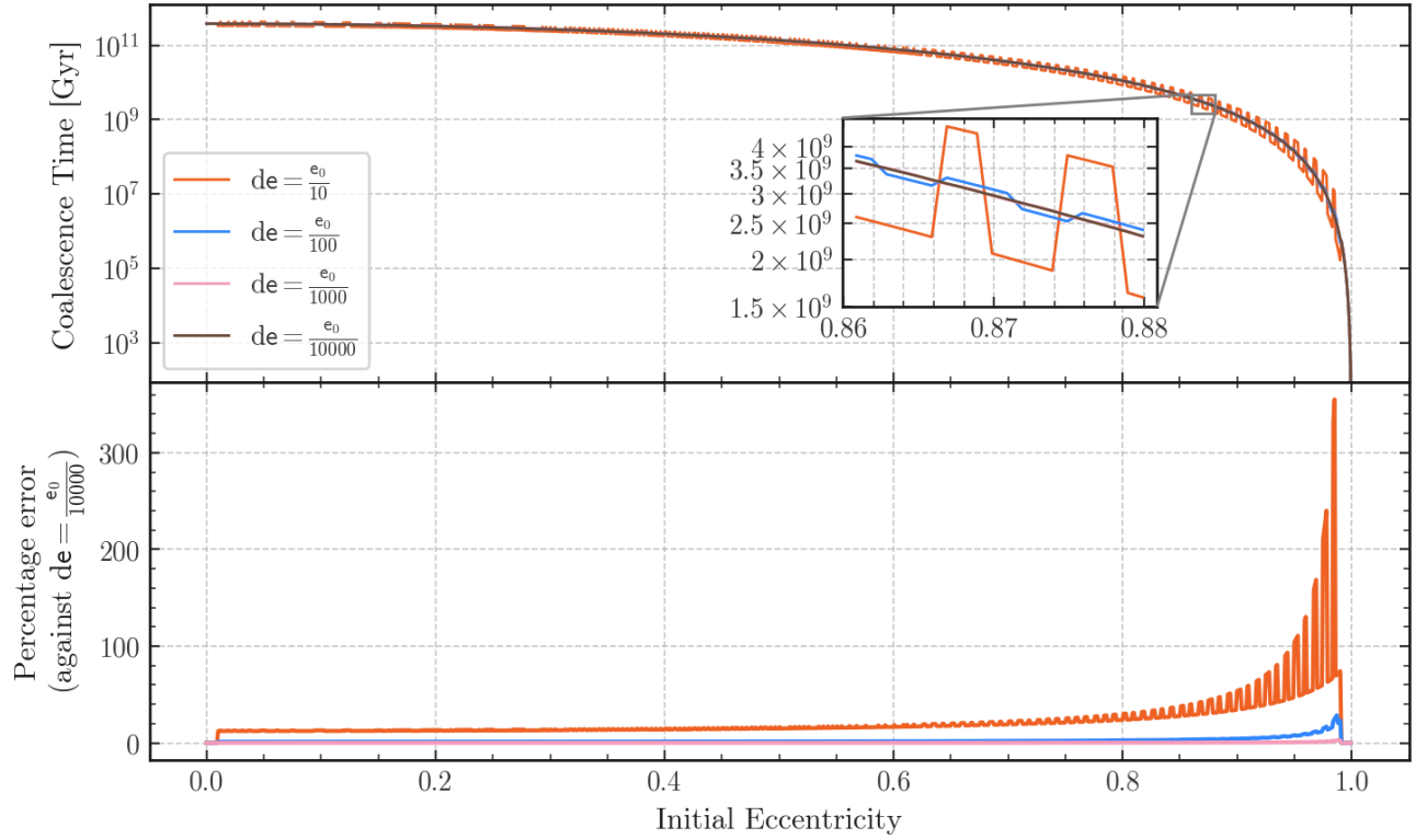
Figure 6.2: The effect of varying de in equation (6.5) on the coalescence time. Although hard to see, the pink line does oscillate above and below the brown line. This binary was assumed to have m_1 = m_2 = 1.44 M_\odot and a_0 = 1970.5 R_\odot (the mean separation of a sample of binaries with \alpha = 100 \text{ km s}^{-1} , \beta = -170 \text{ km s}^{-1} ).
