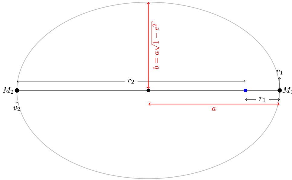
Figure 2.6: A schematic of a simple binary star system with eccentricity e . The centre of mass (barycentre) is shown as a blue dot. Here, M_1 is the heavier star, which orbits at a smaller distance r_1 to the barycentre by Kepler's first and Newton's second laws. The elliptical orbital trajectory is shown in grey. Figure adapted from Richards (2021).
