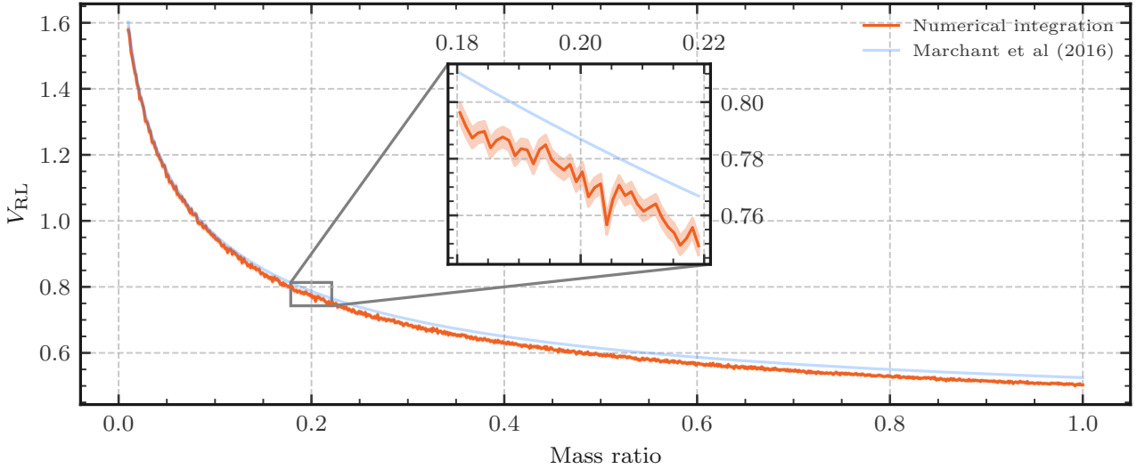
Figure 2.10: As for figure 2.9, but for the \mathcal{L}_2 point with formula given by equation (2.22) (Marchant et al., 2016).
