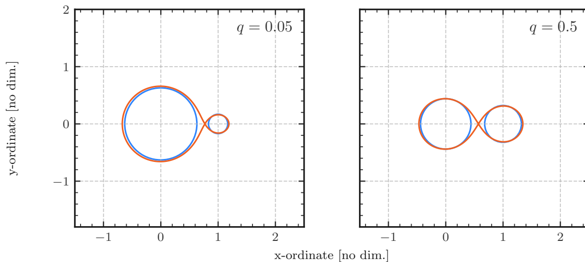
Figure 2.8: A schematic of the Roche lobe formula equation (2.21). Here, the exact solution to the Roche lobe formula \xi in equation (2.20) (orange) vs the fit provided by Eggleton (1983) (blue). Although precise details of the Roche lobe, such as the apex of the teardrop at the point \xi , are lost, the volume is preserved to within 1 per cent accuracy over all mass ratios.
