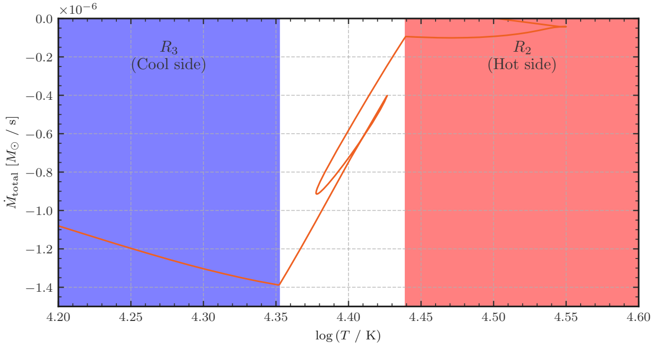
Figure 2.11: An illustration of the bi-stability jump at \log T \approx 4.4 . This illustration was computed for a 21 M_\odot star. Shown in blue is the cool side of the bistability jump, where R_3 (equation (2.28)) is the interpolation, and shown in red is the hot side, where R_2 (equation (2.27)) is the interpolation.
