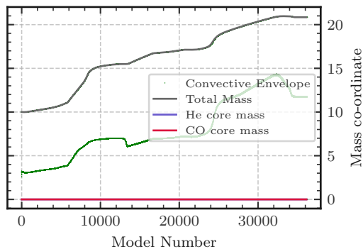
M_{\text{ZAMS}} = 10.0 M_{\odot} star
