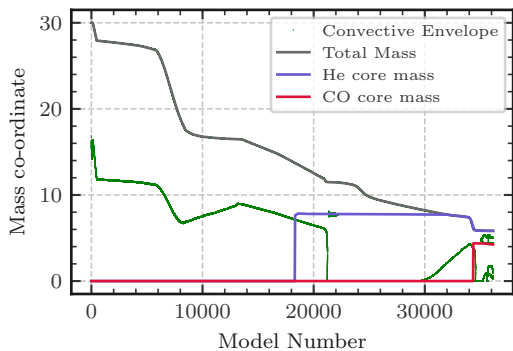
M_{\text{ZAMS}} = 30.0 M_{\odot} star
