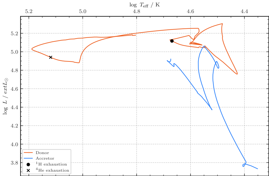
M_{\text{ZAMS}} = 30.0 M_{\odot} star
