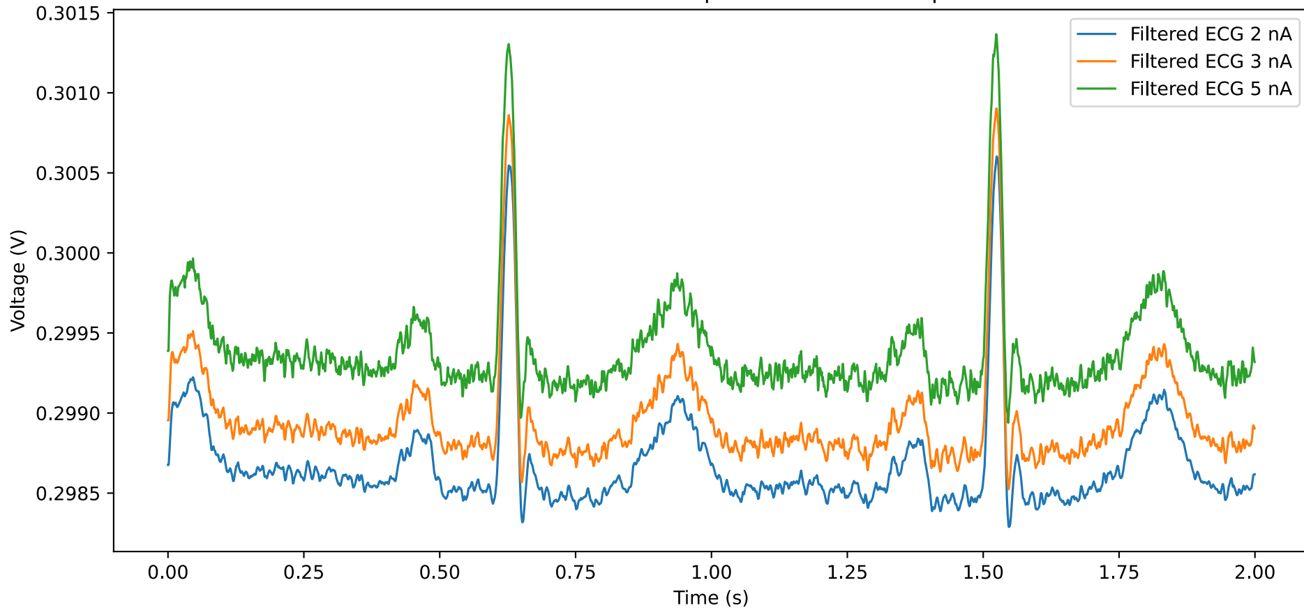
ECG Time-Domain Comparison: Filtered Outputs
