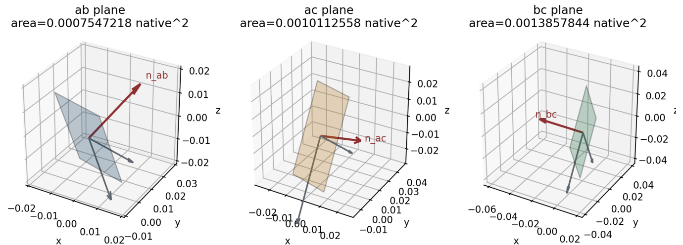
Figure 4. The three central face planes, with exact source areas and normals, provide the dimensional geometric reference for the response construction.
