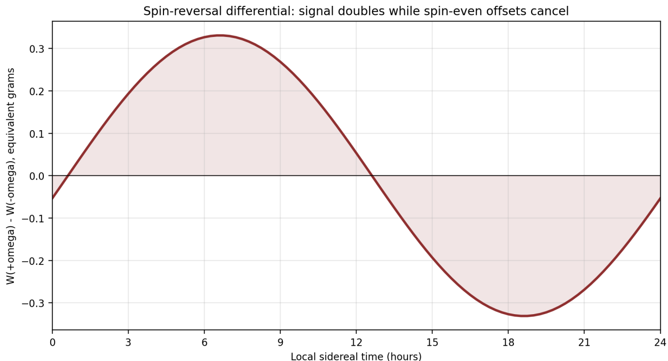
Figure 10. Full spin-reversal difference. The desired spin-odd waveform doubles relative to a single run.
