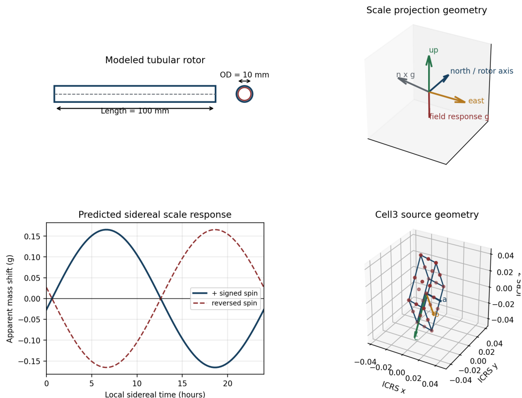
Figure 1. Title composite. The tube dimensions, Cell3 source geometry, local scale projection, and sidereal waveform are generated from the supplied numerical ledger and the derived fixed-laboratory transformation.
