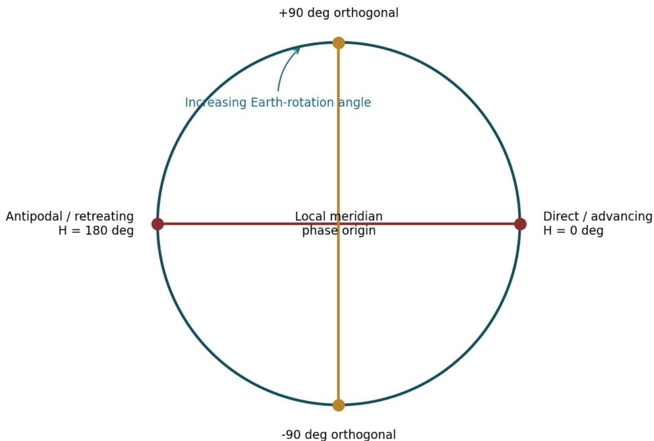
Figure 10. Direct, antipodal, and orthogonal event geometry.
