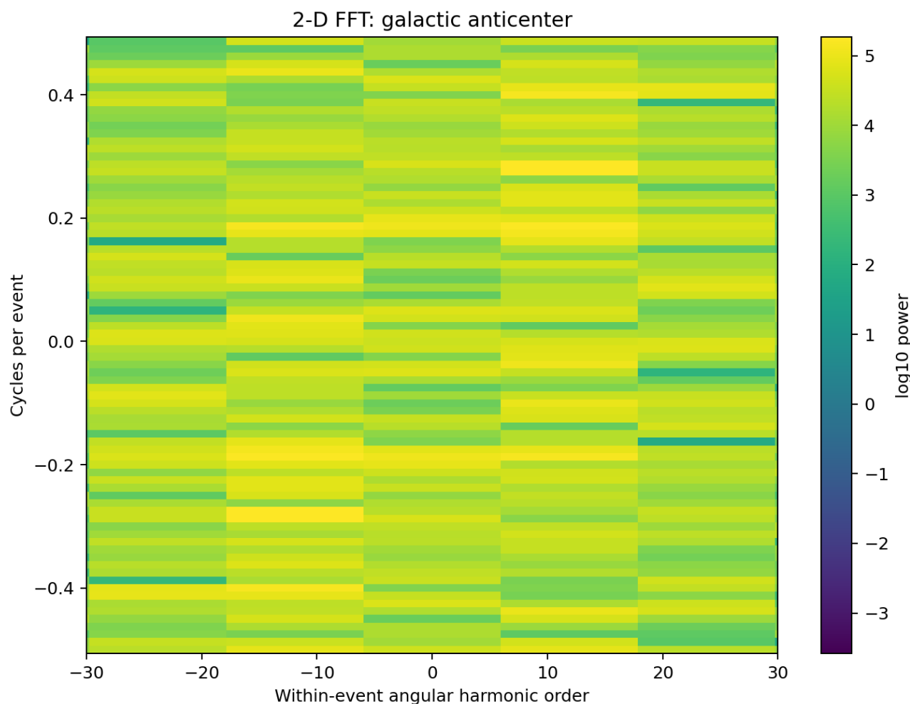
Figure 30. Two-dimensional FFT of a crossing-profile matrix.
