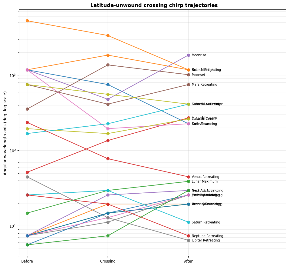
Figure 24. Angular-wavelength chirp atlas.
