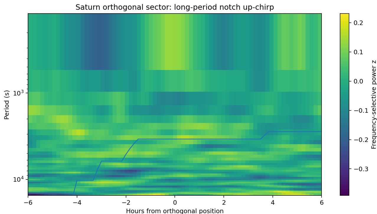
Figure 28. Saturn orthogonal-sector chirp.
