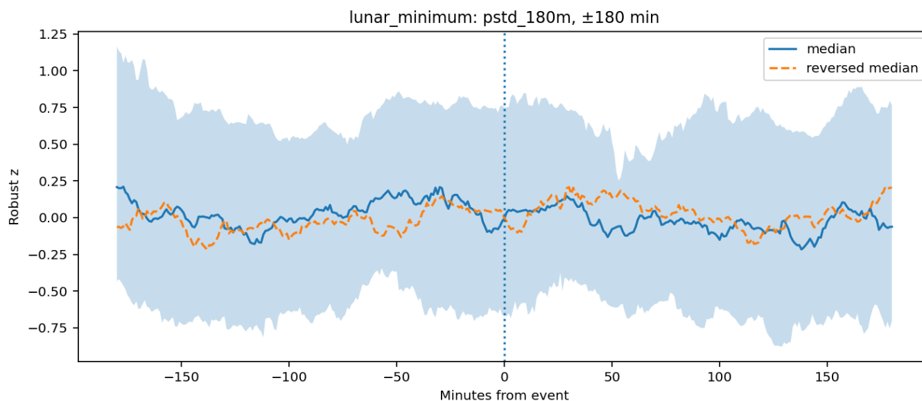
Figure 17. Lunar lower-culmination palindrome.
