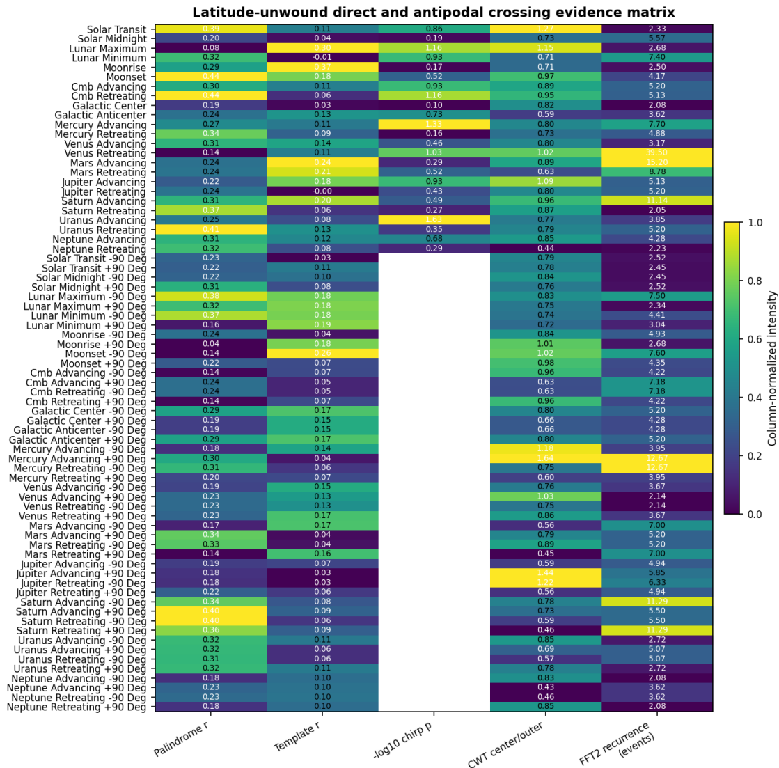
Figure 14. Consolidated direct and antipodal crossing evidence.
