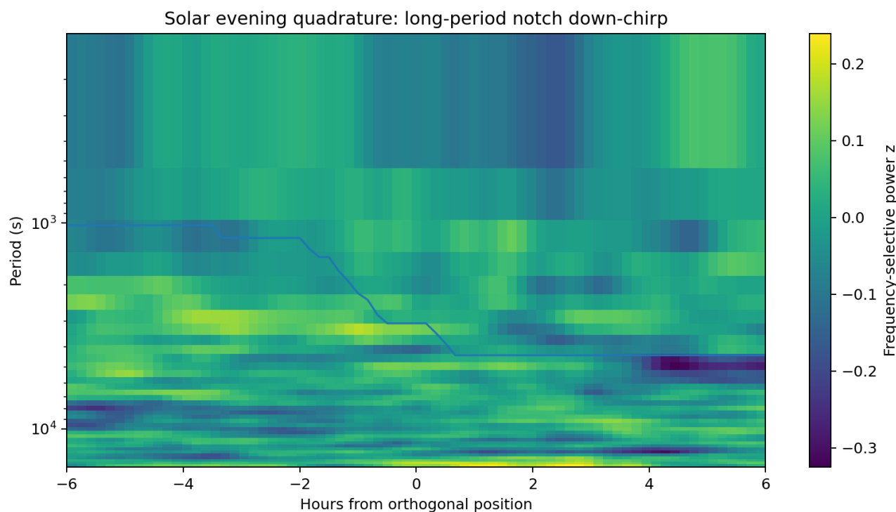
Figure 27. Solar evening orthogonal chirp.
