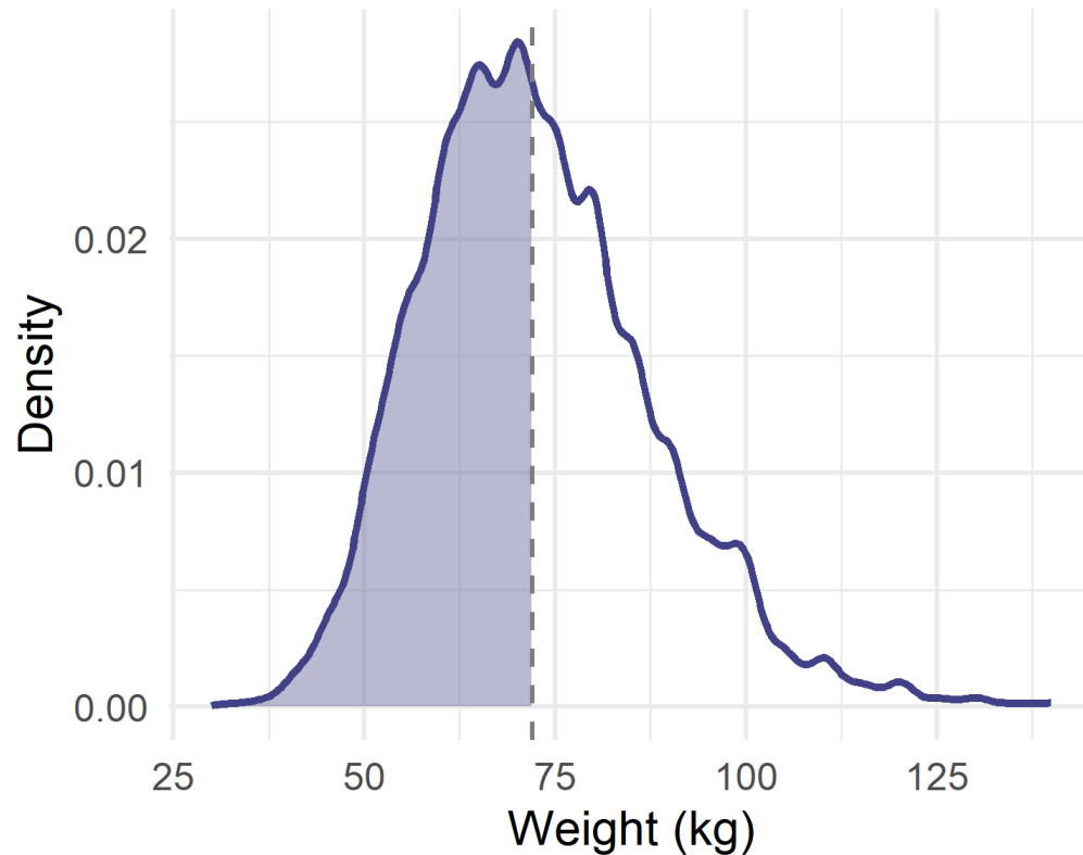
PDF — the area up to the cut
