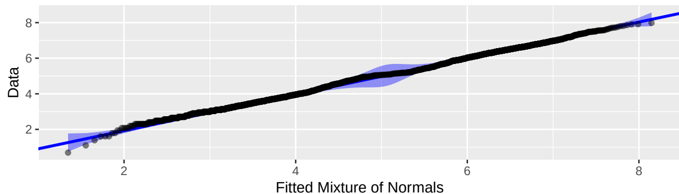
QQ-Plot
