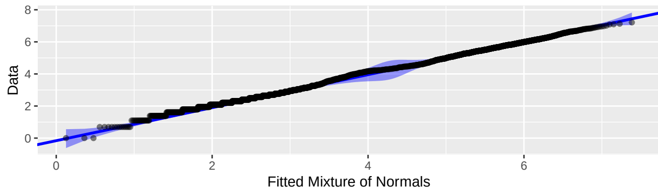
QQ-Plot
