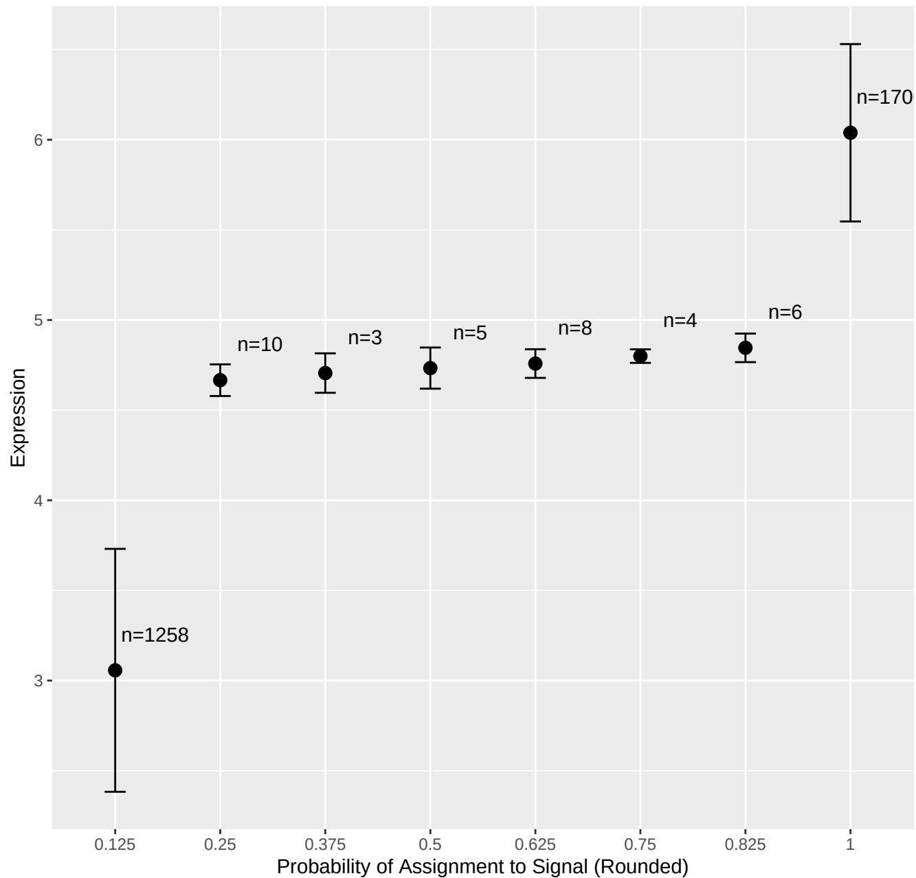
Stripchart of Average Expression ( \pm SD) Across All Genes in Each Category
