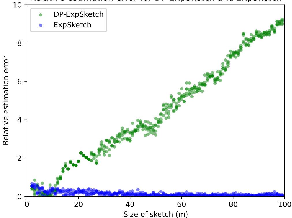
Relative estimation error for DP-ExpSketch and ExpSketch
