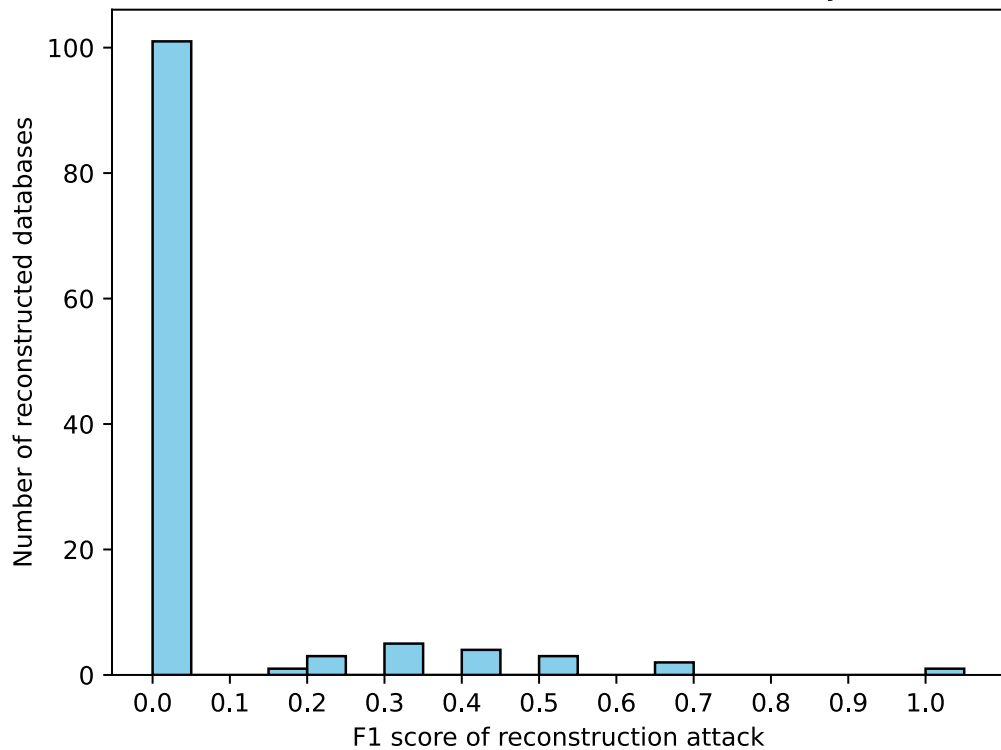
Plot of reconstruction attack accuracy
