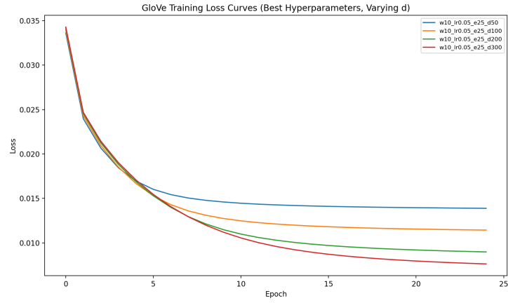
Figure 1.2: Loss curves for best hyperparameters across embedding dimensions
