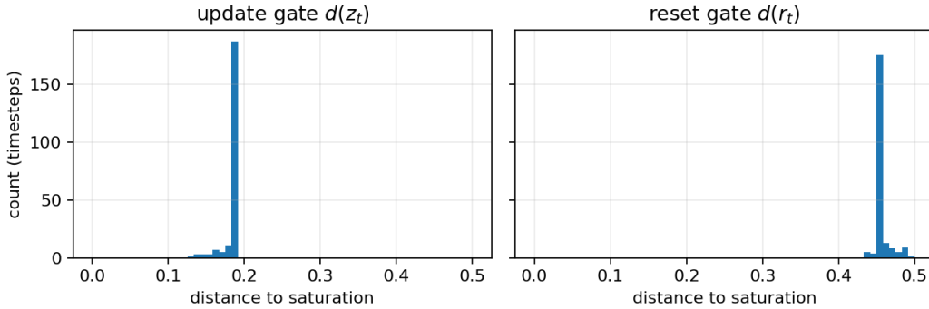
Figure 5: A4 GRU gate saturation-distance histograms.
