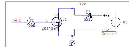
Solenoid and Driver Circuit
