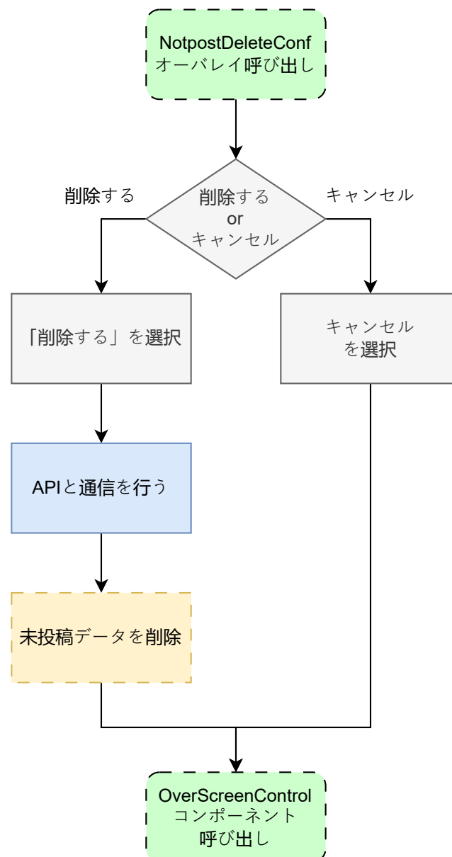
図 9: notpost_delete_conf.dart の状態遷移図
