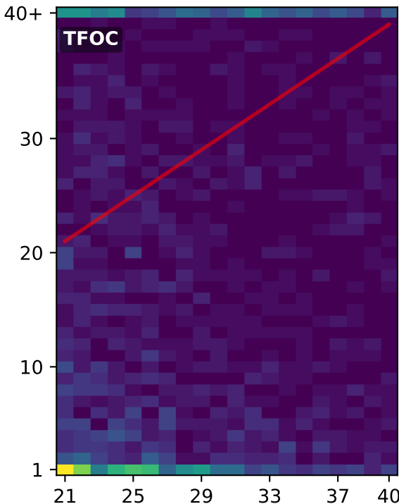
FSCD-LVIS
