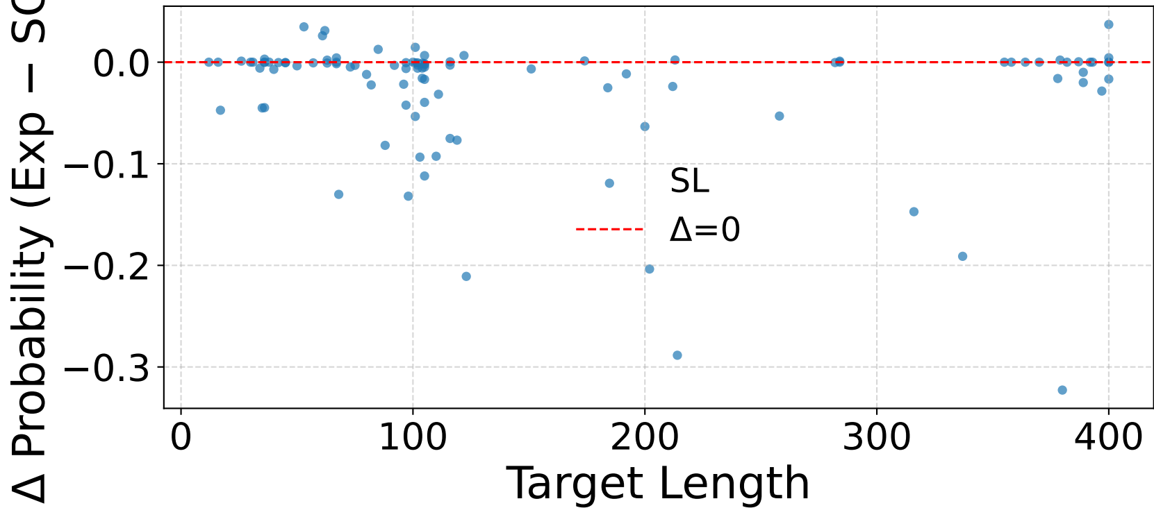
\Delta Probability vs Length — SL
