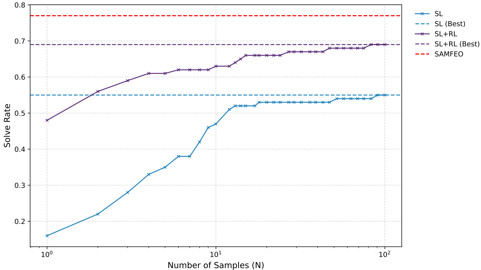
Best-of-N Solve Rate
