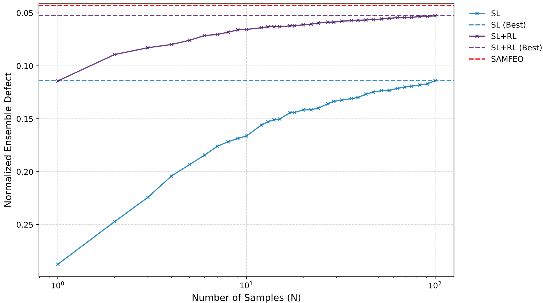
Best-of-N Normalized Ensemble Defect
