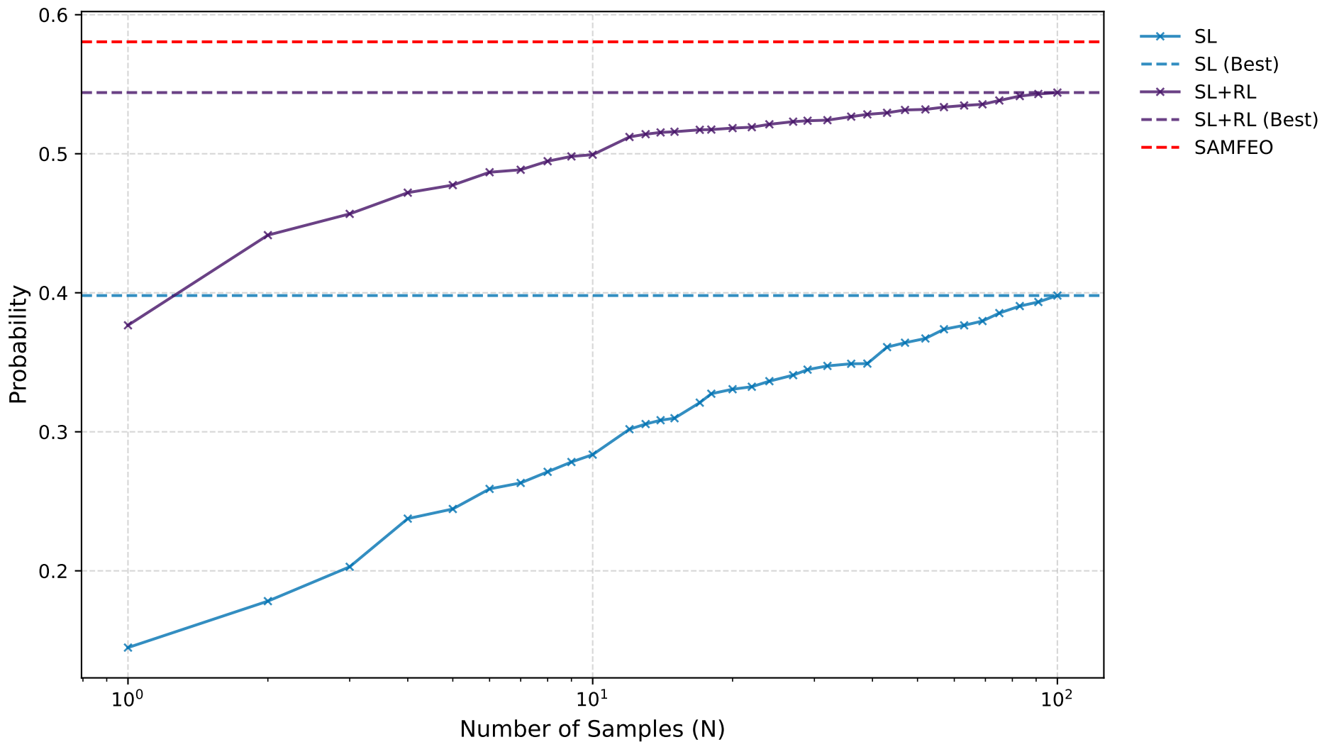
Best-of-N Probability
