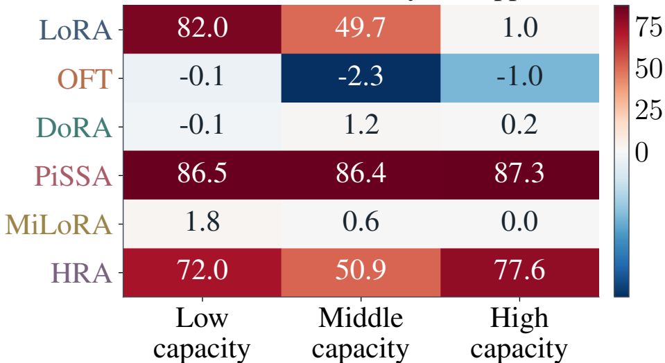
Qwen-7B: accuracy cost (pp)
