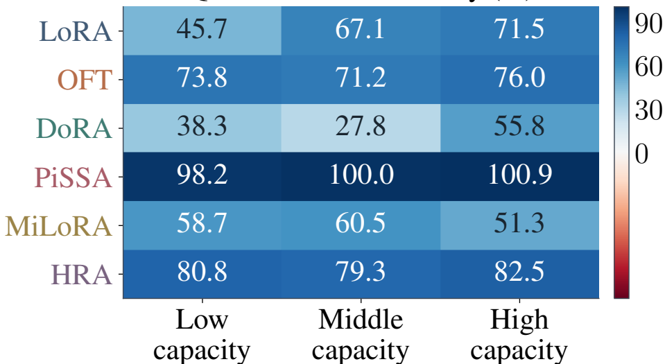
Qwen-7B: NLL recovery (%)
