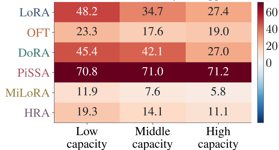
Llama-8B: accuracy cost (pp)
