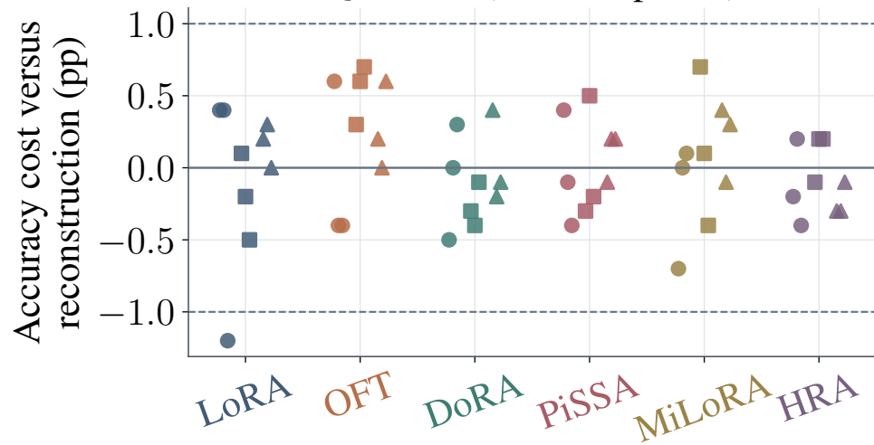
Qwen-7B (54 checkpoints)
