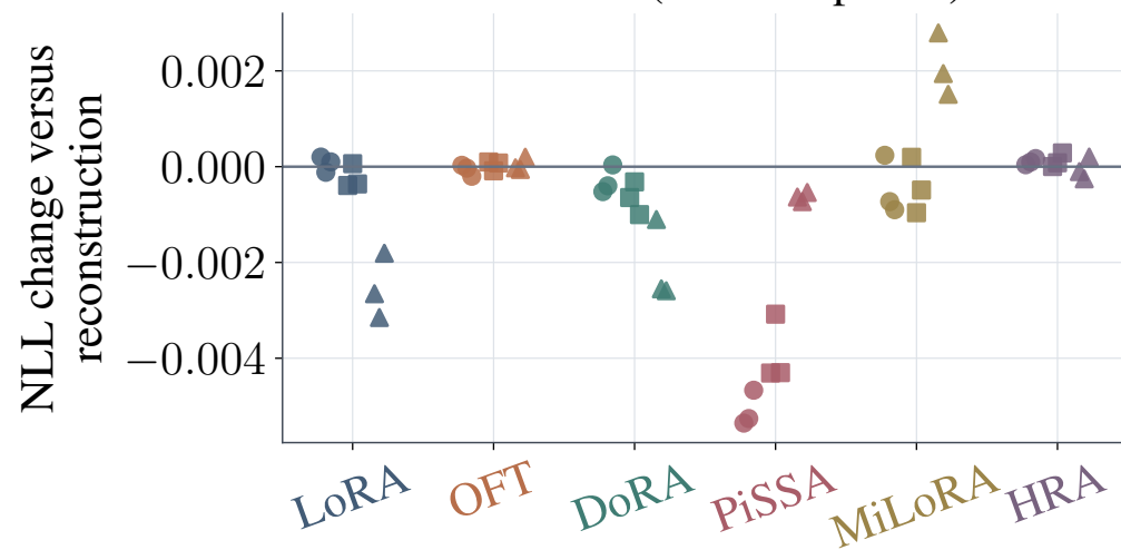
Llama-8B (54 checkpoints)
