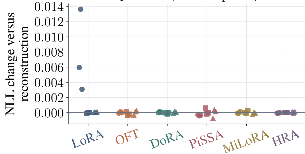
Qwen-7B (54 checkpoints)
