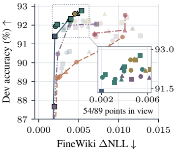
(a) Qwen2.5-7B
