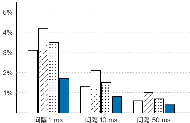
NVMe: fio randread-4k 吞吐降低
