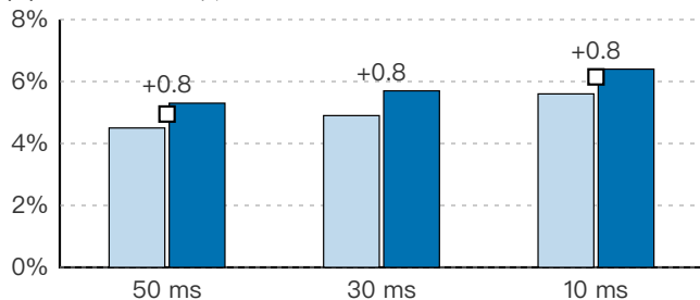
(c) virtio-scsi 读
