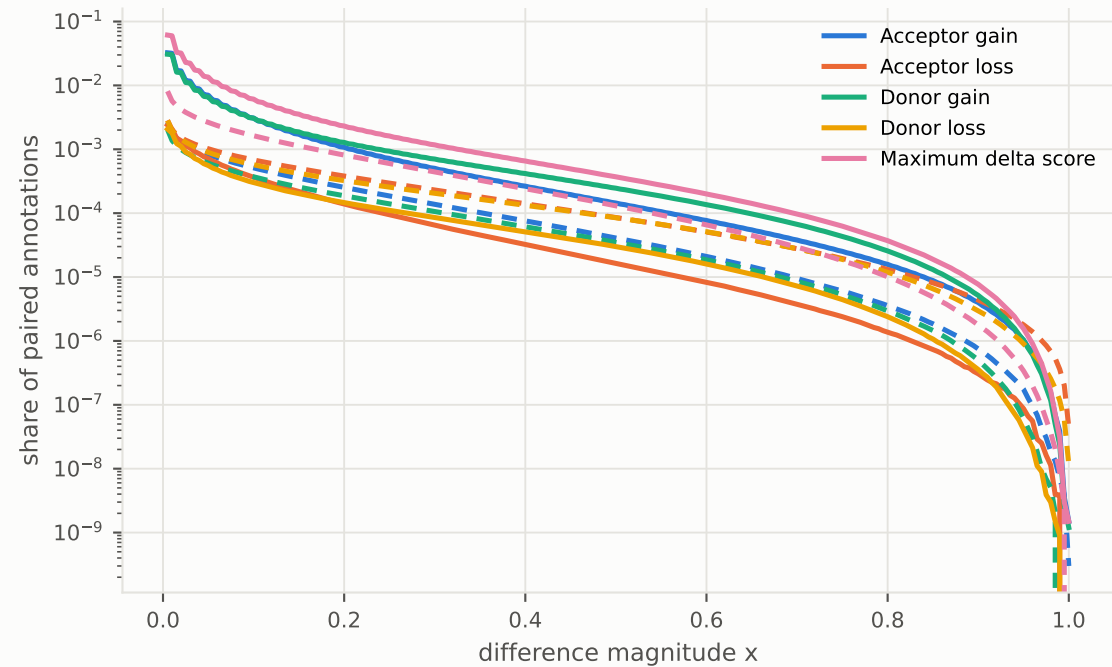
Solid: SpliceAI higher by \geq x · Dashed: OpenSpliceAI higher
