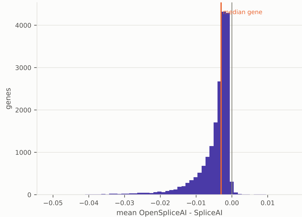
The divergence is a continuum, not a few outliers
