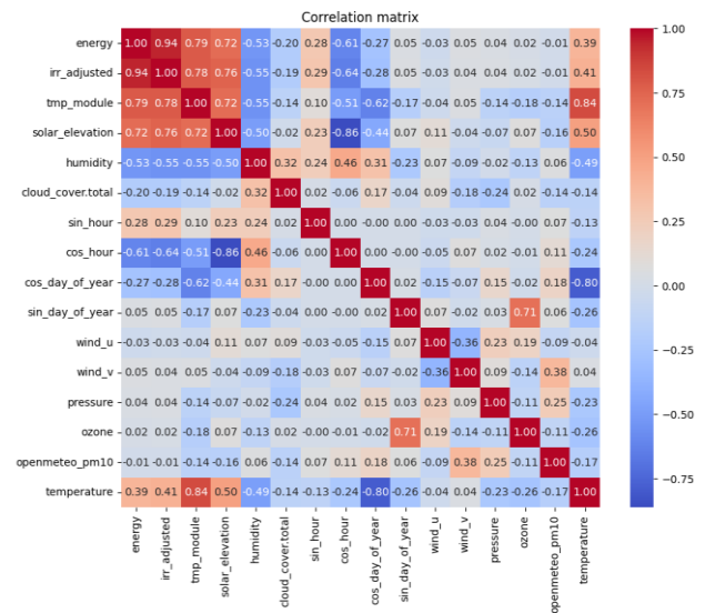
Fig. 2. Correlation matrix
