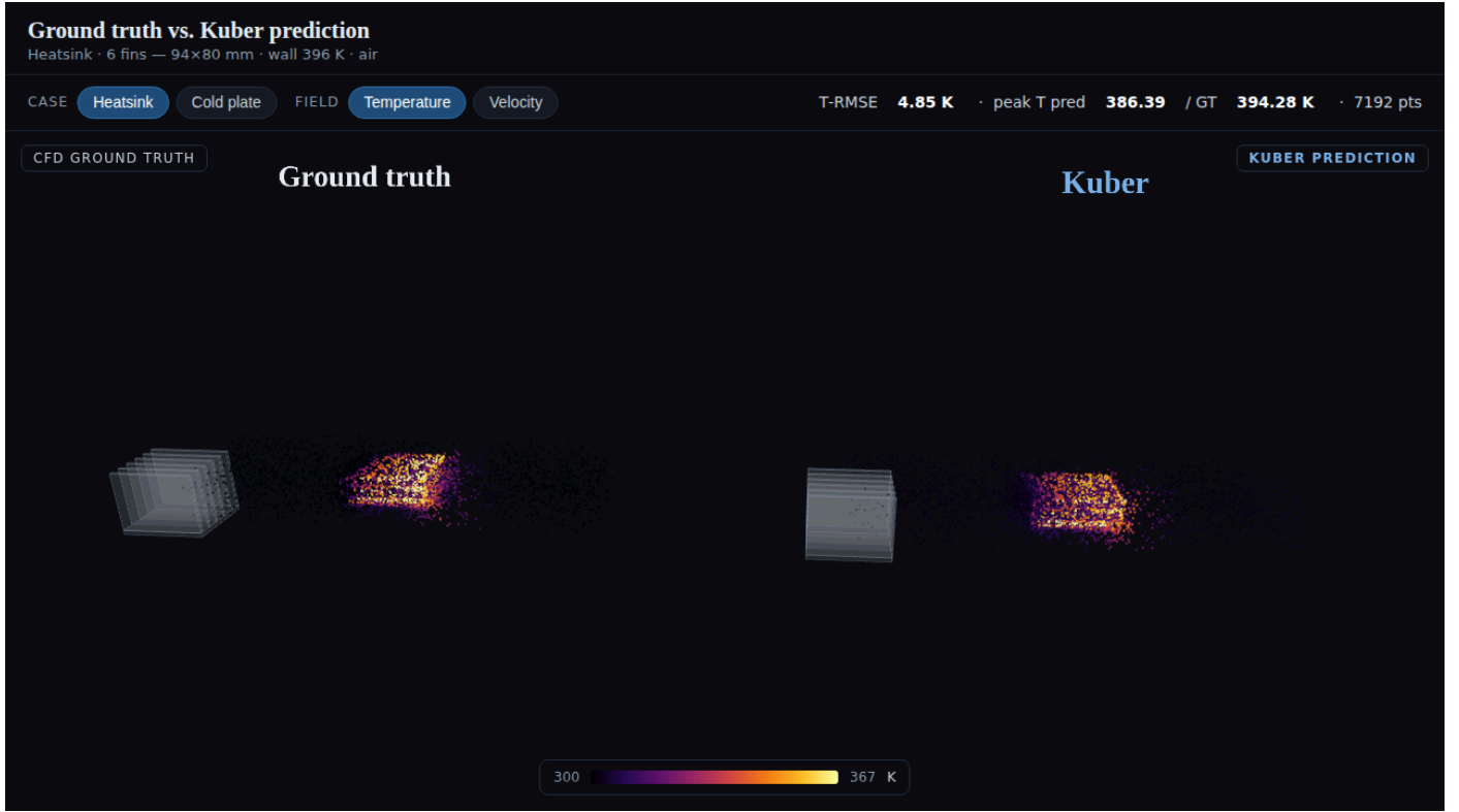
Fig. 2. Qualitative comparison from the interactive viewer: solid device geometry with the fluid temperature field, CFD ground truth (left) beside the surrogate prediction (right) for a heatsink; peak temperature and per-case T -RMSE are reported live.
