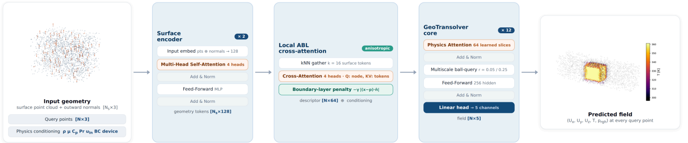
Fig. 2. KuberNet. Three inputs - the boundary surface point cloud with normals, the query points, and the physics conditioning - feed a neural spine (surface encoder → local anisotropic boundary-layer (ABL) cross-attention → concatenated per-node embedding → GeoTransolver physics-attention core) that predicts the five-channel field at every query node.
