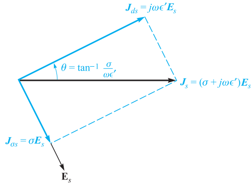
Figure 11.2 The time-phase relationship between J_{ds} , J_{os} , J_s , and E_s . The tangent of \theta is equal to \sigma/\omega\epsilon' , and 90^\circ - \theta is the common power-factor angle, or the angle by which J_s leads E_s .
