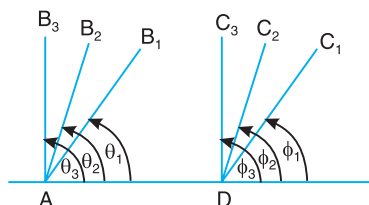
(b) Three positions of input and output link.
