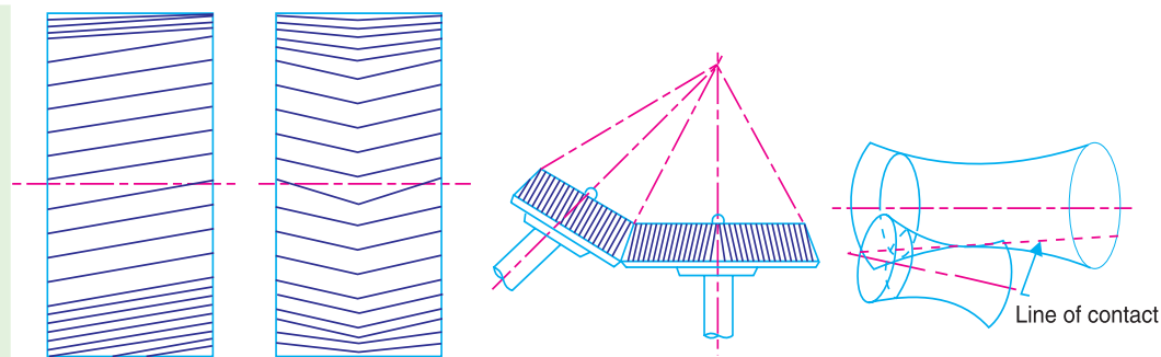
(a) Single helical gear. (b) Double helical gear.
