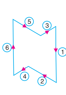
(g) Secondary couple polygon.
