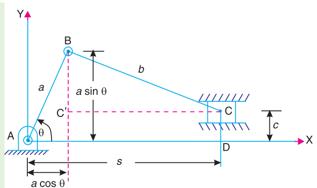
Fig. 25.20. Slider crank mechanism.
