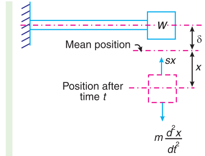
Fig. 23.3. Natural frequency of free transverse vibrations.
