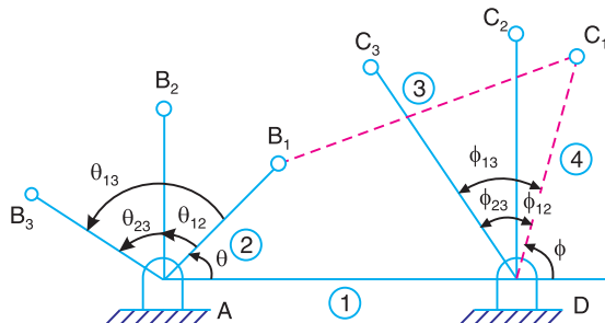
Fig. 25.7. Layout of four bar mechanism.
