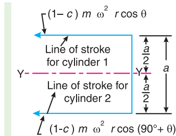
Fig. 22.5. Swaying couple.
