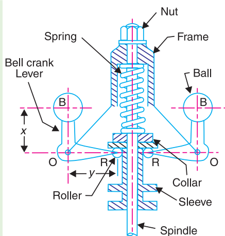
Fig. 18.18. Hartnell governor.
