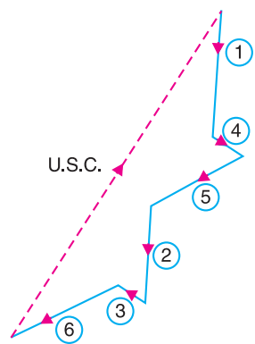
(g) Secondary couple polygon.
