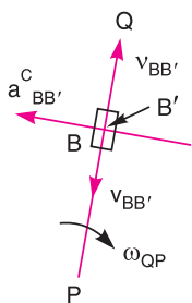
(c) Direction of coriolis component.
