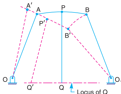
Fig. 9.10. Roberts mechanism
