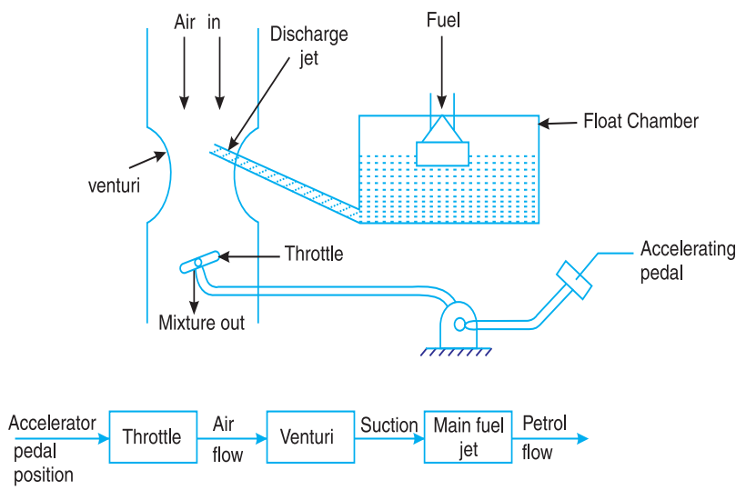
Fig. 26.1. Block diagram of a single carburettor.
