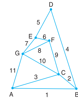
(a) Looked chain having binary, ternary and quaternary joints.
