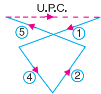
(e) Primary couple polygon.
